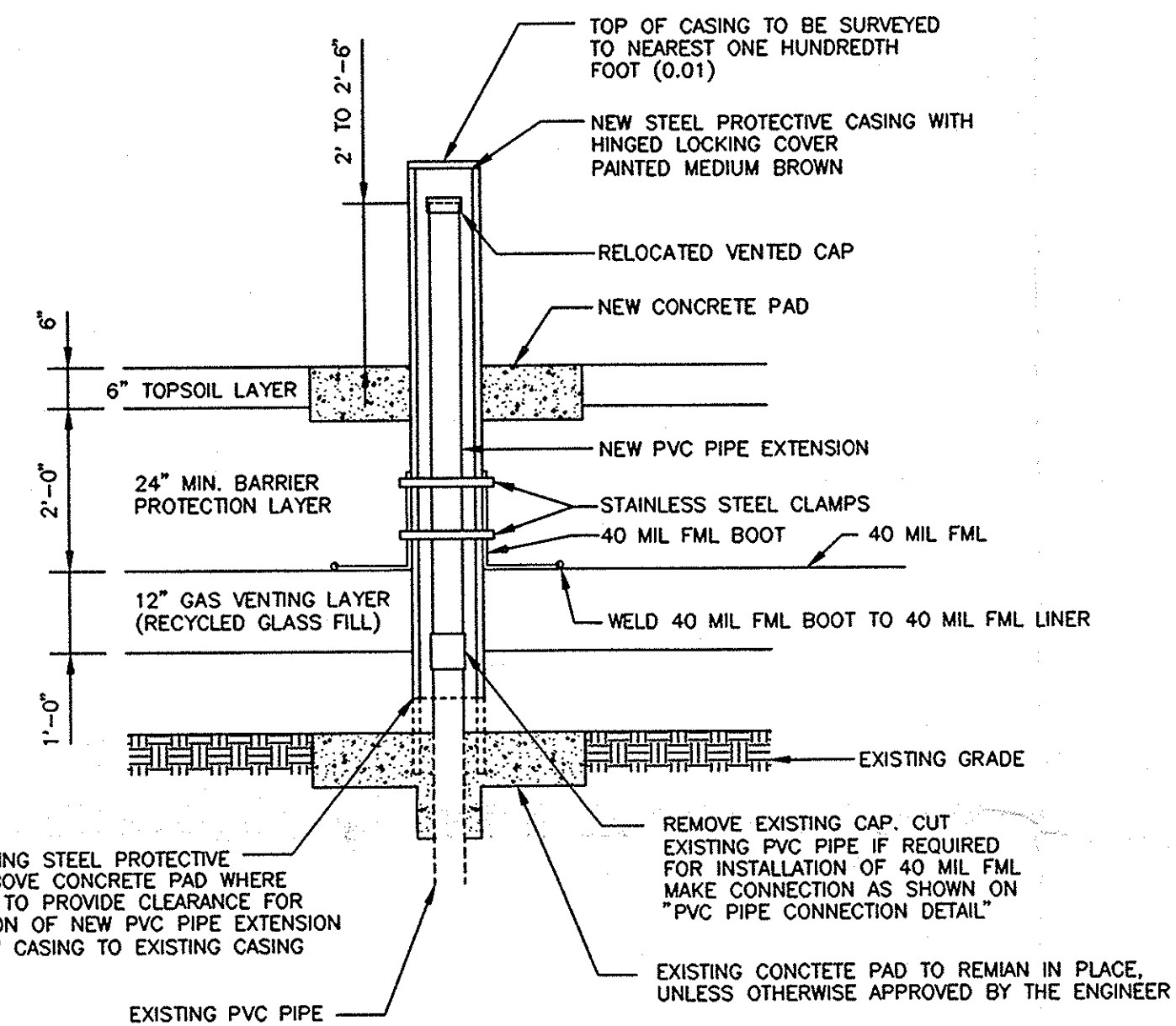
MONITORING WELL EXTENSION DETAIL
