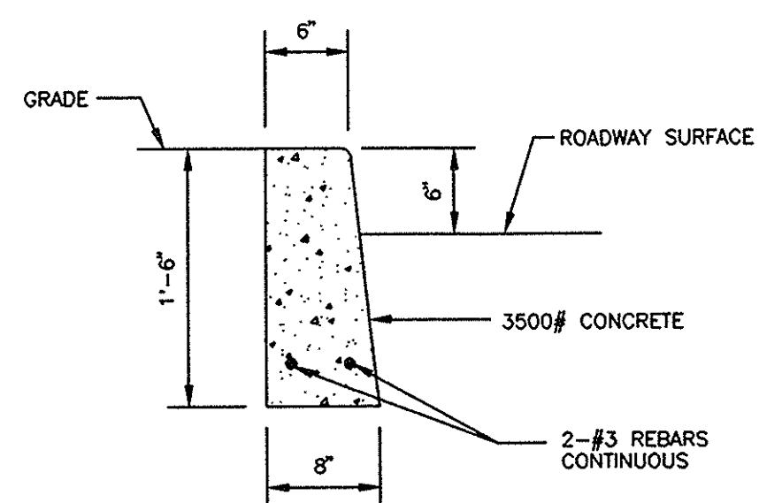
CONCRETE CURB DETAIL
