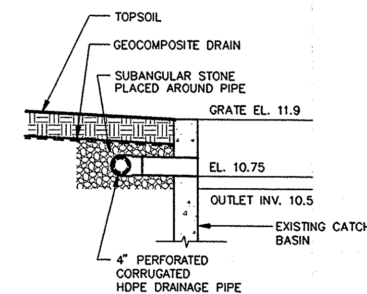
FRENCH DRAIN FIELD INLET CROSS-SECTION
