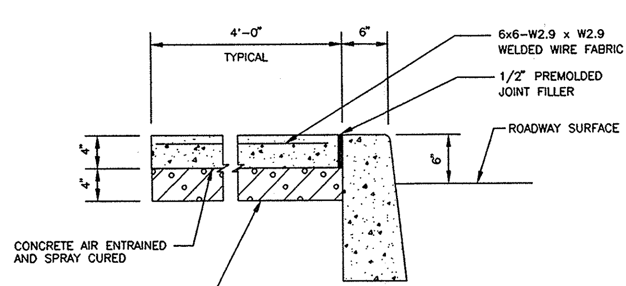
CONCRETE WALK DETAIL
