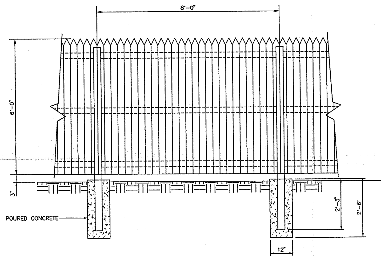
TYPICAL STOCKADE FENCE DETAIL
