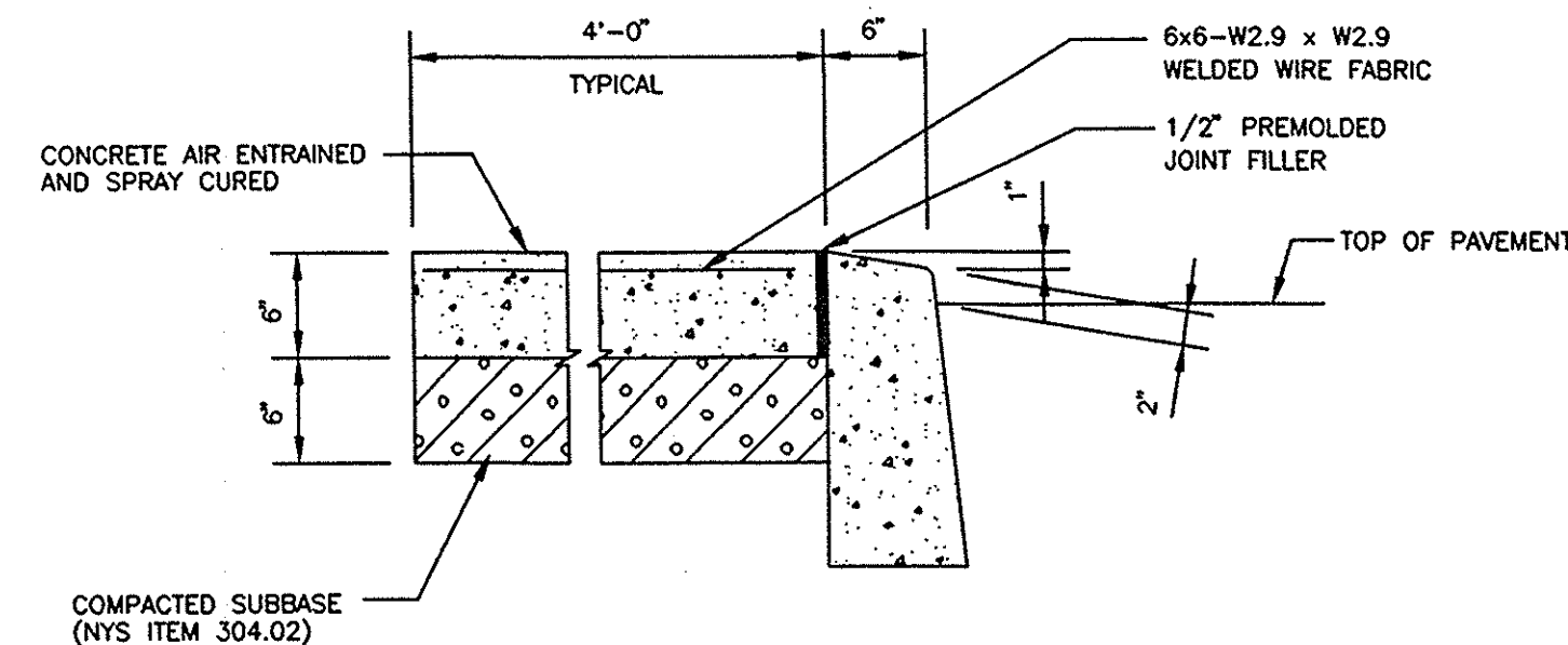
CONCRETE DRIVEWAY APRON DETAIL
