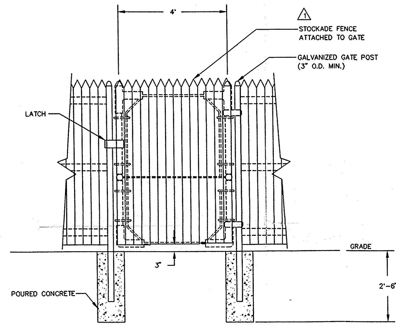
TYPICAL PEDESTRIAN GATE DETAIL
