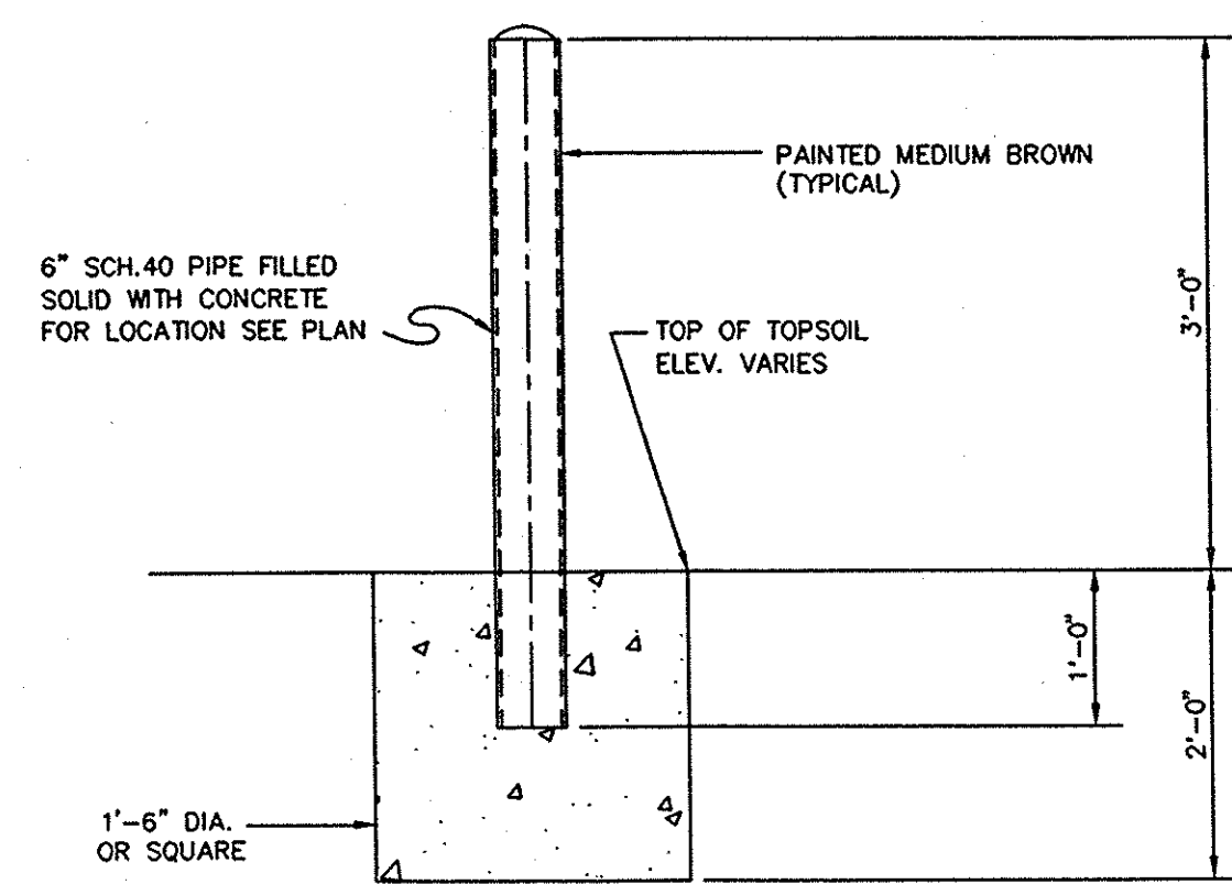
BOLLARD DETAIL
