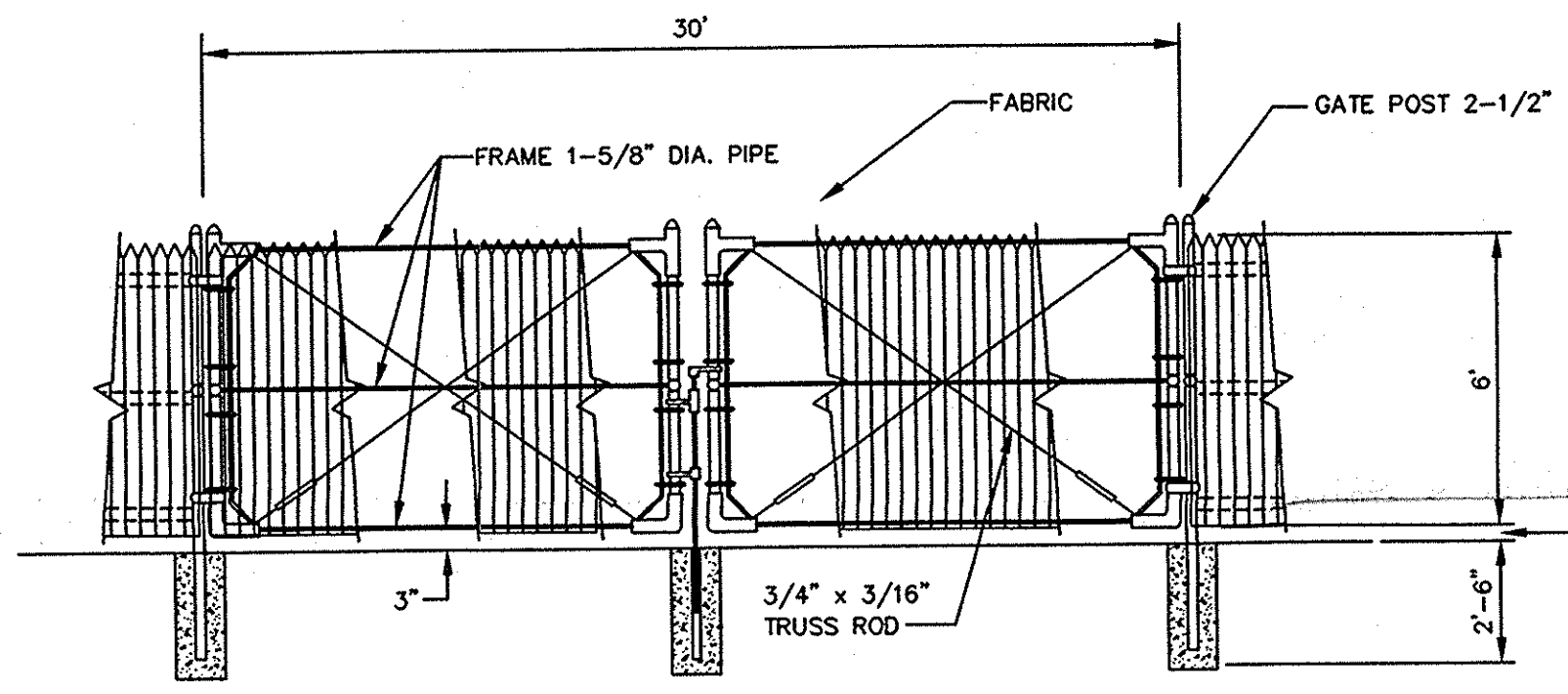
TYPICAL DOUBLE GATE N.T.S.
