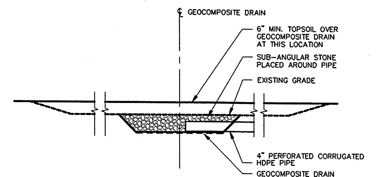
DRAIN OUTLET AT STA.0+65 CROSS-SECTION
