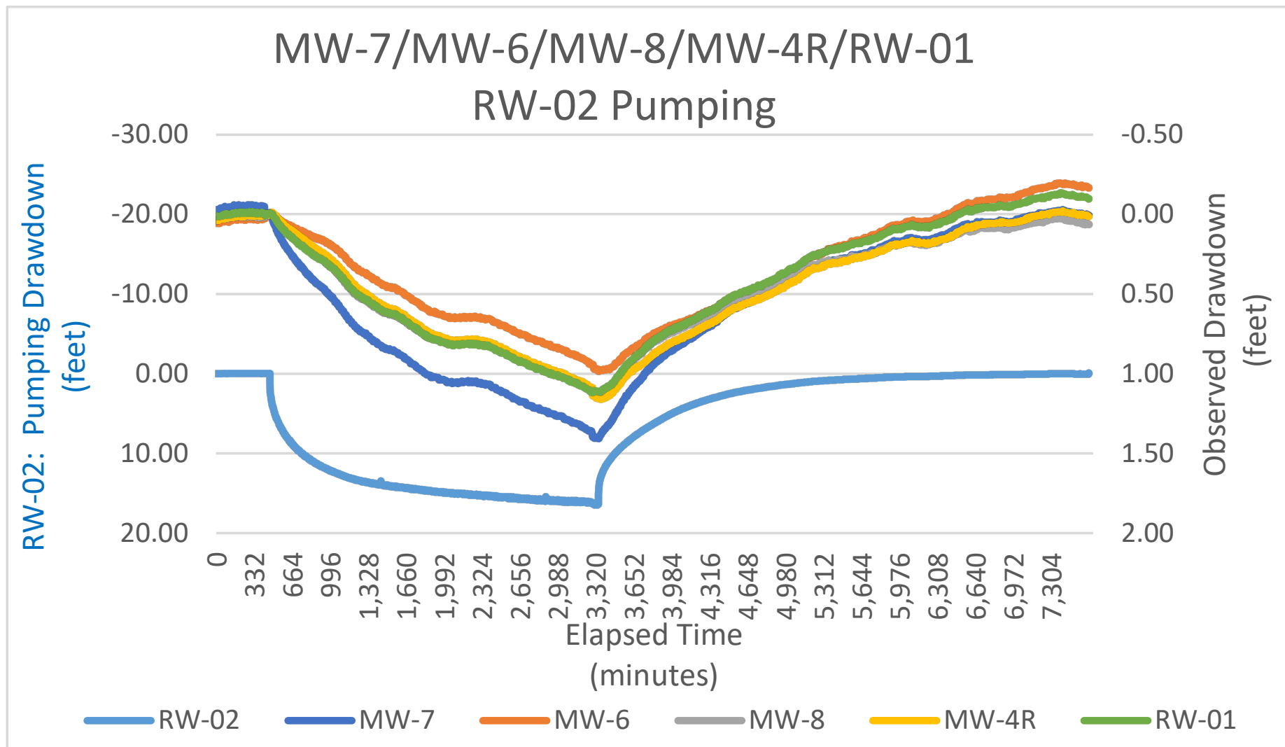
Chart 6 Observed Drawdown During GWET System Evaluation: Well RW-02 Test September 20, 2023 through September 22, 2023 Former Ward Products 61 Edson Street, Amsterdam, New York NYSDEC Site No. 429004
