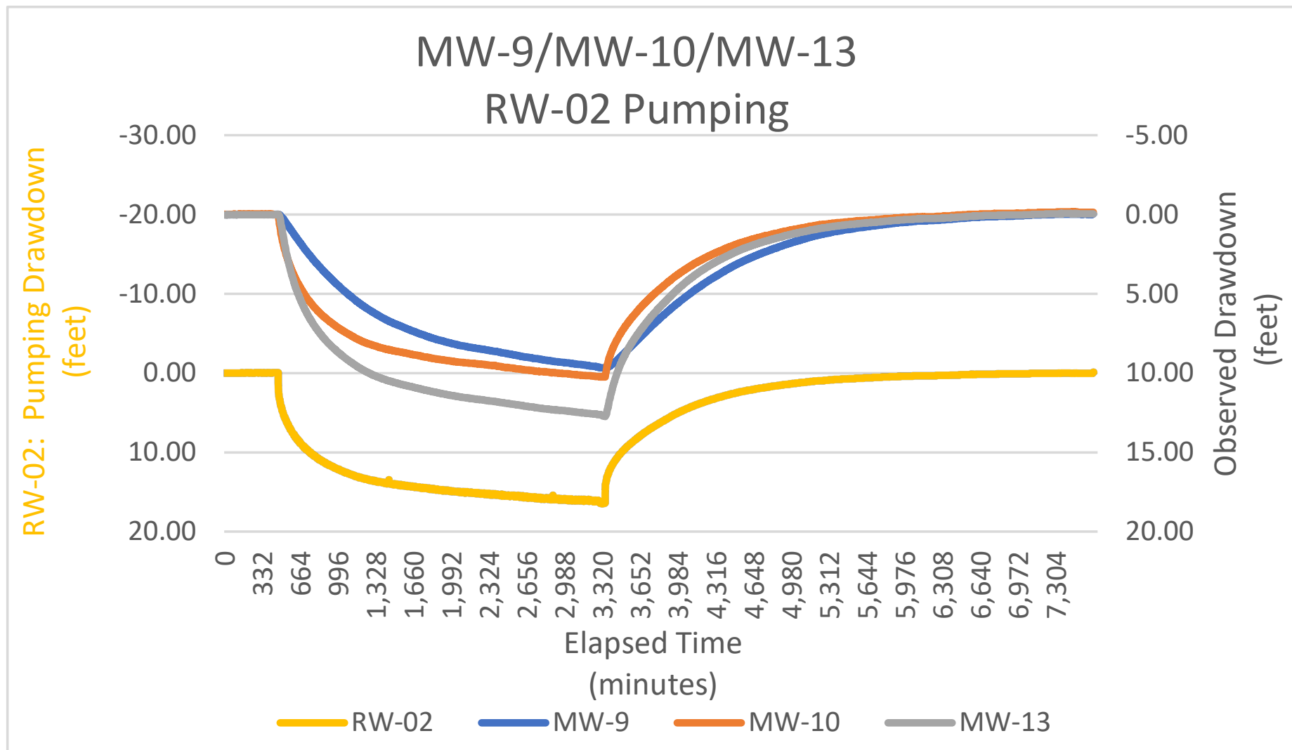
Chart 7 Observed Drawdown During GWET System Evaluation: Well RW-02 Test September 20, 2023 through September 22, 2023 Former Ward Products 61 Edson Street, Amsterdam, New York NYSDEC Site No. 429004
