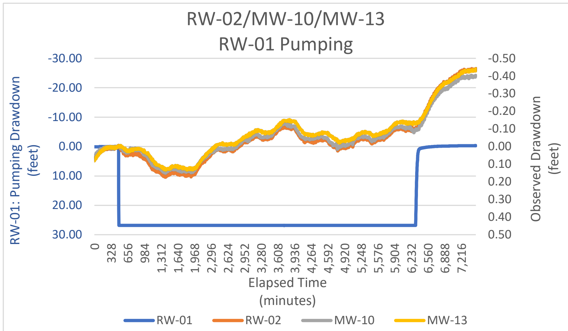
Chart 3 Observed Drawdown During GWET System Evaluation: Well RW-01 Test September 14, 2023 through September 18, 2023 Former Ward Products 61 Edson Street, Amsterdam, New York NYSDEC Site No. 429004
