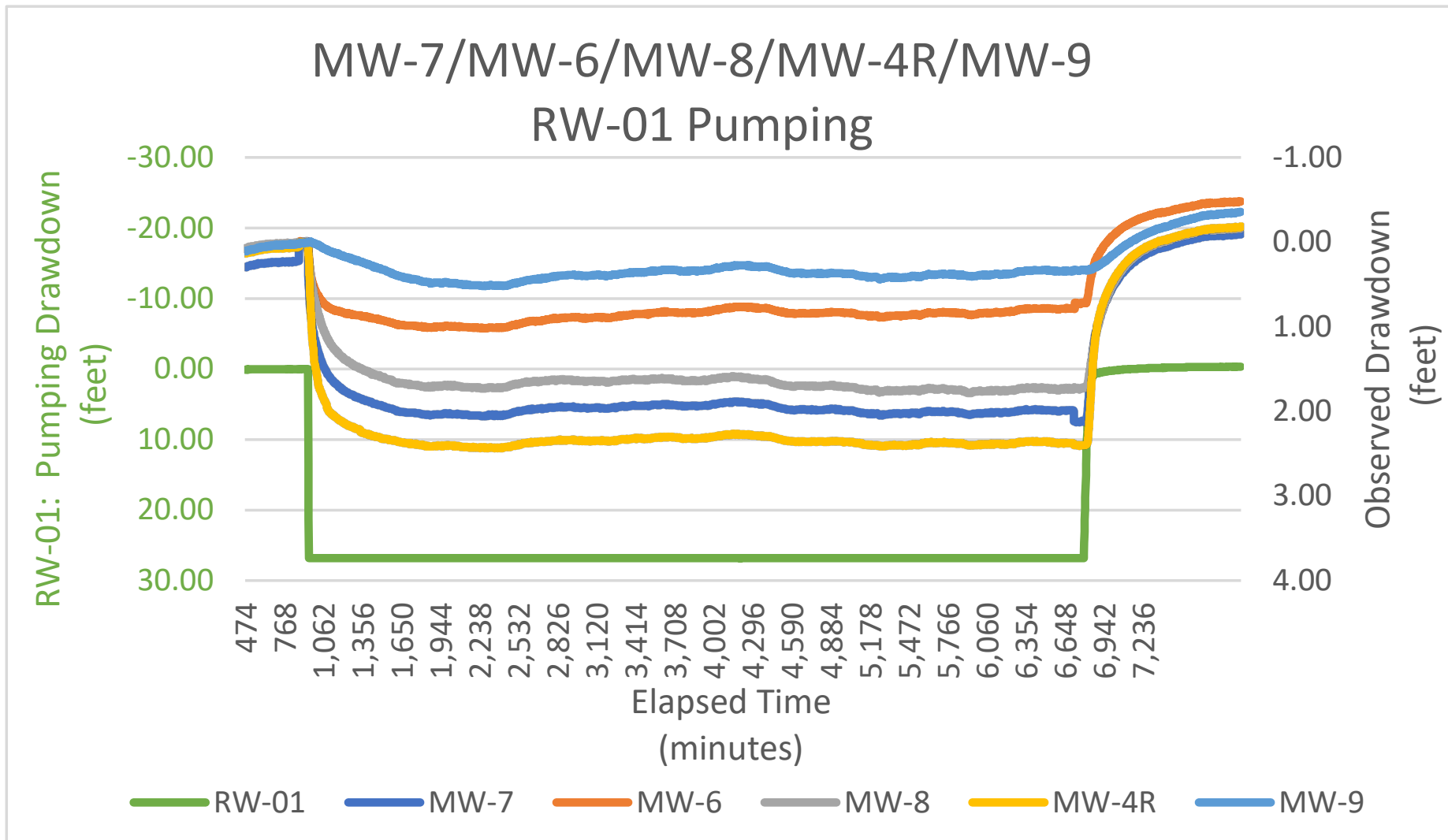
Chart 2 Observed Drawdown During GWET System Evaluation: Well RW-01 Test September 14, 2023 through September 18, 2023 Former Ward Products 61 Edson Street, Amsterdam, New York NYSDEC Site No. 429004
