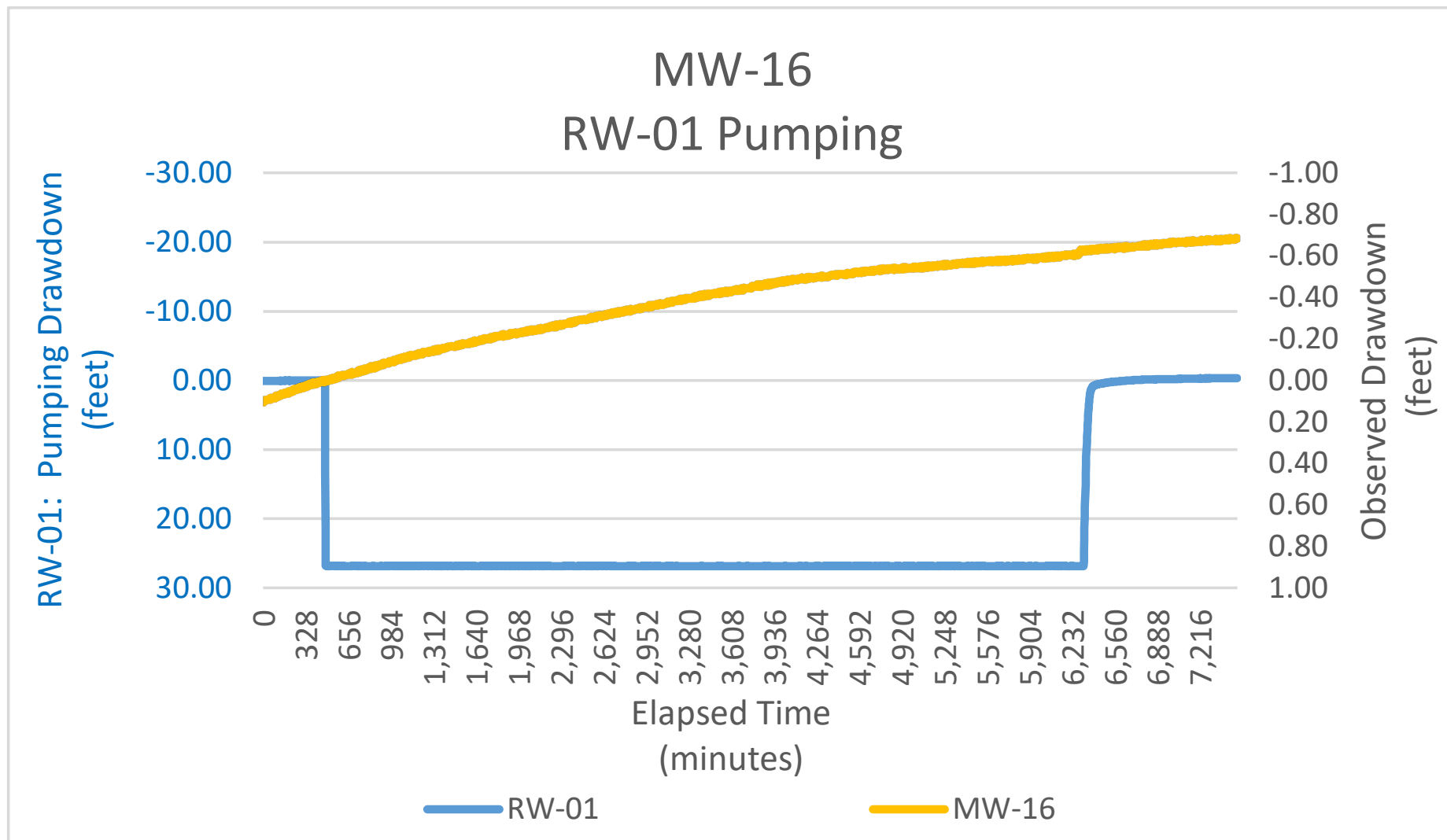
Chart 5 Observed Drawdown During GWET System Evaluation: Well RW-01 Test September 14, 2023 through September 18, 2023 Former Ward Products 61 Edson Street, Amsterdam, New York NYSDEC Site No. 429004
