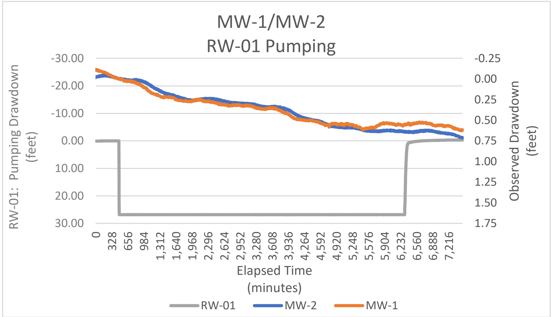
Chart 4 Observed Drawdown During GWET System Evaluation: Well RW-01 Test September 14, 2023 through September 18, 2023 Former Ward Products 61 Edson Street, Amsterdam, New York NYSDEC Site No. 429004
