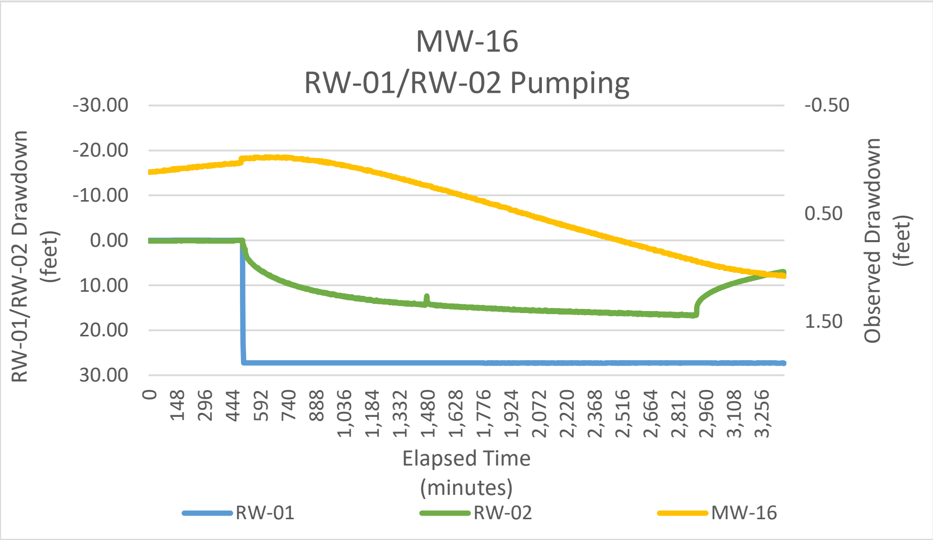
Chart 13 Observed Drawdown During GWET System Evaluation: Combined (RW-01/RW-02) Test September 25, 2023 through September 27, 2023 Former Ward Products 61 Edson Street, Amsterdam, New York NYSDEC Site No. 429004
