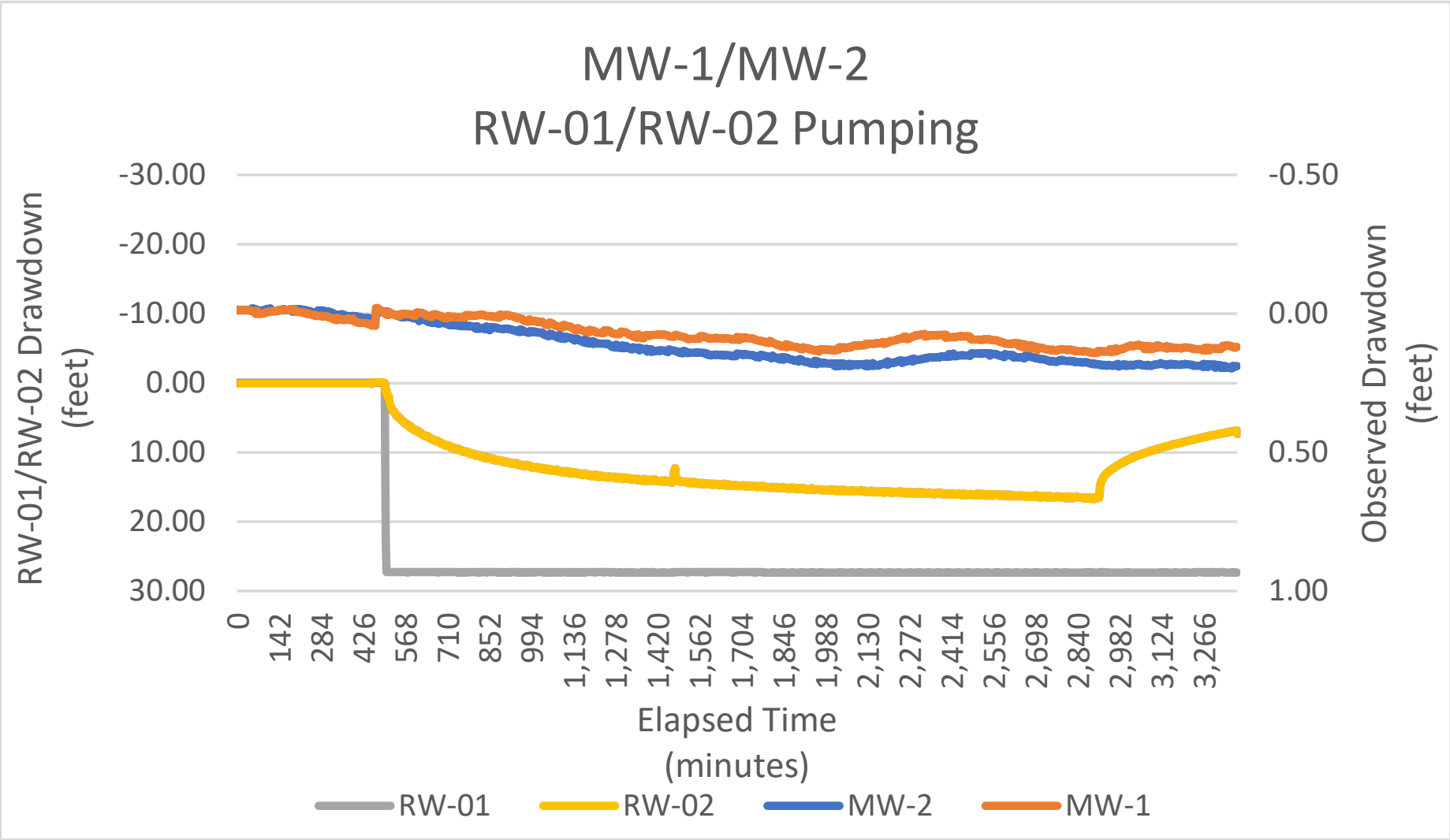
Chart 12 Observed Drawdown During GWET System Evaluation: Combined (RW-01/RW-02) Test September 25, 2023 through September 27, 2023 Former Ward Products 61 Edson Street, Amsterdam, New York NYSDEC Site No. 429004
