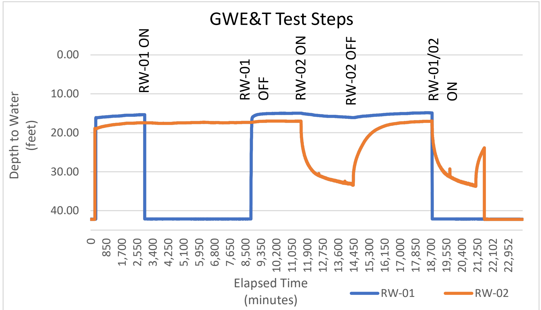
Chart 1 Data Collected During GWET System Evaluation September 14, 2023 through September 27, 2023 Former Ward Products 61 Edson Street, Amsterdam, New York NYSDEC Site No. 429004
