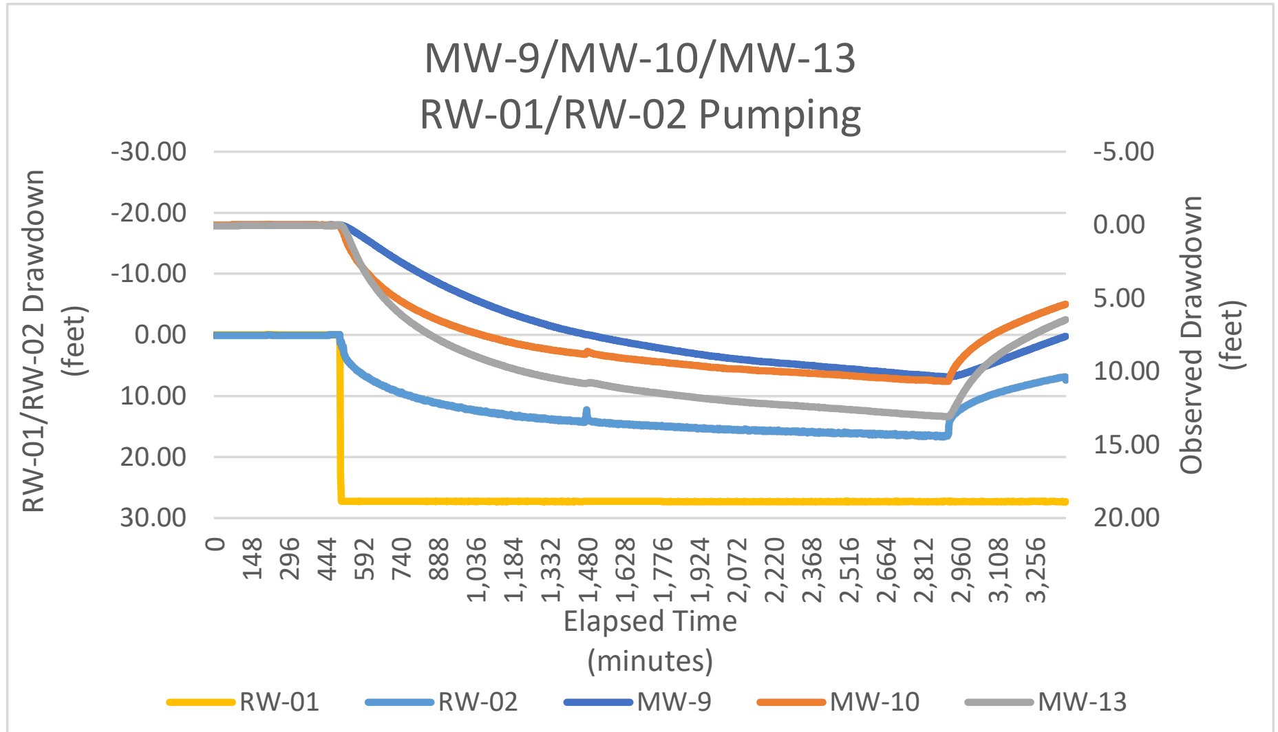
Chart 11 Observed Drawdown During GWET System Evaluation: Combined (RW-01/RW-02) Test September 25, 2023 through September 27, 2023 Former Ward Products 61 Edson Street, Amsterdam, New York NYSDEC Site No. 429004
