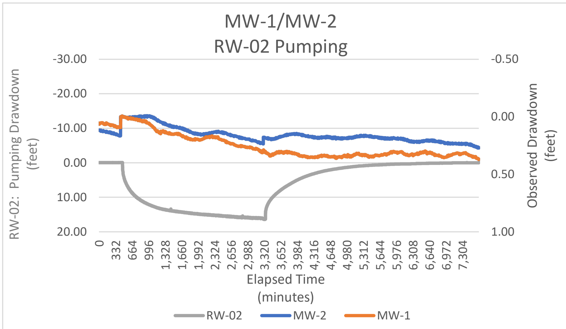
Chart 8 Observed Drawdown During GWET System Evaluation: Well RW-02 Test September 20, 2023 through September 22, 2023 Former Ward Products 61 Edson Street, Amsterdam, New York NYSDEC Site No. 429004
