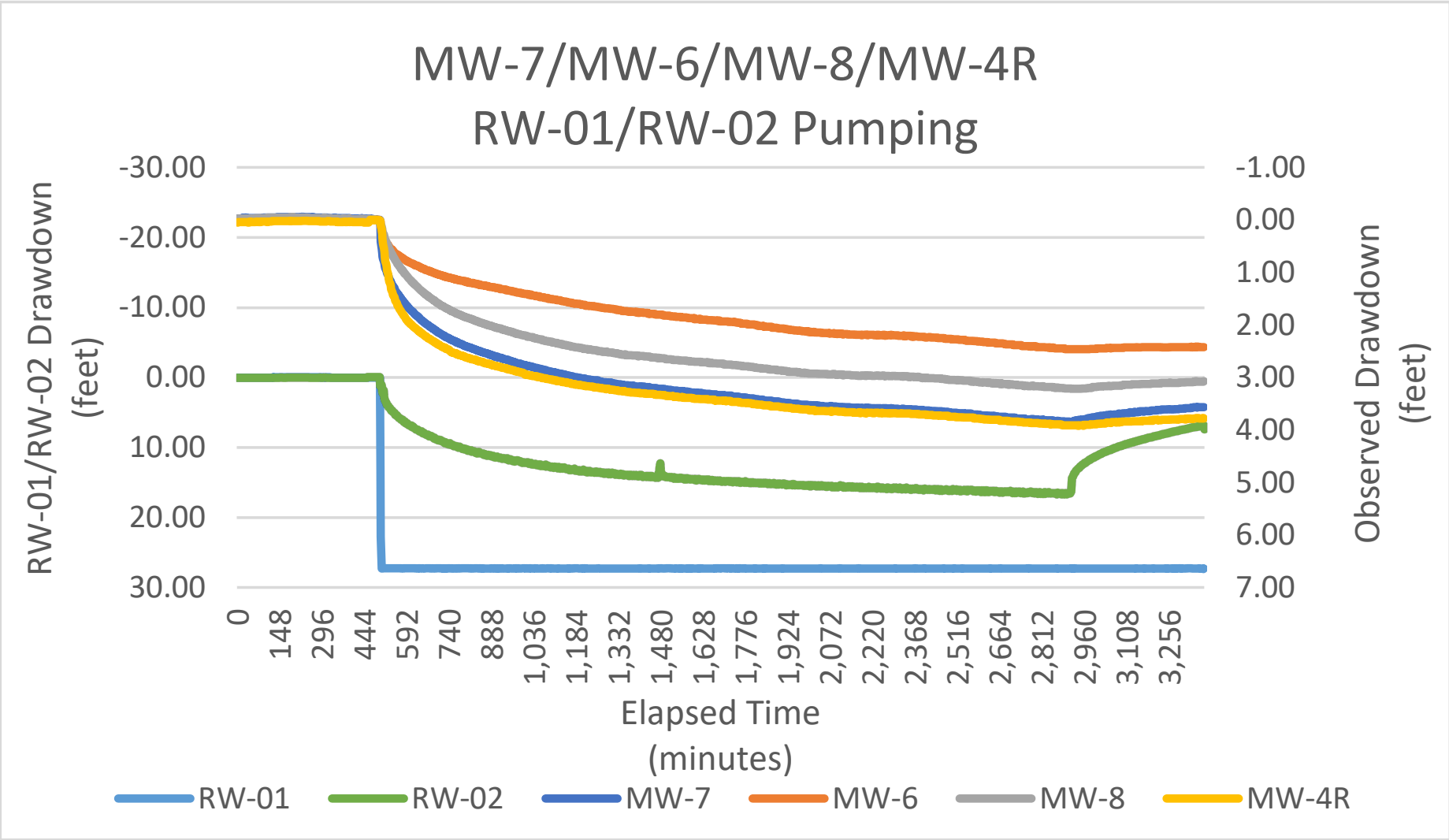
Chart 10 Observed Drawdown During GWET System Evaluation: Combined (RW-01/RW-02) Test September 25, 2023 through September 27, 2023 Former Ward Products 61 Edson Street, Amsterdam, New York NYSDEC Site No. 429004
