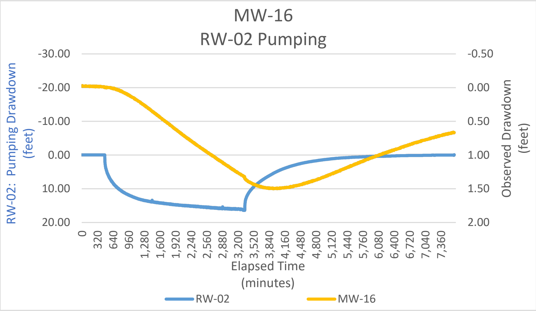
Chart 9 Observed Drawdown During GWET System Evaluation: Well RW-02 Test September 20, 2023 through September 22, 2023 Former Ward Products 61 Edson Street, Amsterdam, New York NYSDEC Site No. 429004
