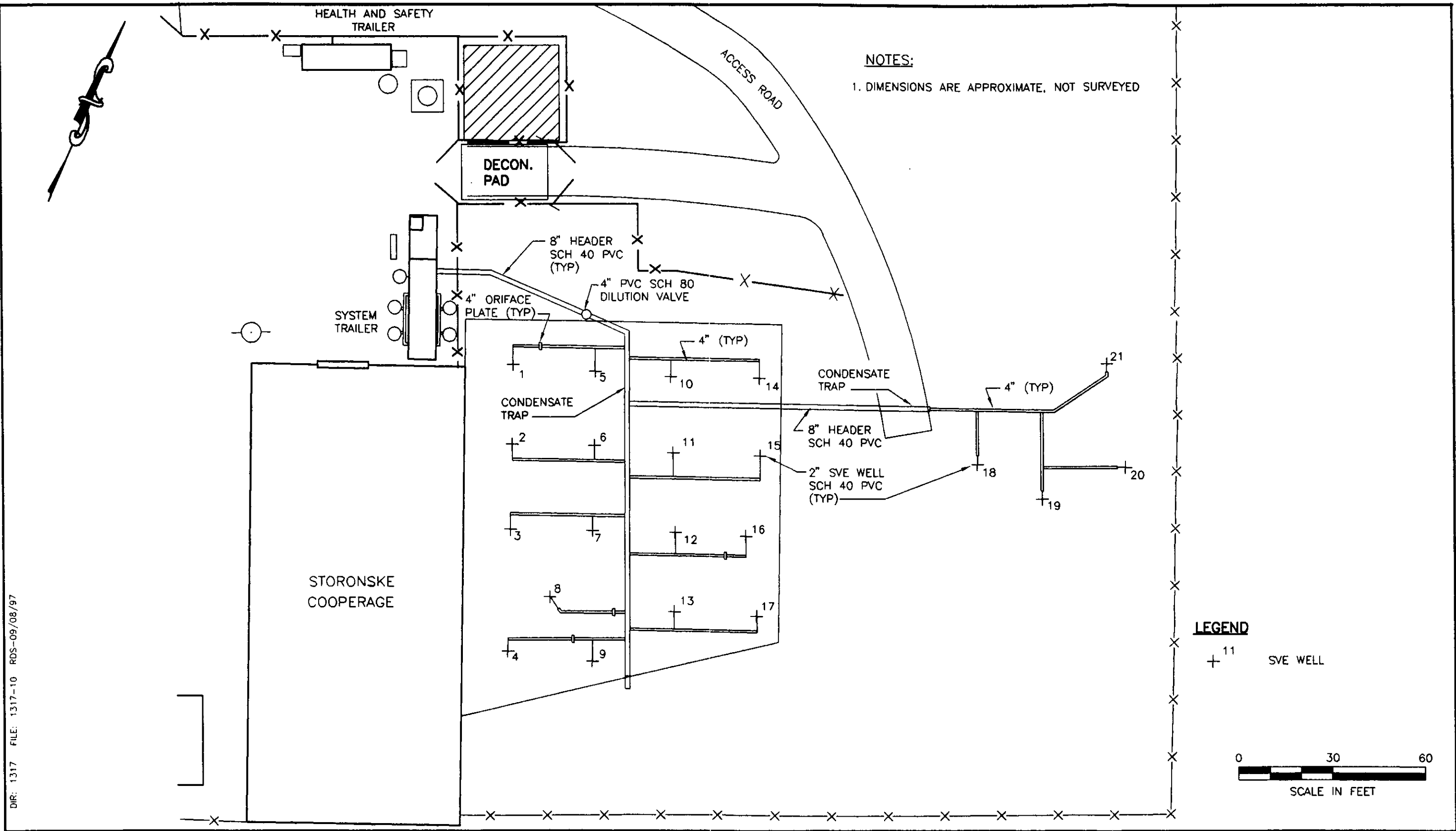
STORONSKE COOPERAGE SITE SVE SYSTEM LAYOUT
