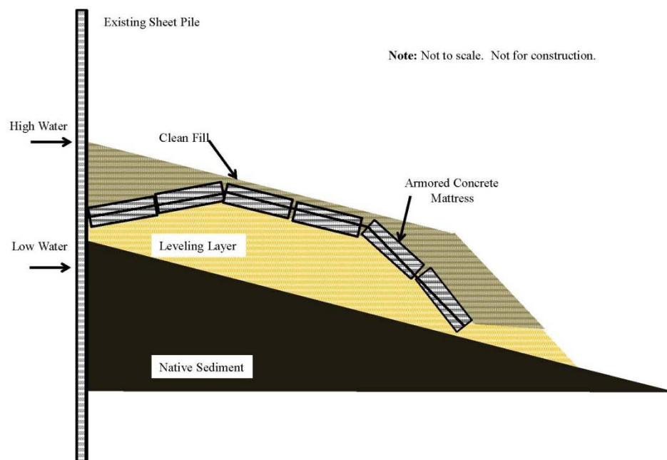
Figure 4. Conceptual Cross-Section: Fringe Wetland
