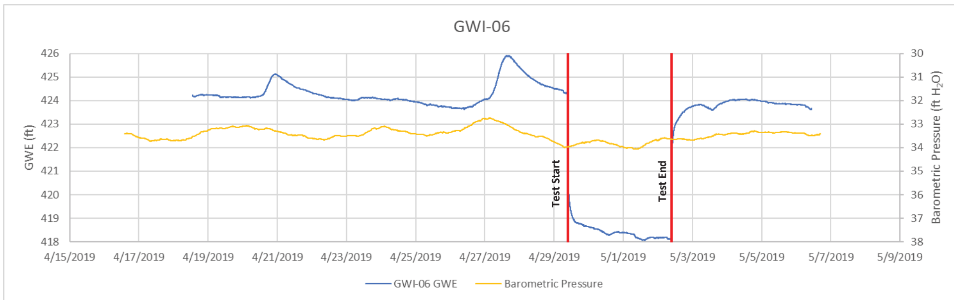
Figure A8-3: April 2019 Pumping Test: Barometric Pressure & Groundwater Elevation Hoosick Falls, New York
