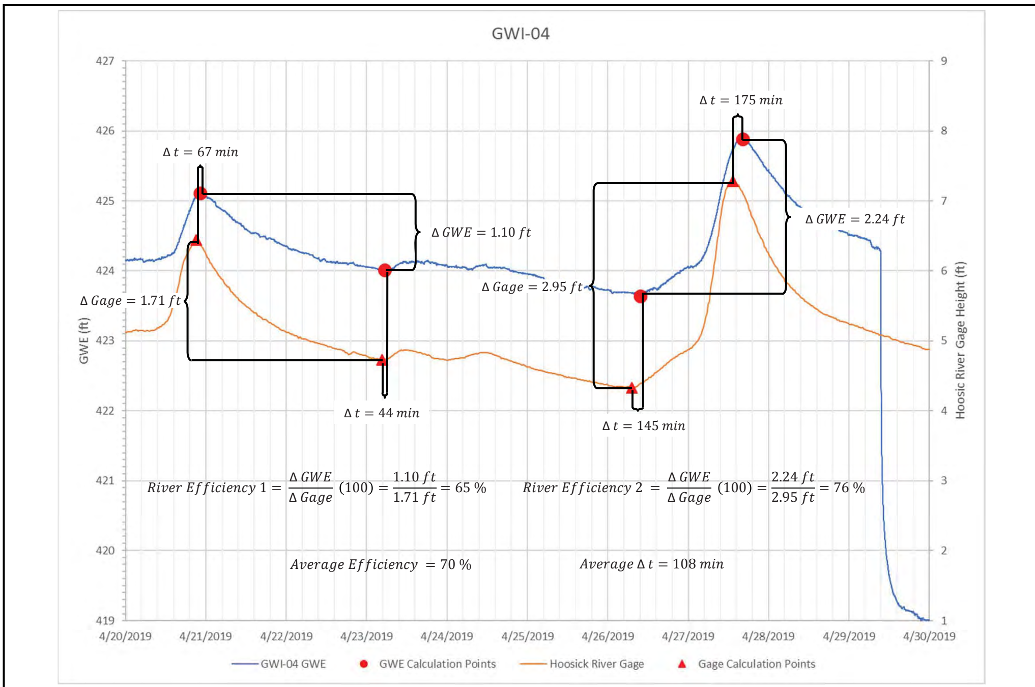
Figure A10-4: April 2019 Pump Test – River Efficiency Calculation of GWI-04 Hoosick Falls, New York
