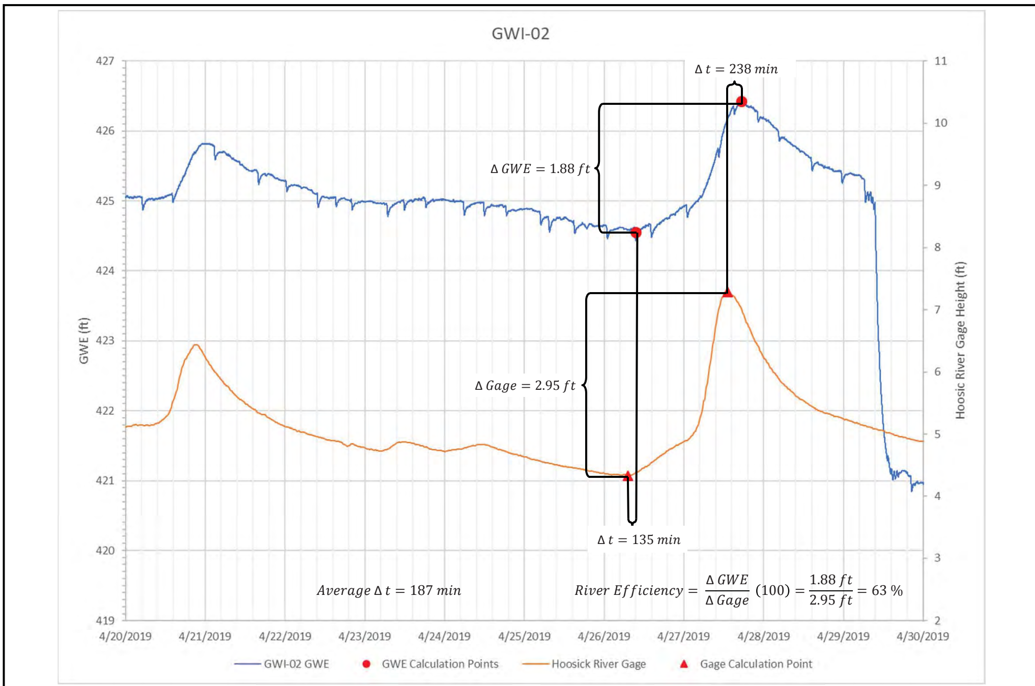
Figure A10-2: April 2019 Pump Test – River Efficiency Calculation of GWI-02
