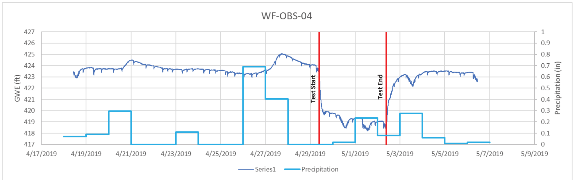
Figure A11-5: April 2019 Pumping Test: Precipitation & Groundwater Elevation Hoosick Falls, New York
