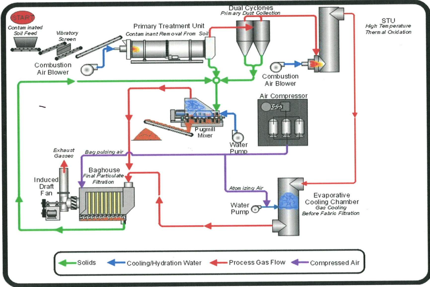
ESMI of New York Direct-fired Parallel Flow LTTD System
