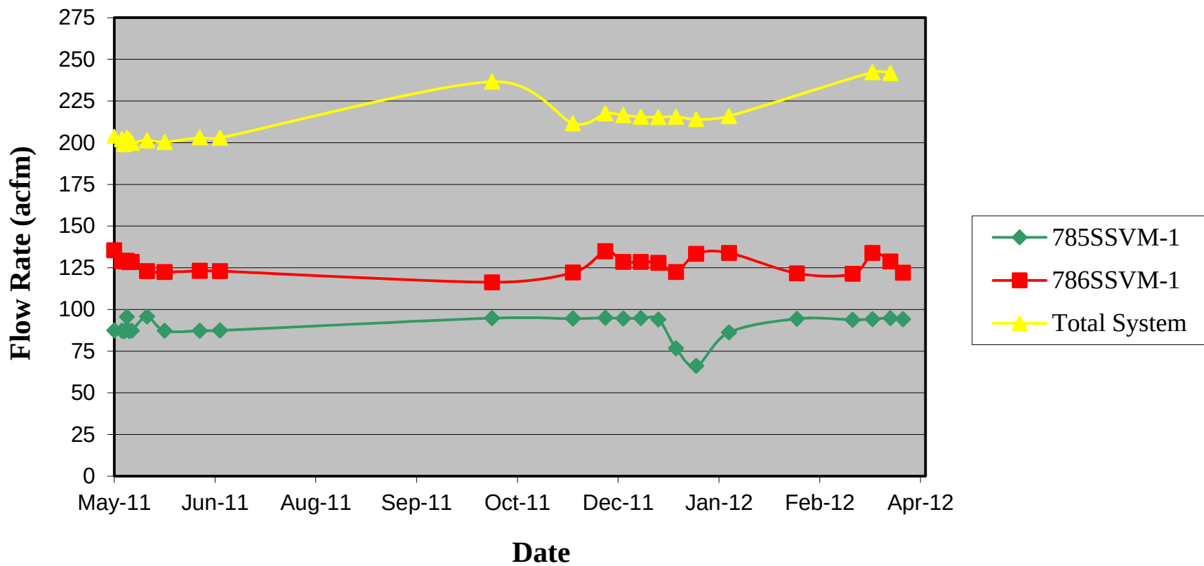
Figure 3-3 785SSVM-1 and 786SSVM-1 Long Term Operation Flow Rate (May 2011 through March 2012)
