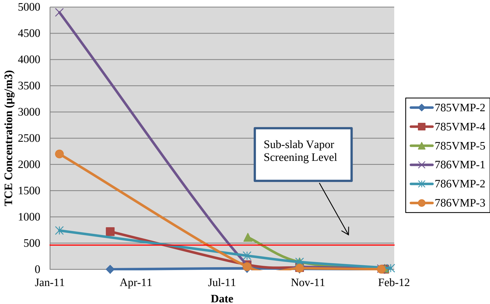
Figure 3-7 Trend Chart Sub-Slab Results Building 785 and 786 (February 2011 through March 2012)
