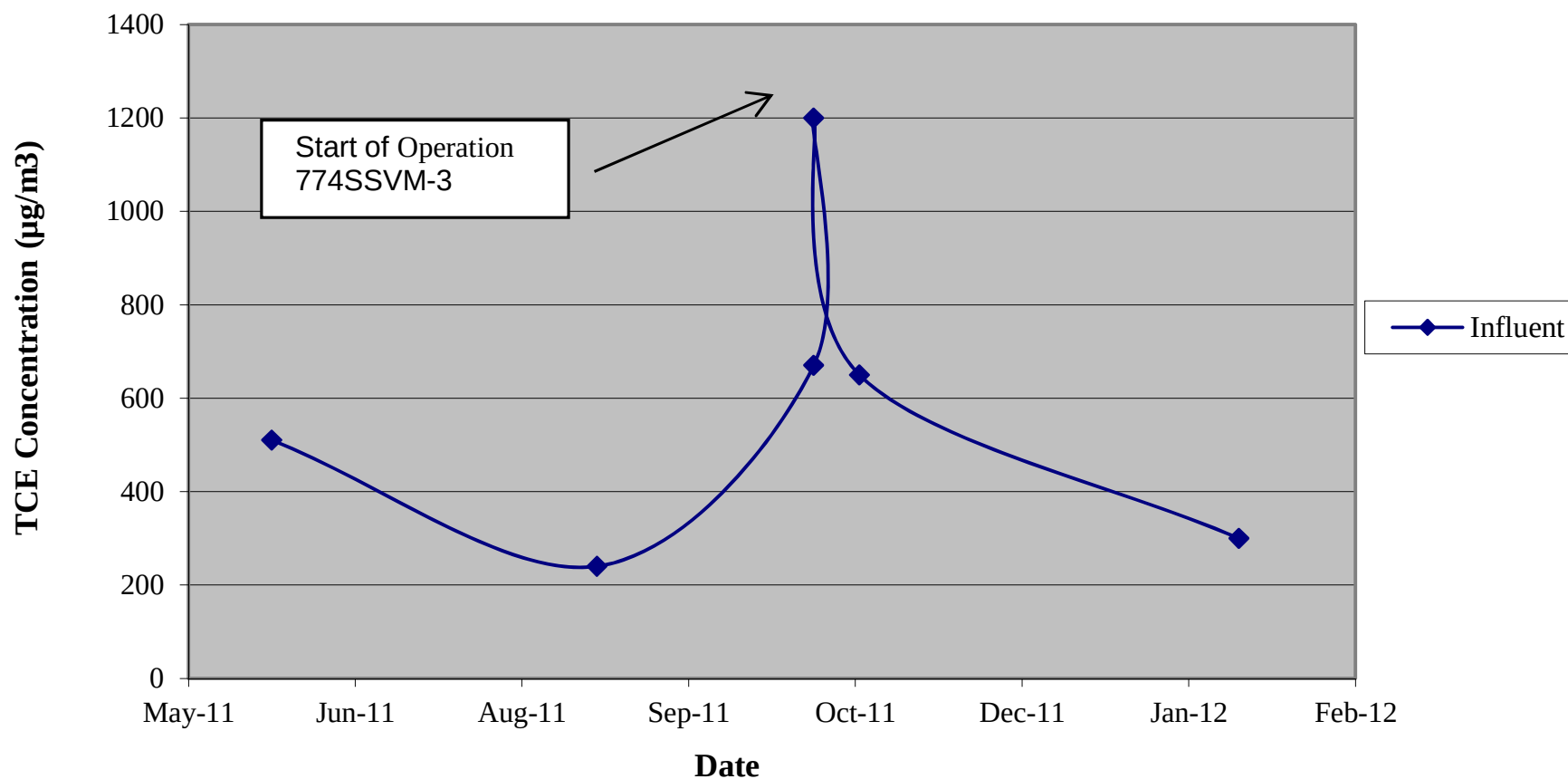
Figure 3-6 Trend Chart Influent Results Building 774 and 776 (June 2011 through March 2012)
