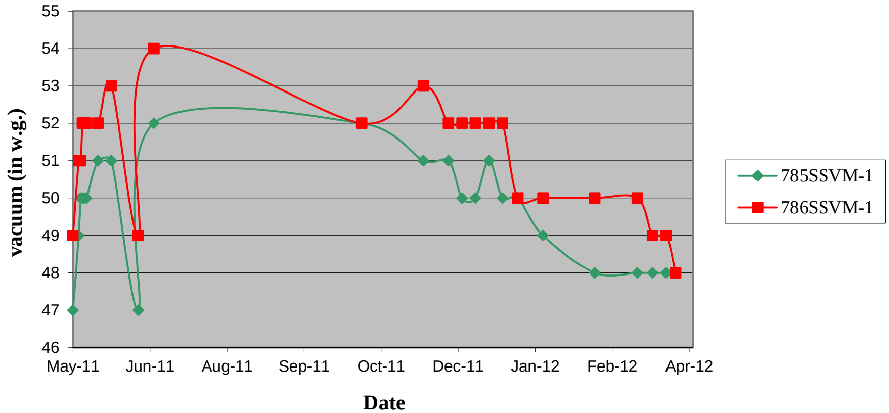
Figure 3-4 785SSVM-1 and 786SSVM-1 Long Term Operation Vacuum (May 2011 through March 2012)
