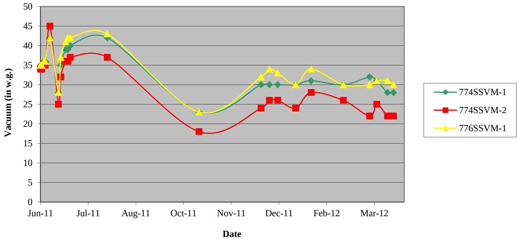
Figure 3-2 774SSVM-1, -2 and 776SSVM-1 Long Term Operation Vacuum (June 2011 through March 2012)
