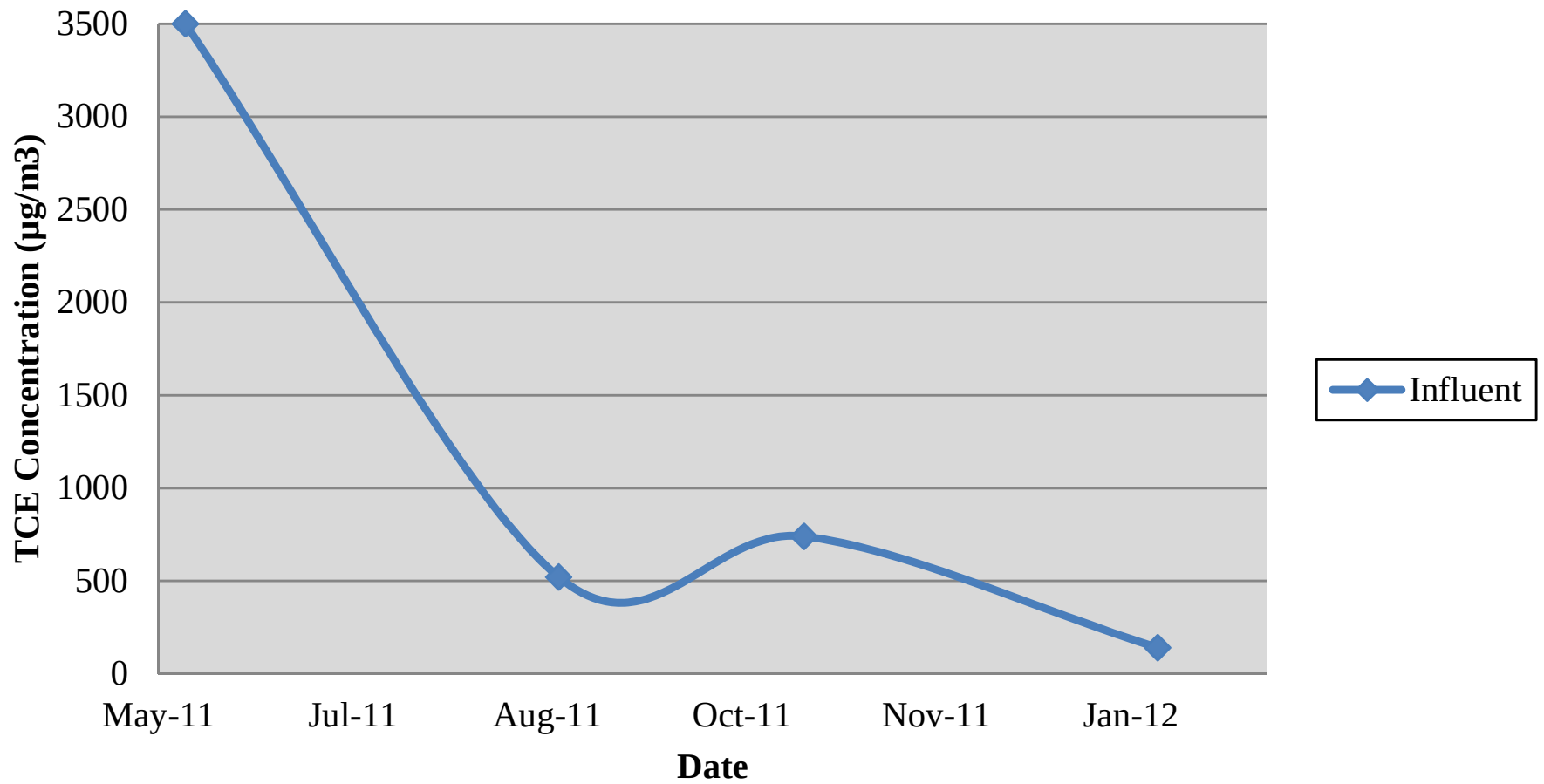
Figure 3-8 Trend Chart Influent Results Building 785 and 786 (May 2011 through March 2012)
