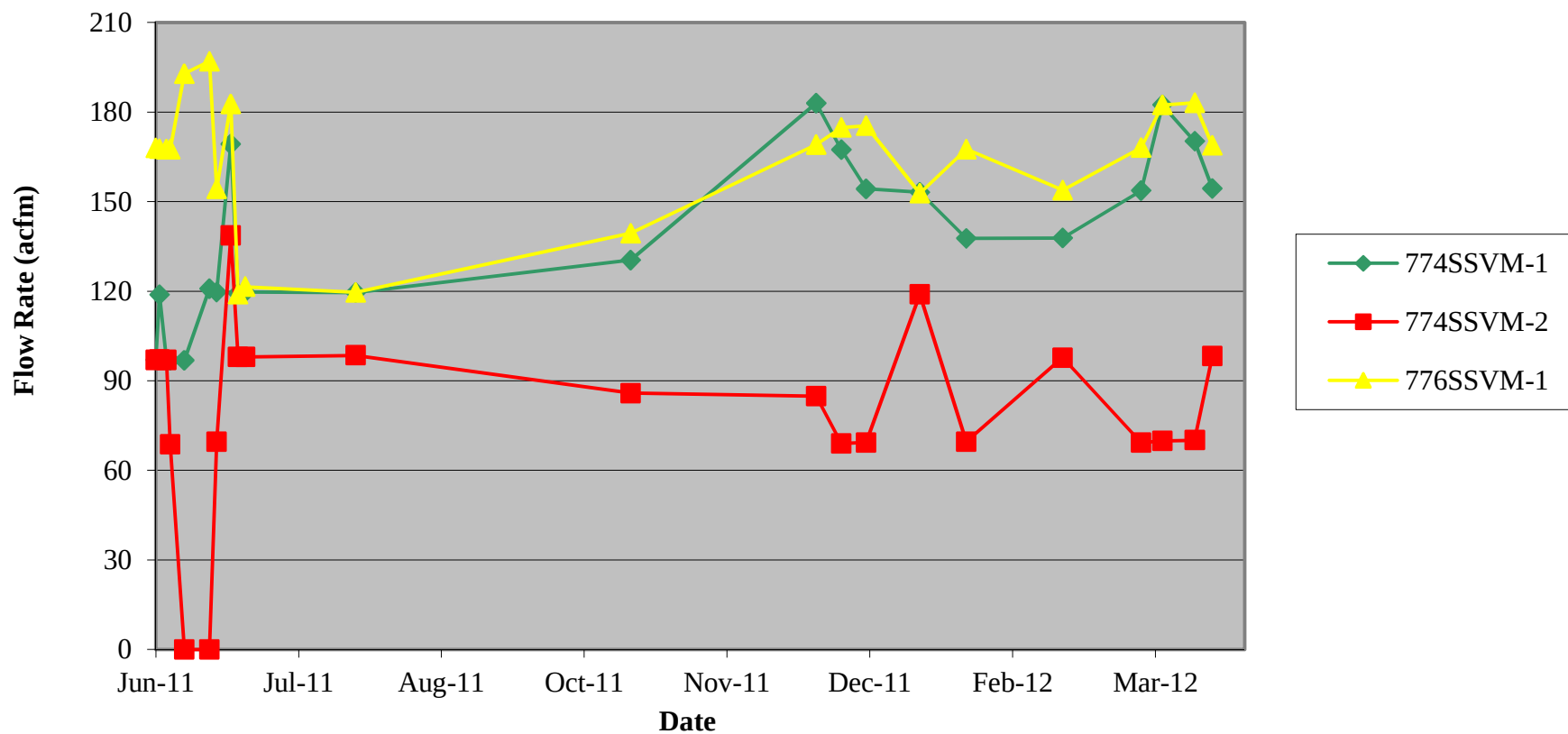
Figure 3-1 774SSVM-1, -2 and 776SSVM-1 Long Term Operation Flow Rate (June 2011 through March 2012)
