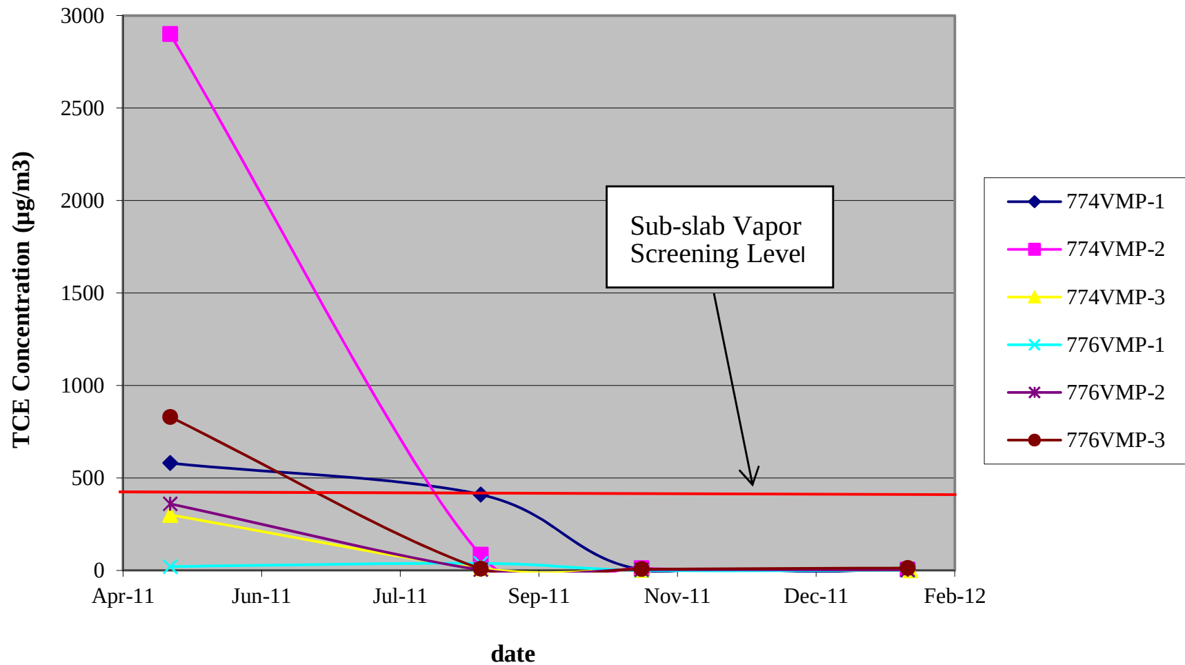
Figure 3-5 Trend Chart Sub-Slab Results Building 774 and 776 (May 2011 through March 2012)
