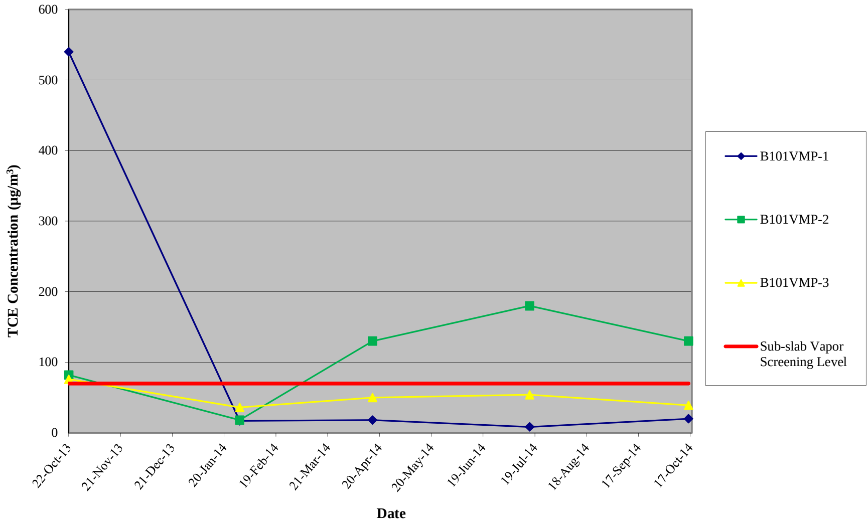
Figure 7 Sub-Slab TCE Trend Chart (October 2013 through December 2014)
