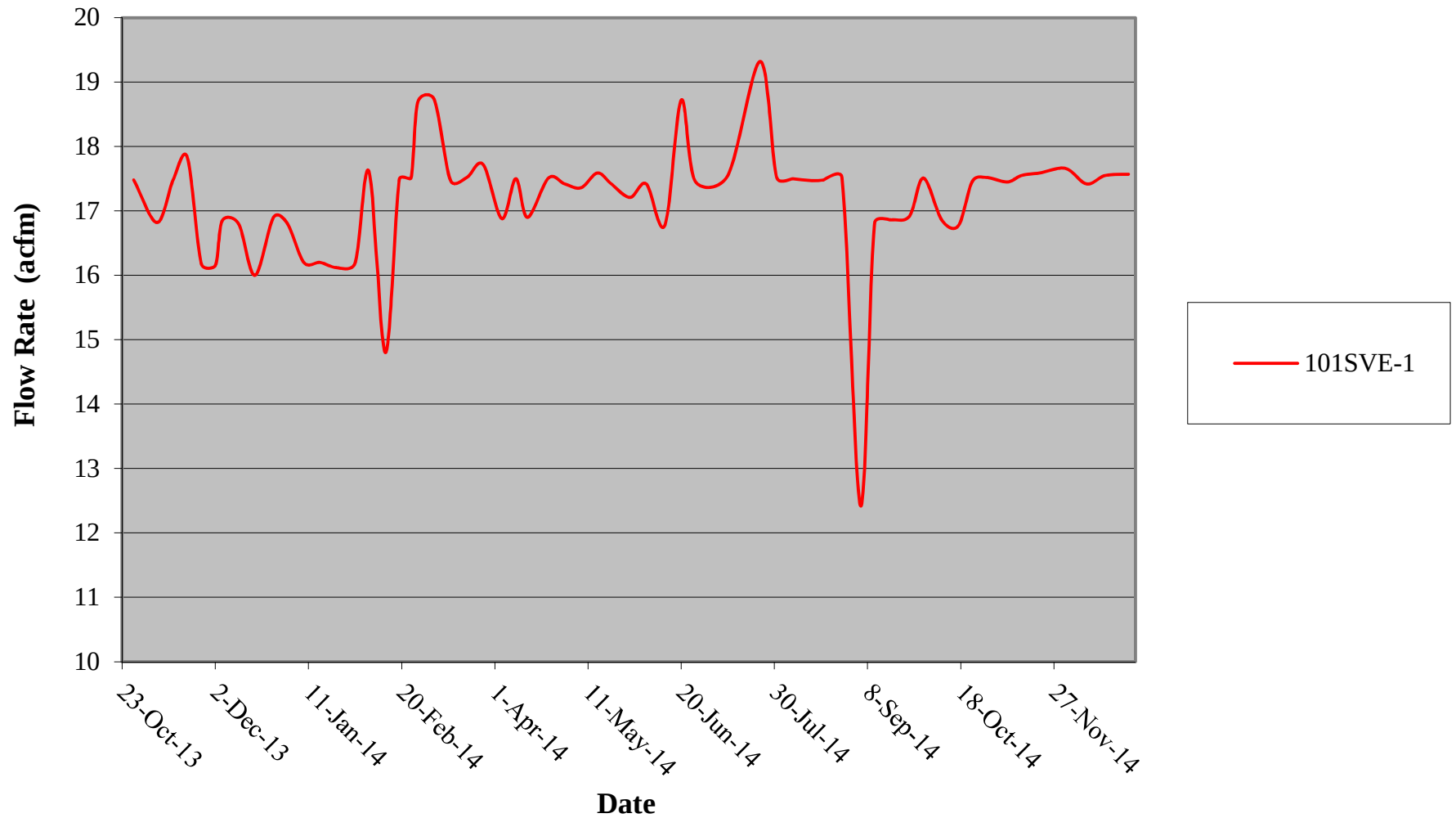
Figure 6 101SVE-1 Long Term Operation Flow Rate (October 2013 through December 2014)
