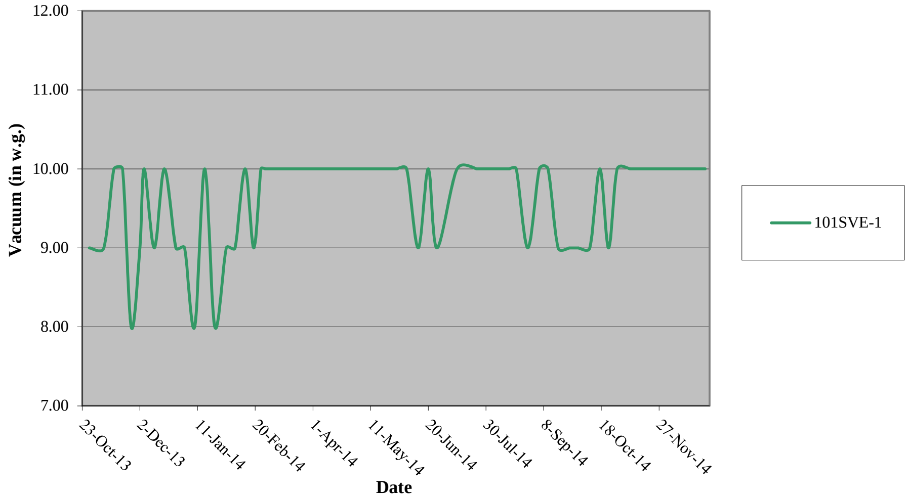
Figure 5 101SVE-1 Long Term Operation Vacuum Rate (October 2013 through December 2014)
