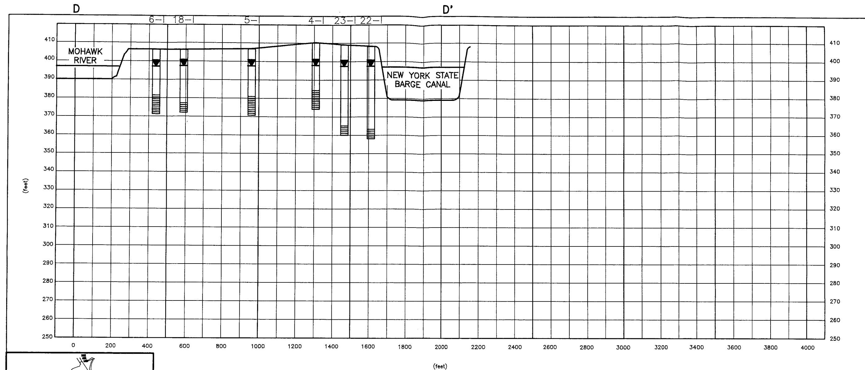
SECTION D-D'
