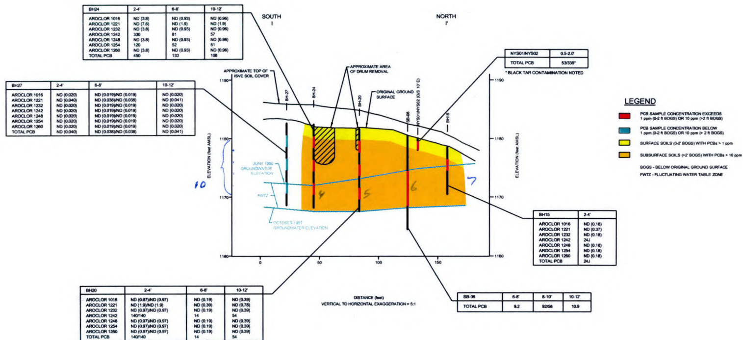
figure 3 PCB CONCENTRATIONS IN SOILS, EXCAVATION AREA A, CROSS-SECTION I-I' SOLVENT SAVERS SITE Lincklaen, New York
