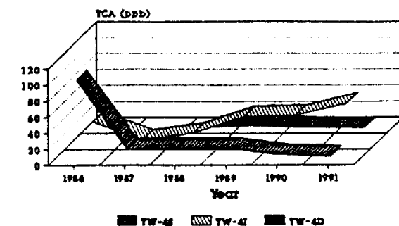
Gladding Cordage Site Monitoring Wells TW-4
