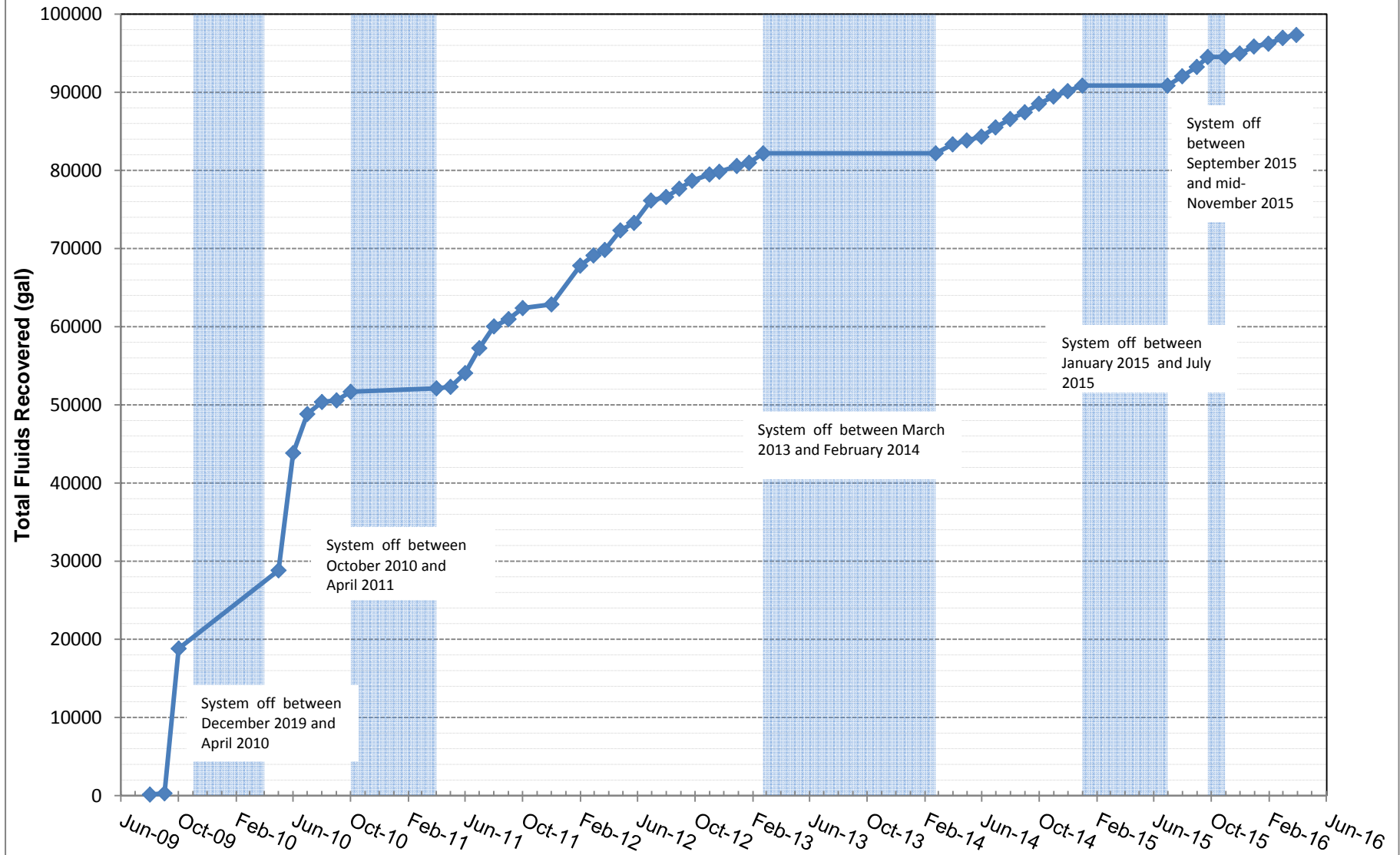
Figure 2 Total Fluids Recovery (2009 - March 2016) NYSEG Norwich Former MGP Site
