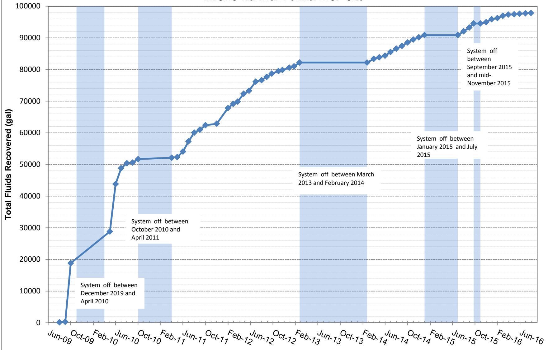
Figure 2 Total Fluids Recovery (2009 - July 2016) NYSEG Norwich Former MGP Site
