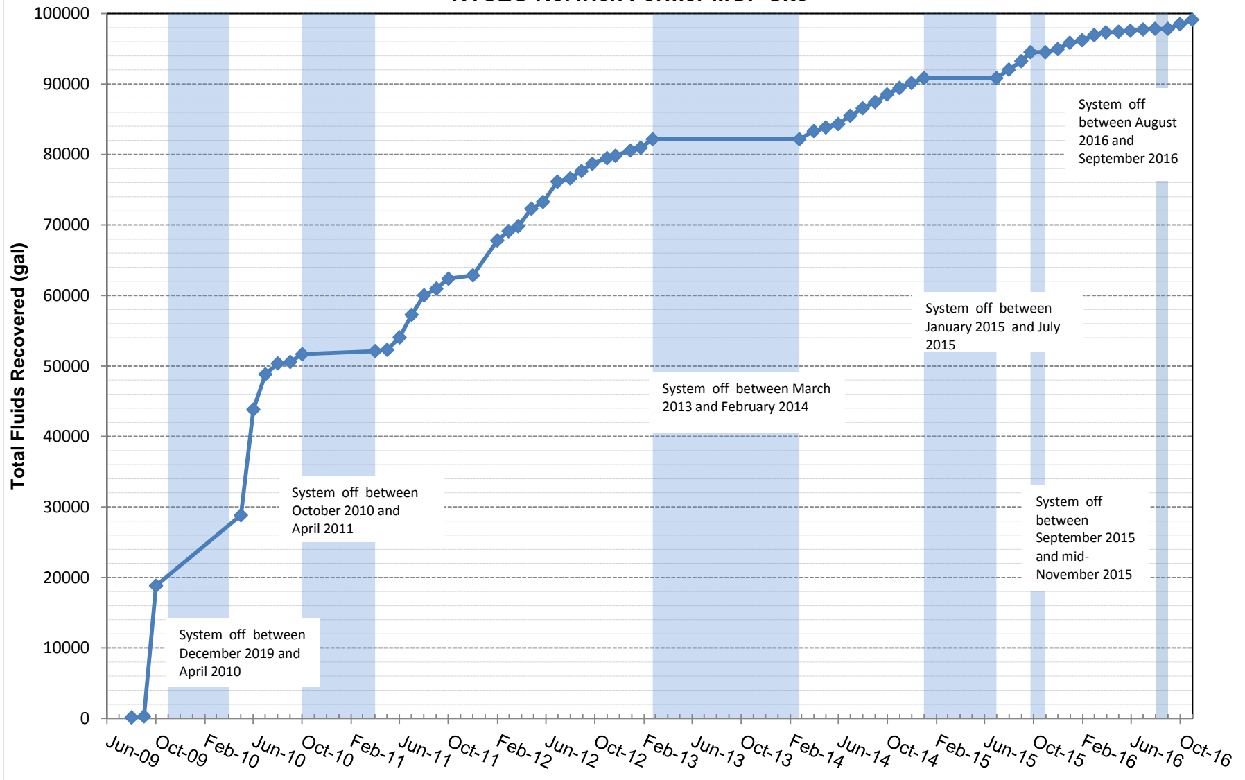
Figure 2 Total Fluids Recovery (2009 -October 2016) NYSEG Norwich Former MGP Site
