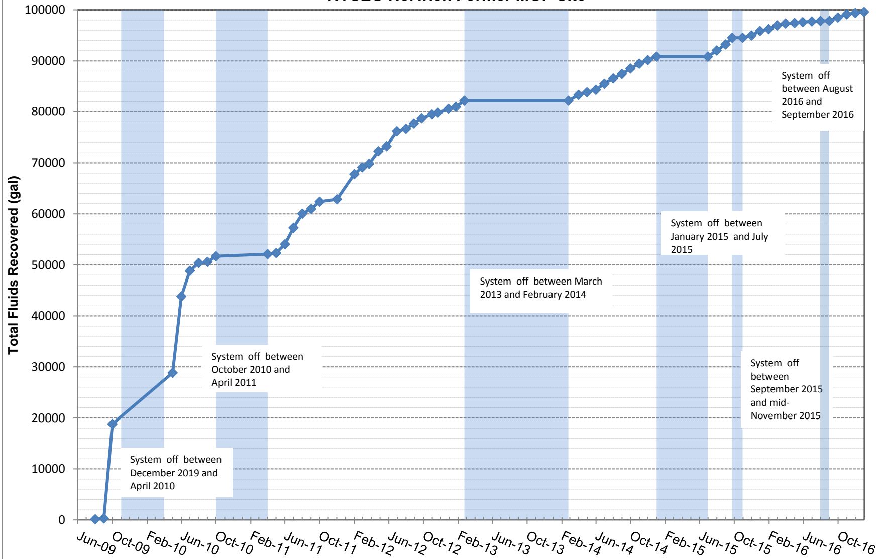
Figure 2 Total Fluids Recovery (2009 -December 2016) NYSEG Norwich Former MGP Site
