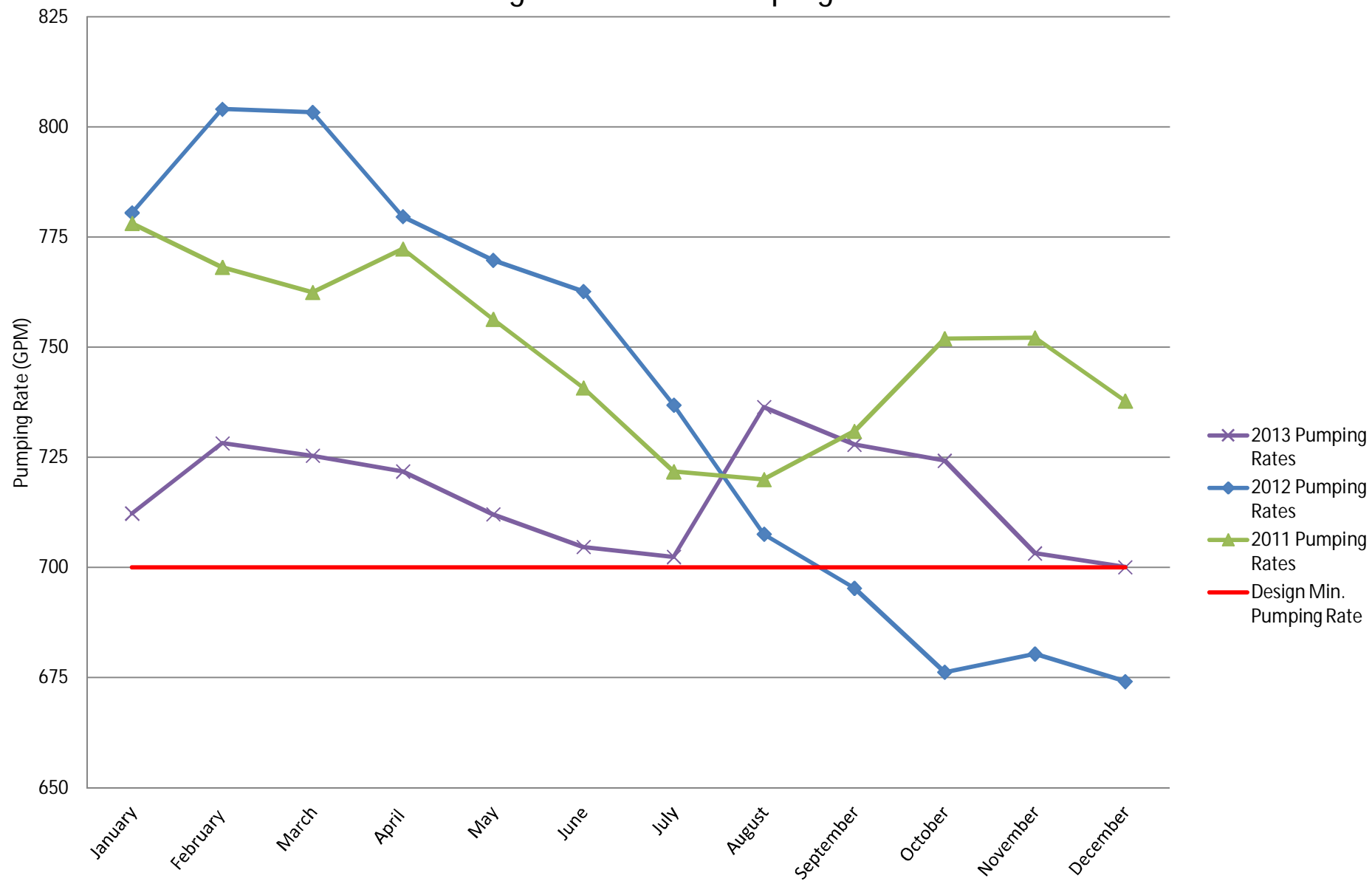
Chart 14: 2011, 2012 & 2013 Pumping Rates vs. Design Minimum Pumping Rate
