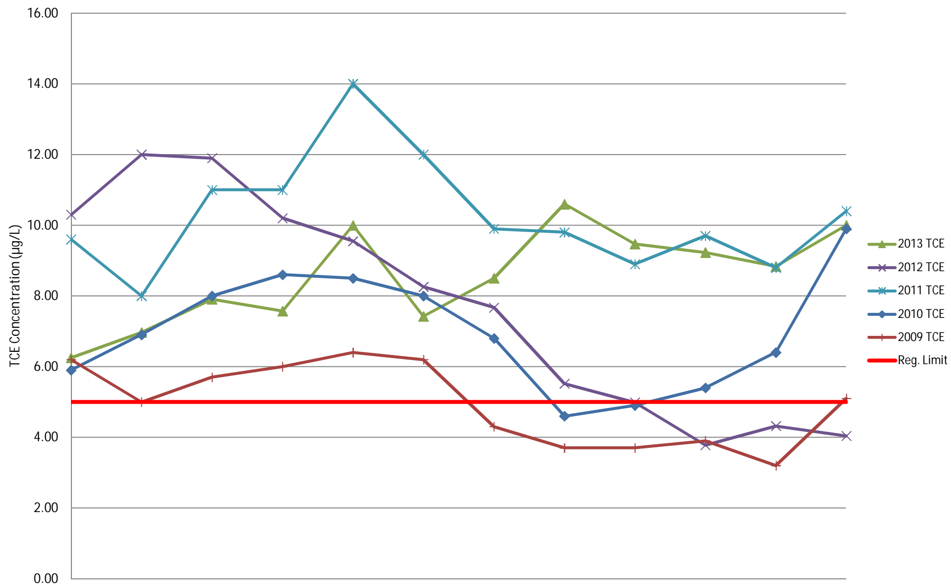
Chart 4: Tower Influent TCE Concentrations (µg/L) 2009, 2010, 2011, 2012 & 2013
