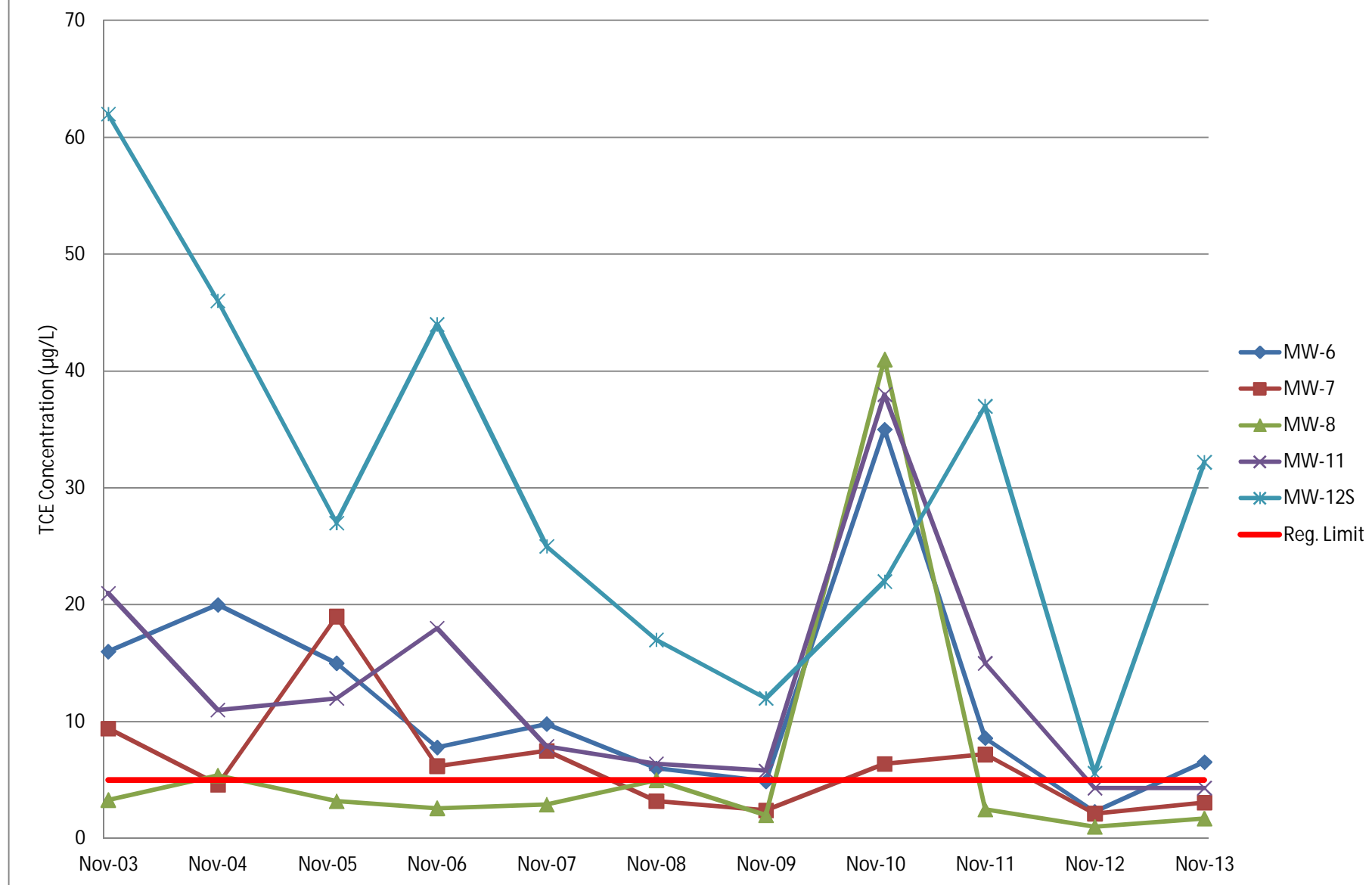
Chart 9: Interior Shallow Wells 10-Year TCE Concentrations ( \mu\text{g/L} )
