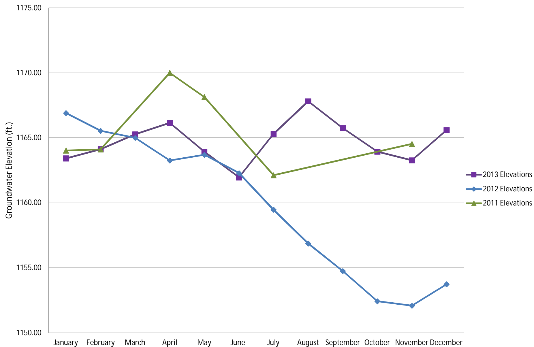
Chart 15: 2011, 2012 & 2013 Recovery Well Groundwater Elevations
