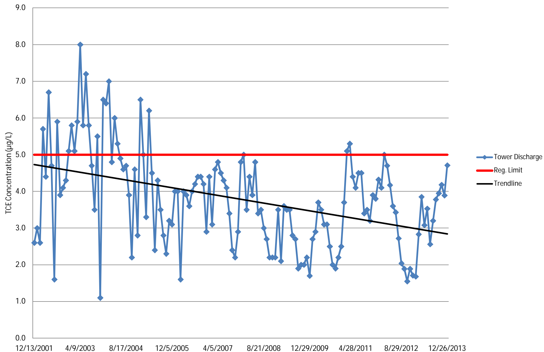
Chart 2: Tower Discharge TCE Concentrations ( \mu\text{g/L} ) December 2001 to December 2013
