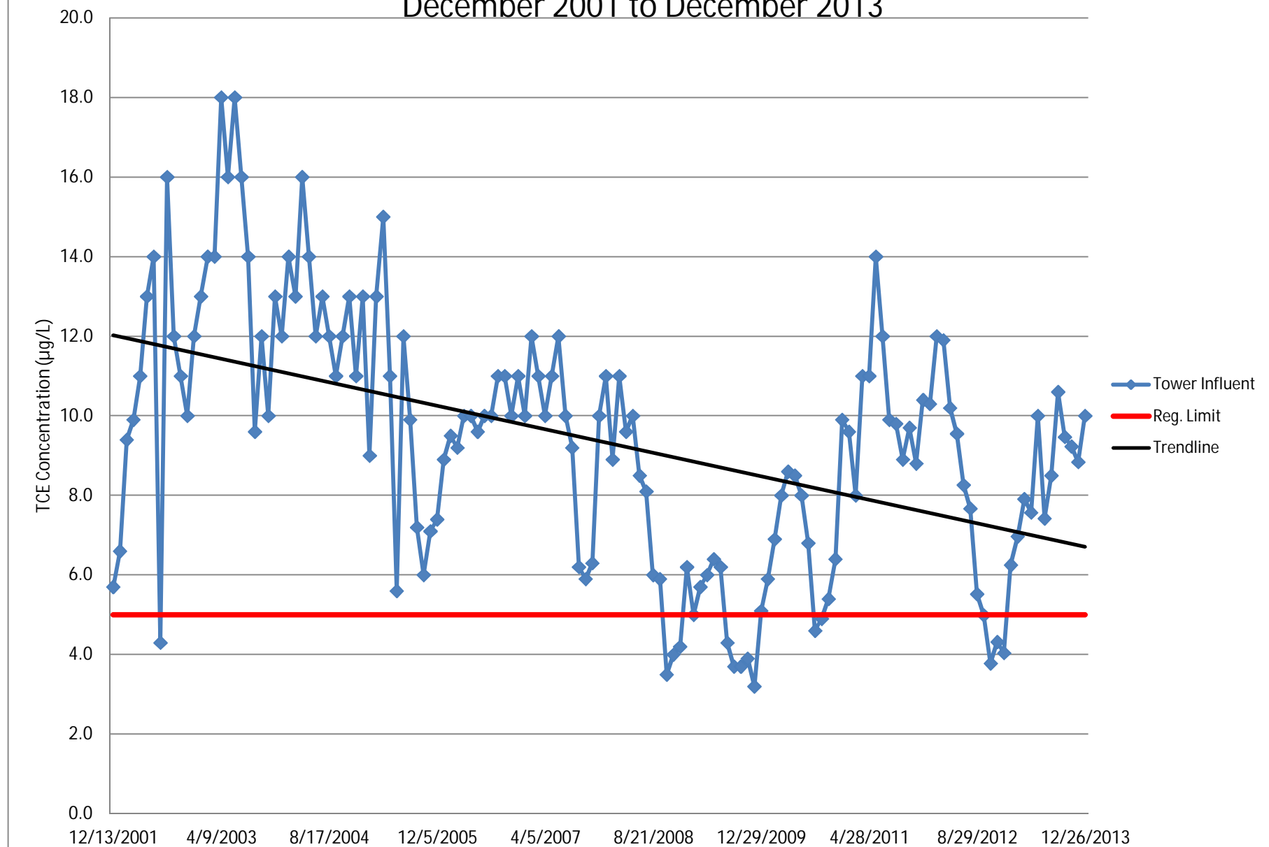
Chart 1: Tower Influent TCE Concentrations ( \mu\text{g/L} ) December 2001 to December 2013
