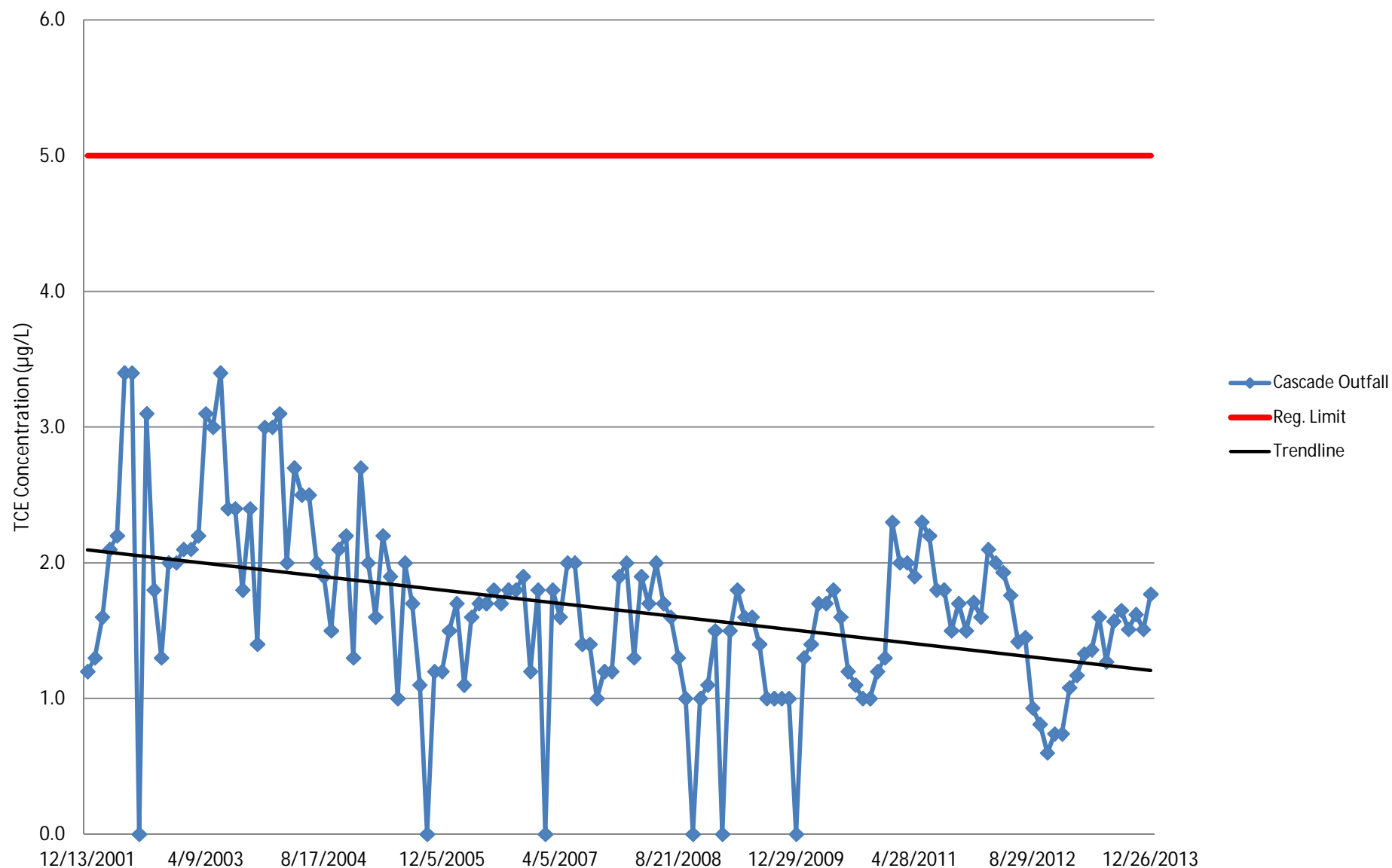
Chart 3: Cascade Outfall TCE Concentrations ( \mu\text{g/L} ) December 2001 to December 2013
