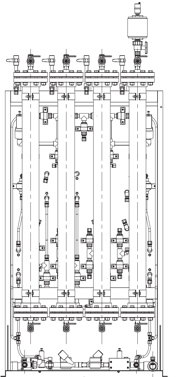
BACK ELEVATION
