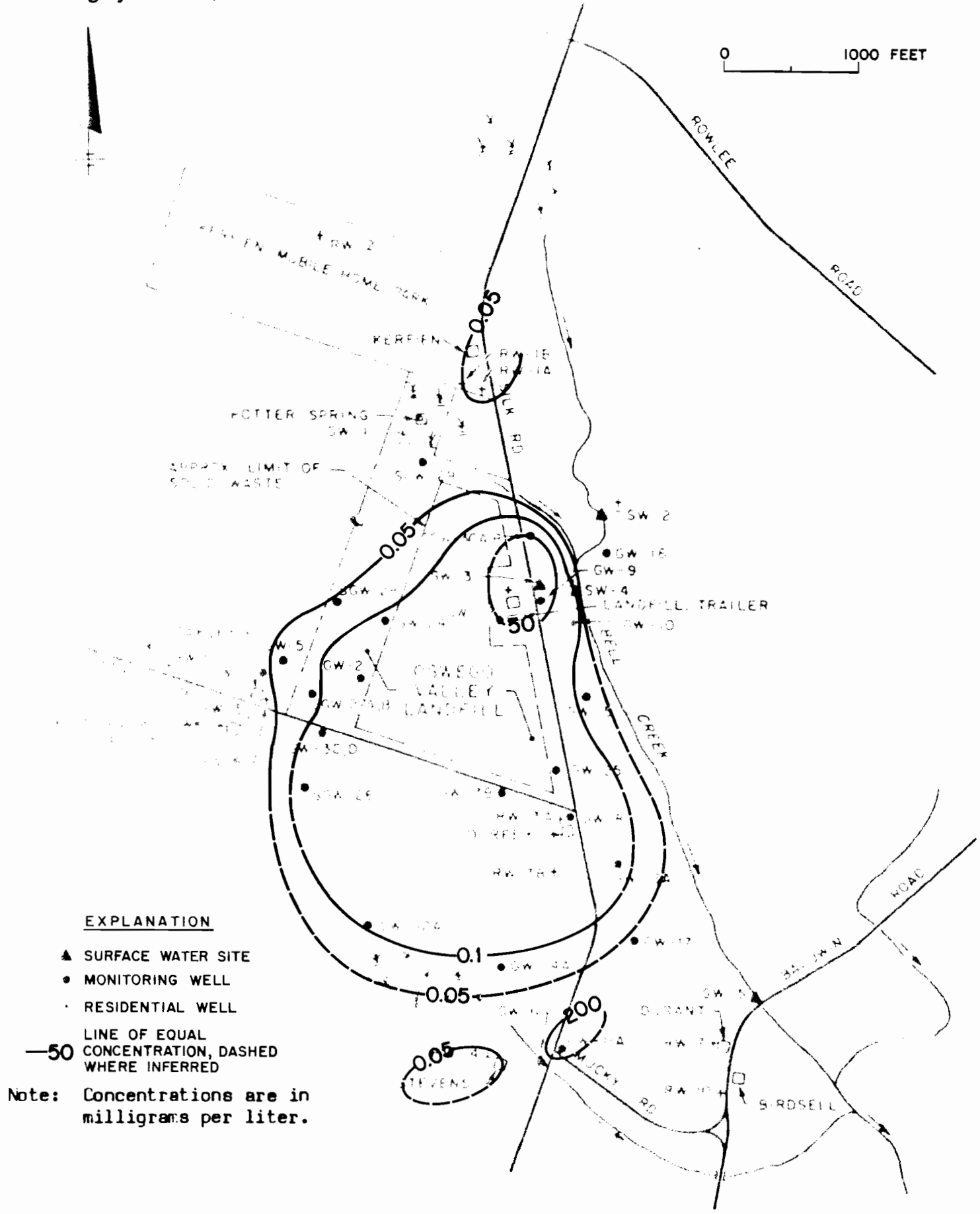
IRON CONCENTRATIONS IN THE SHALLOW WATER BEARING ZONE OSWEGO VALLEY LANDFILL, VOLNEY, NEW YORK
