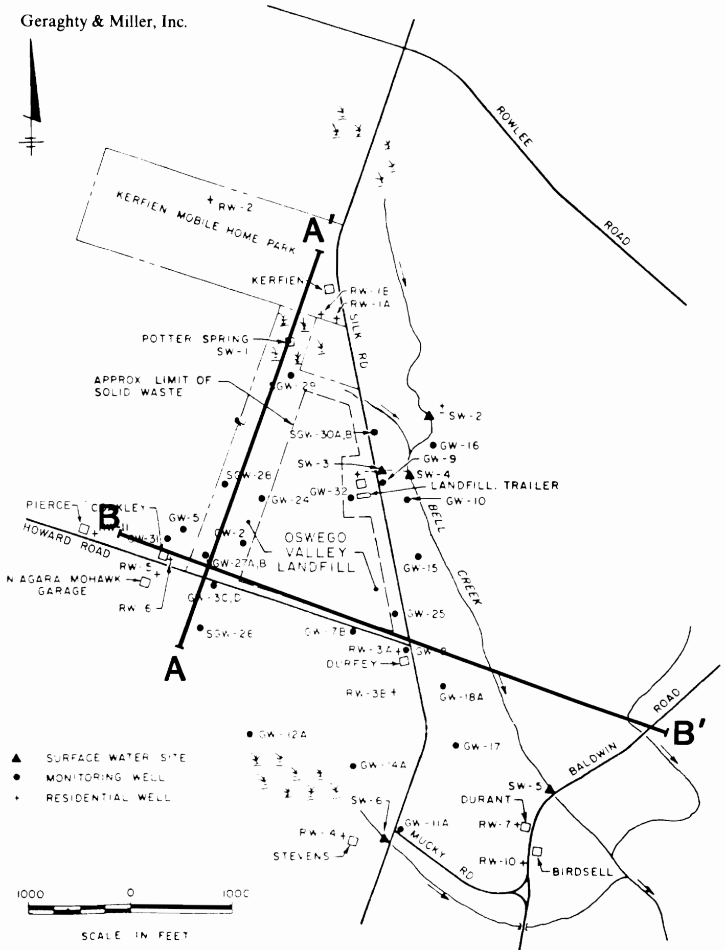
LINE OF GEOLOGIC CROSS SECTIONS OSWEGO VALLEY LANDFILL, VOLNEY, NEW YORK
