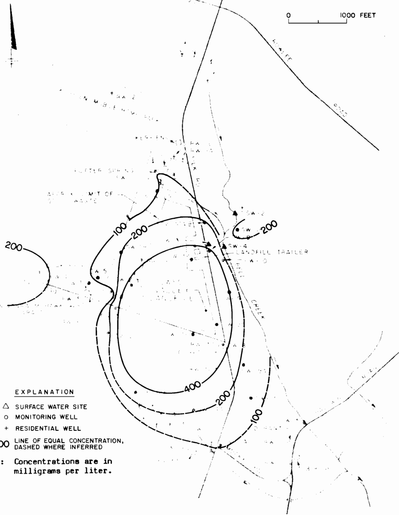
ALKALINITY CONCENTRATIONS IN THE SHALLOW WATER BEARING ZONE OSWEGO VALLEY LANDFILL, VOLNEY, NEW YORK
