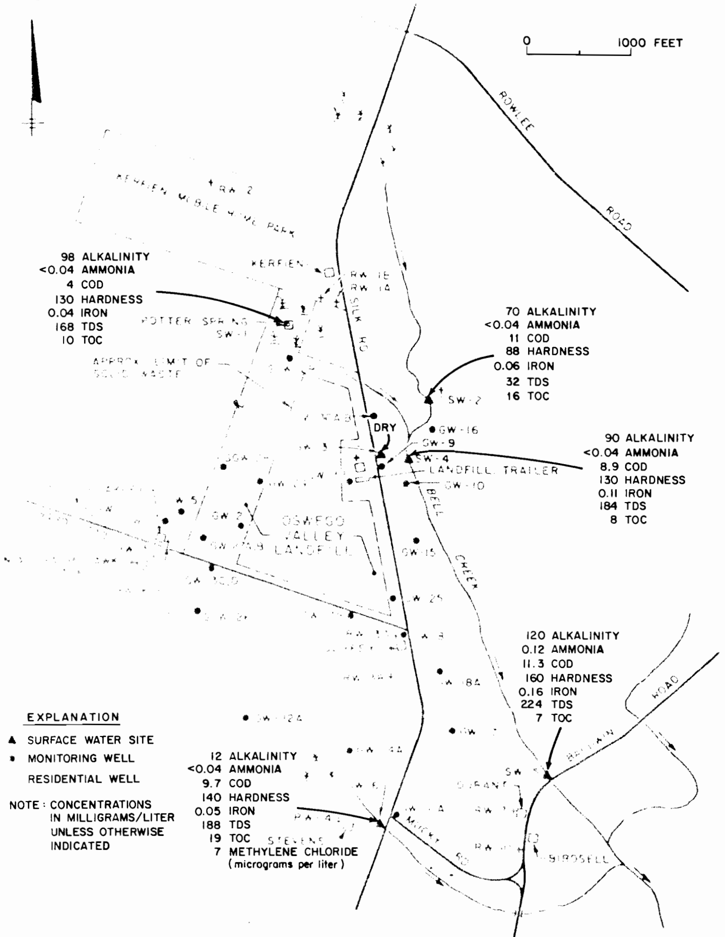
CONCENTRATIONS OF INORGANIC AND ORGANIC COMPOUNDS IN SURFACE WATER SAMPLES JANUARY 26, 1985 OSWEGO VALLEY LANDFILL, VOLNEY, NEW YORK
