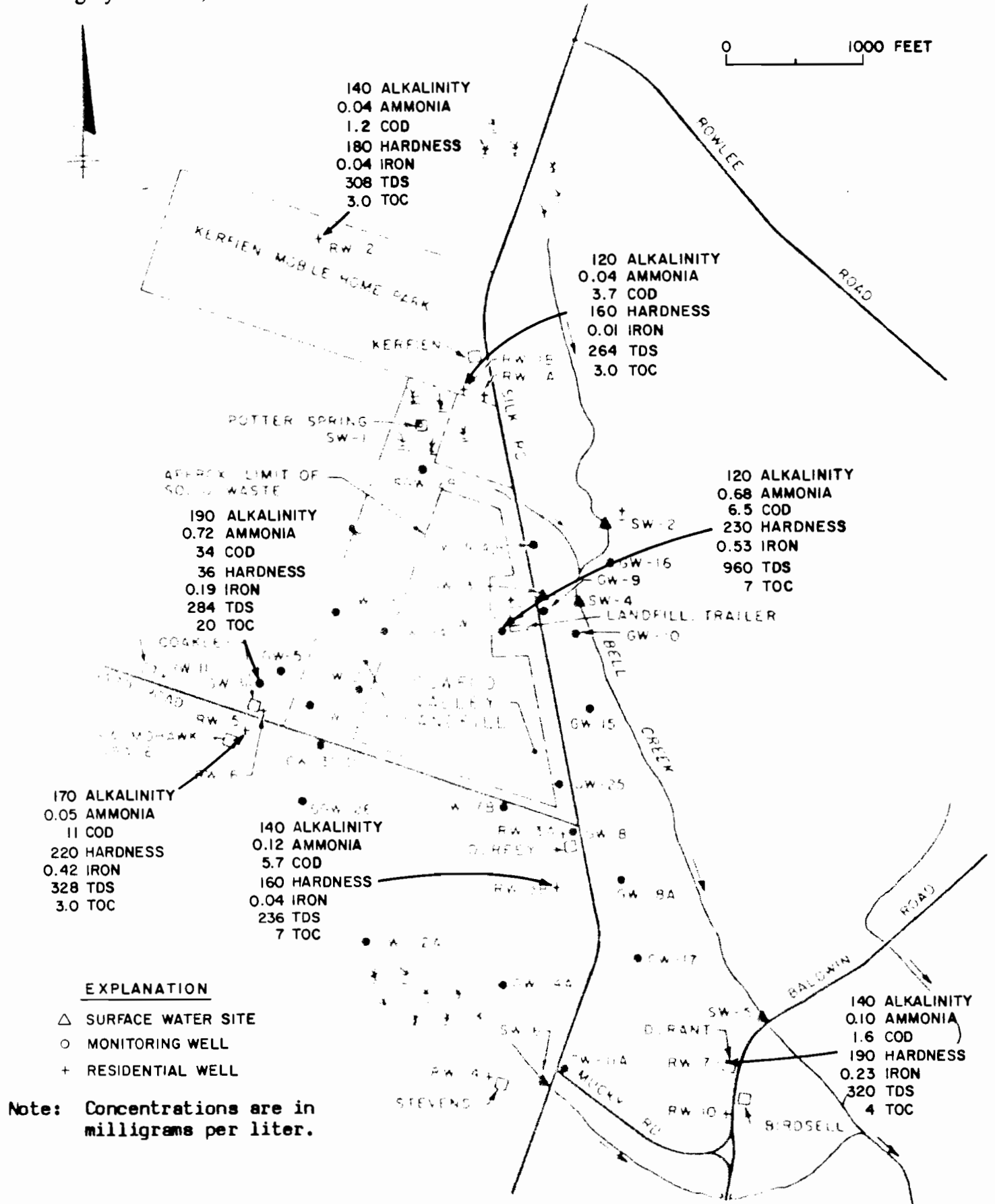
CONCENTRATIONS OF INORGANIC COMPOUNDS IN THE BEDROCK AQUIFER (INCLUDES ANALYTICAL RESULTS FROM SAMPLES COLLECTED FROM THE UNCONSOLIDATED ZONE - BEDROCK INTERFACE) OSWEGO VALLEY LANDFILL, VOLNEY, NEW YORK
