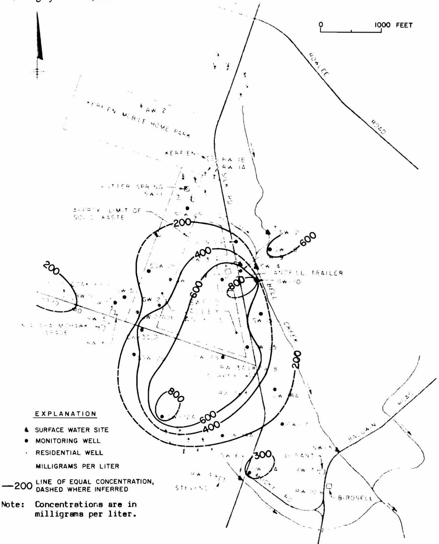
TOTAL DISSOLVED SOLIDS CONCENTRATIONS IN THE SHALLOW WATER-BEARING ZONE OSWEGO VALLEY LANDFILL, VOLNEY, NEW YORK
