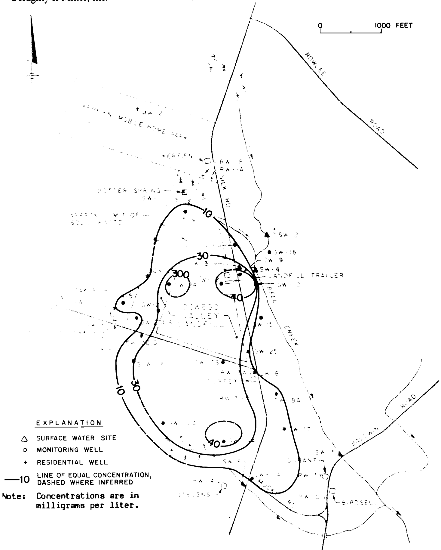
CHEMICAL OXYGEN DEMAND CONCENTRATIONS IN THE SHALLOW WATER BEARING ZONE OSWEGO VALLEY LANDFILL, VOLNEY, NEW YORK
