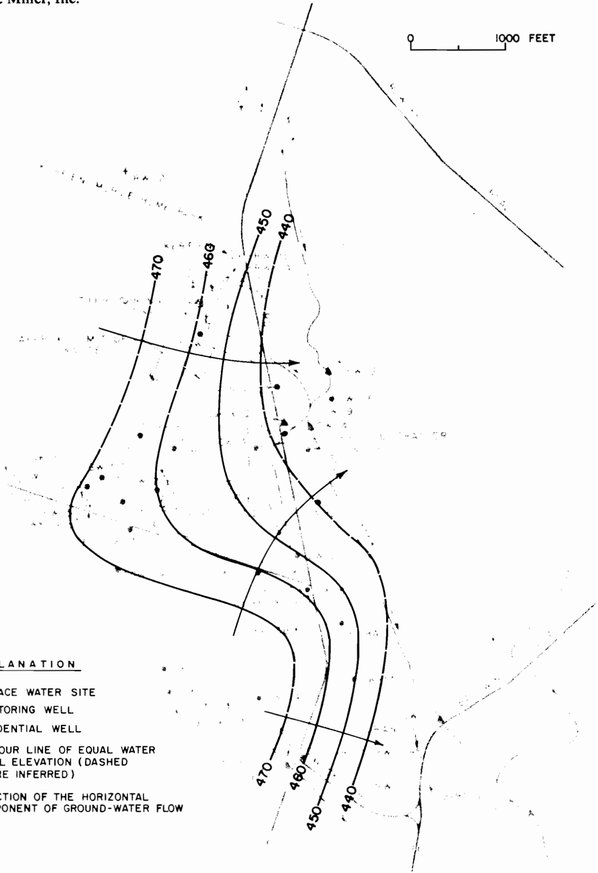
PIEZOMETRIC SURFACE MEASURED 1-28-85 AT THE OSWEGO VALLEY LANDFILL, VOLNEY, NEW YORK
