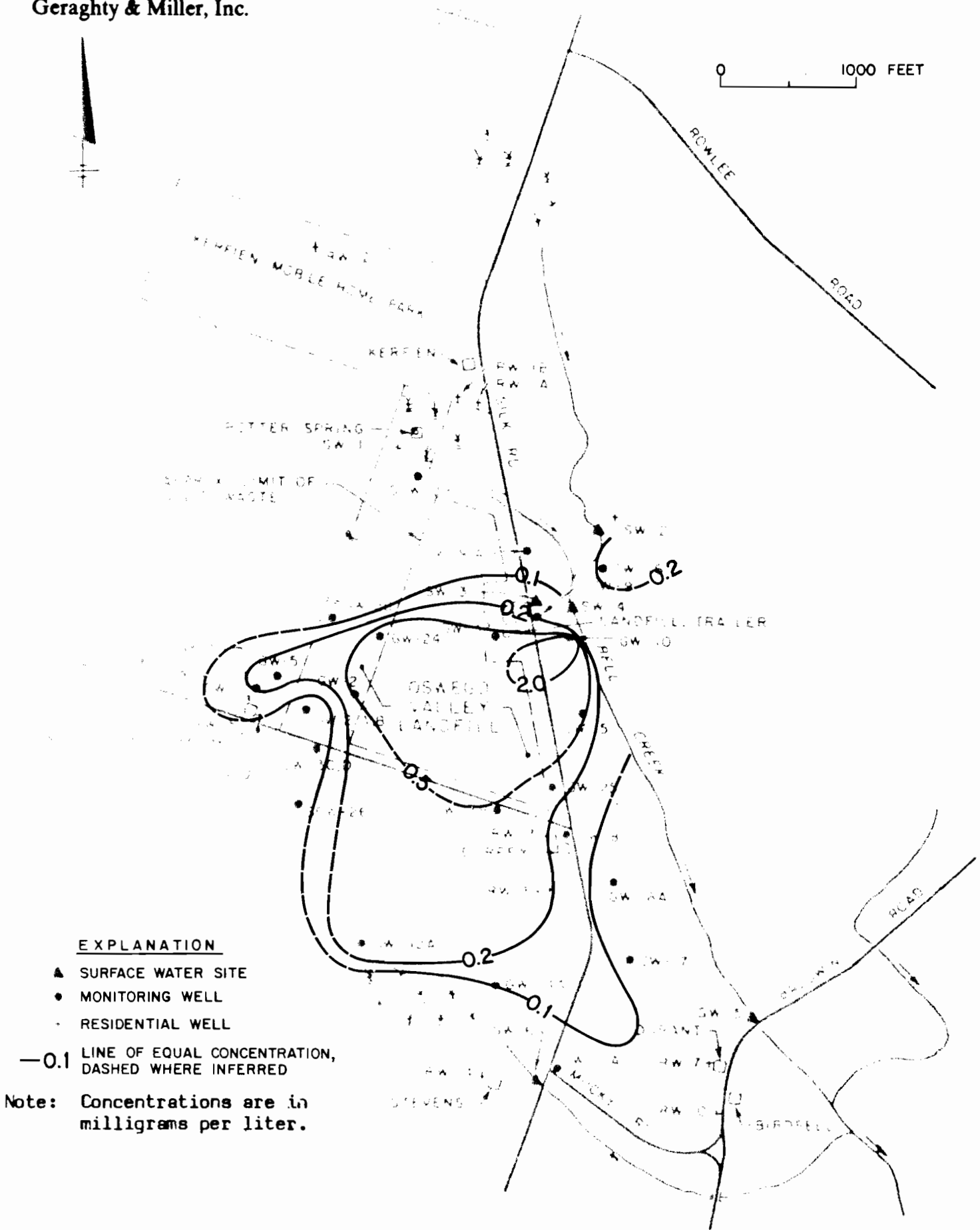
AMMONIA CONCENTRATIONS IN THE SHALLOW WATER BEARING ZONE OSWEGO VALLEY LANDFILL, VOLNEY, NEW YORK
