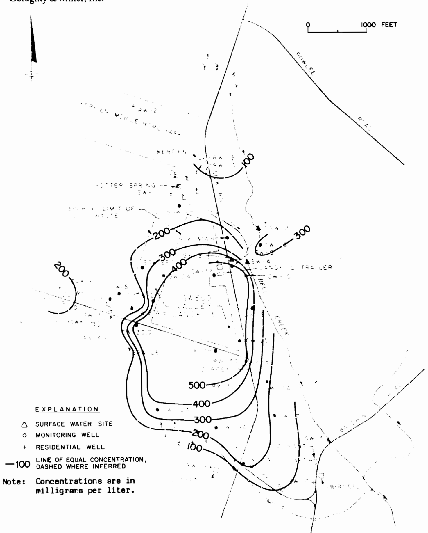
HARDNESS CONCENTRATIONS IN THE SHALLOW WATER BEARING ZONE OSWEGO VALLEY LANDFILL, VOLNEY, NEW YORK
