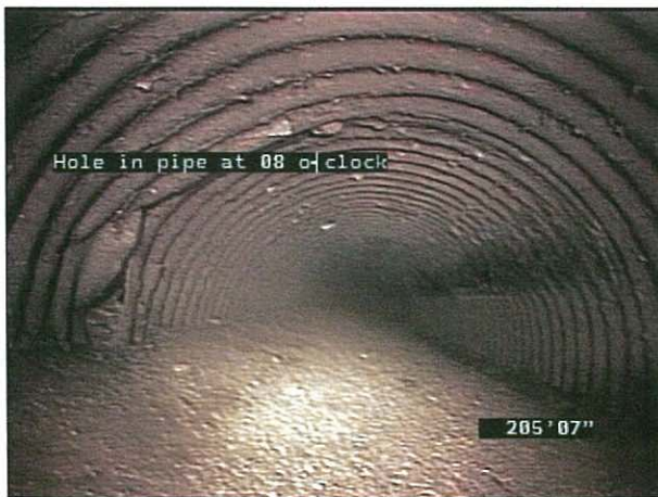
IMAGE: 29a, TAPE #: 01, 00:00:00 205.55FT, Hole in pipe at 08 o'clock
