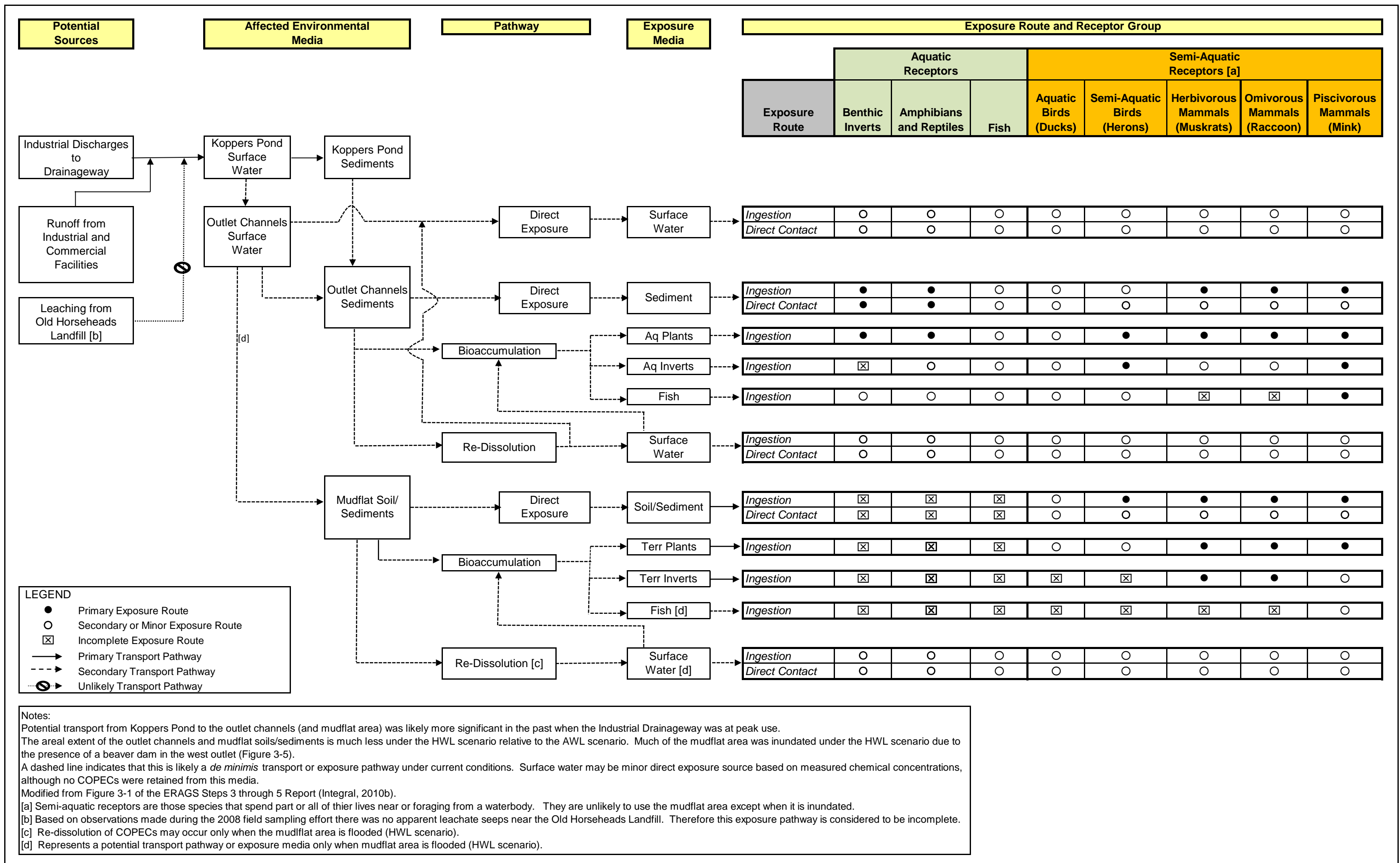
Figure 28c. Conceptual Site Model for the Outlet Channels and Mudflat Area under the AWL and HWL Scenarios Kentucky Avenue Wellfield OU4 - Koppers Pond, Horseheads, New York
