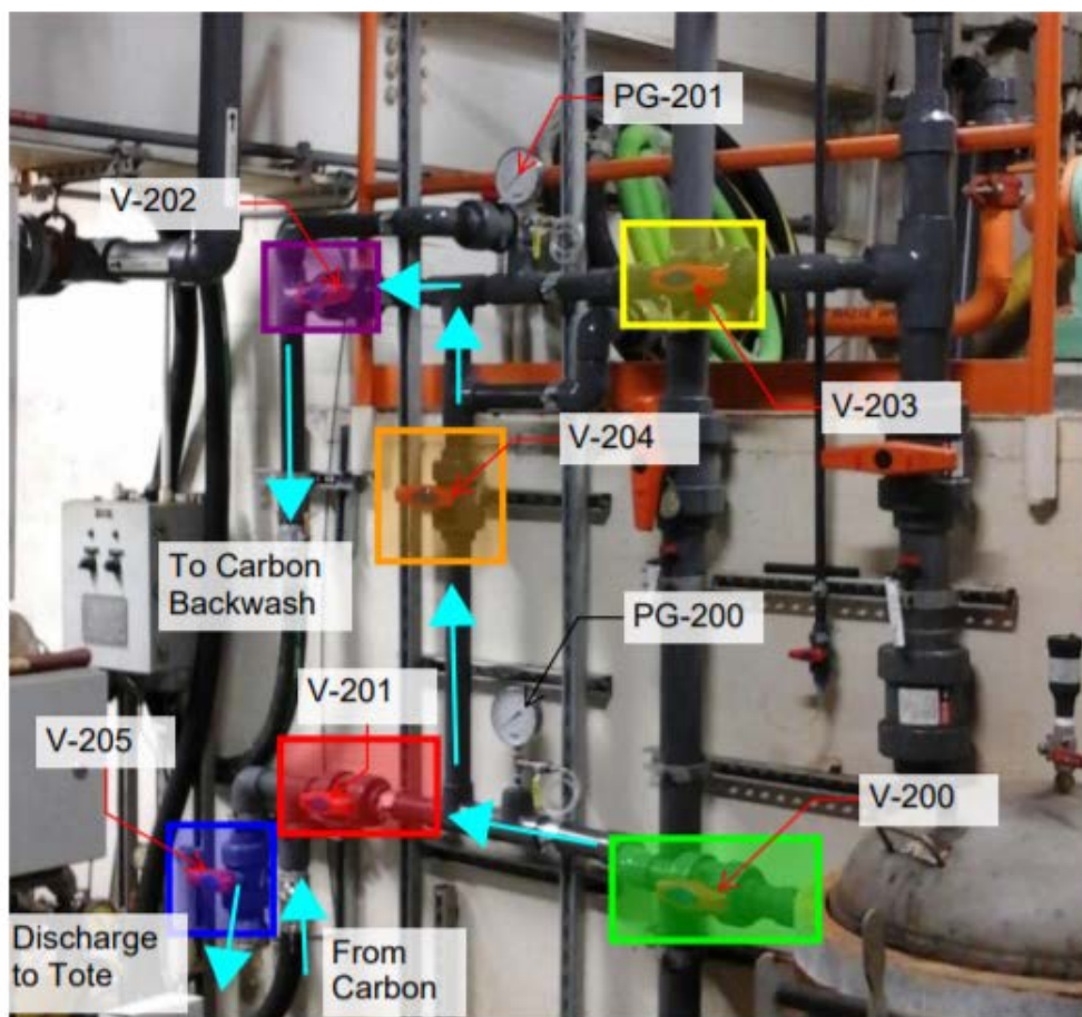
Figure 3 – Backwash Flow
