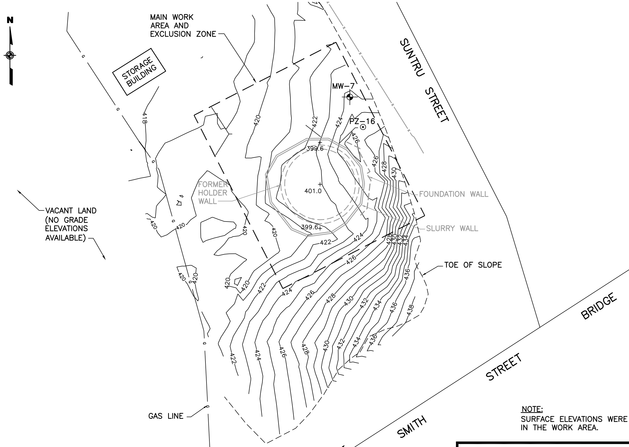
EAST STATION HOLDER IRM REMOVAL AREA FINAL CONTOUR PLAN OF FORMER GAS HOLDER REMOVAL WORK AREA URS FIGURE 3
