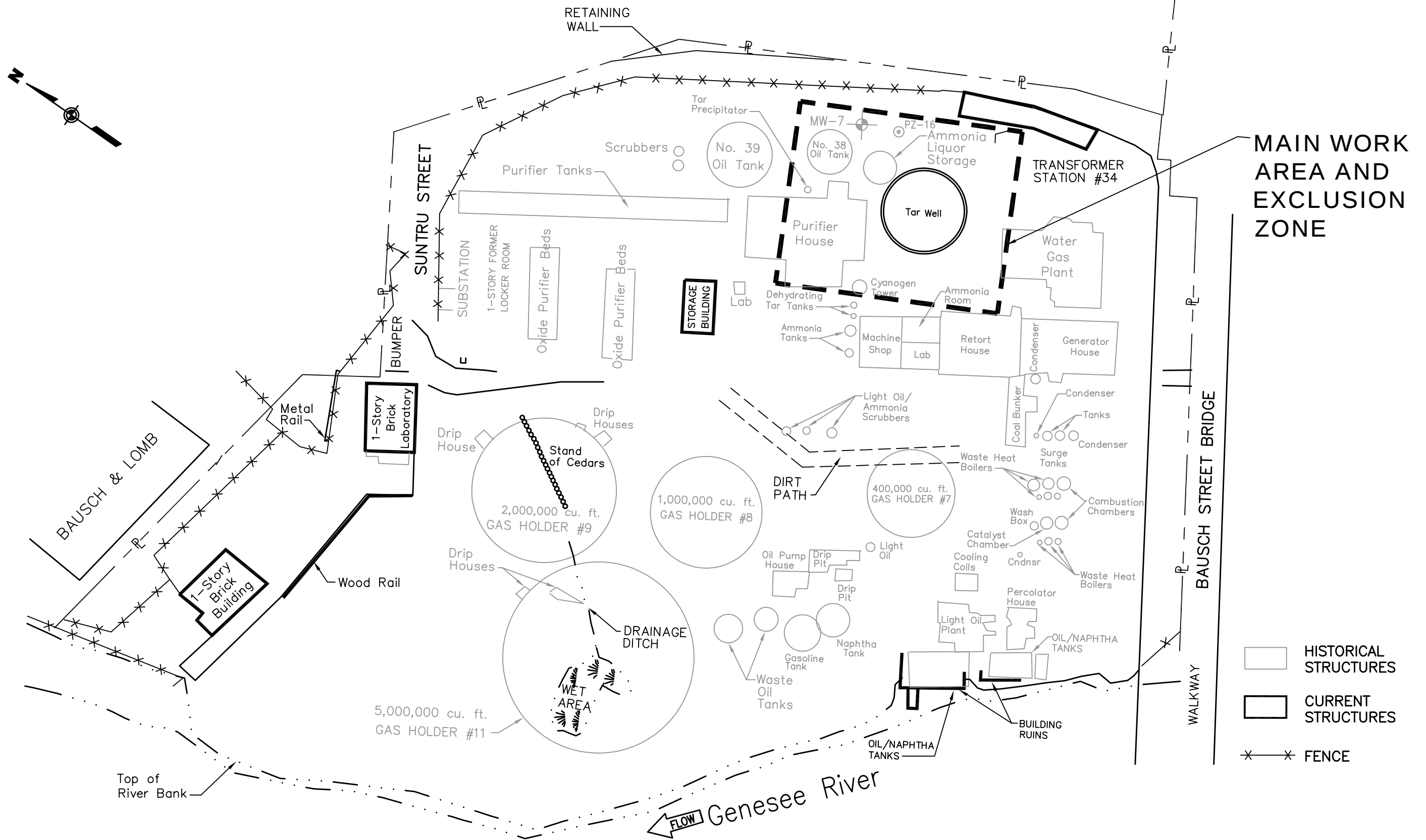
EAST STATION HOLDER REMOVAL IRM AREA BASE MAP
