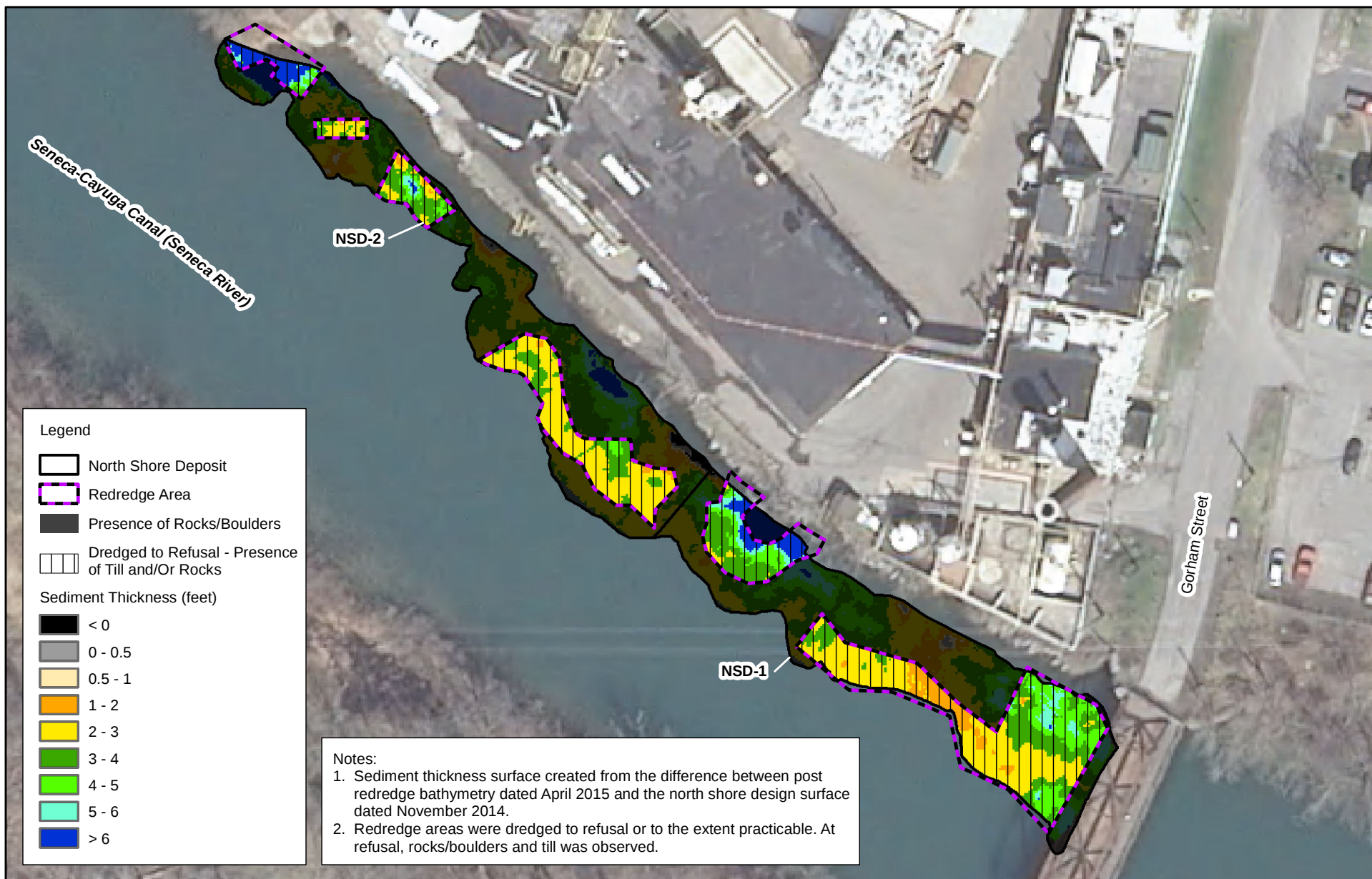
Figure 5 Final Dredge Completion Surface AOC A Sediment Removal Verification North Shore Deposit Former Hampshire Chemical Corp. Facility Waterloo, New York
