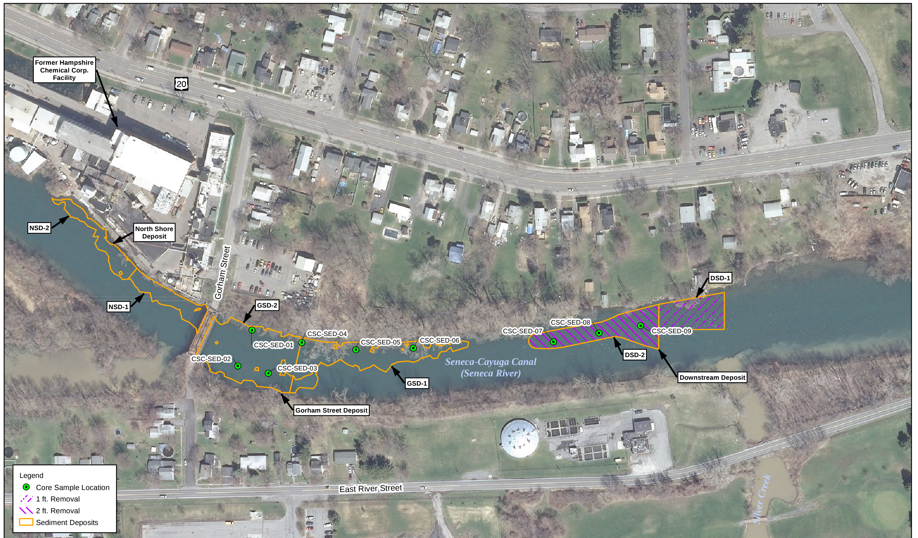
Figure 1 Sediment Core Verification Samples AOC A Sediment Removal Verification Technical Memorandum North Shore Deposit Former Hampshire Chemical Corp. Facility Waterloo, New York
