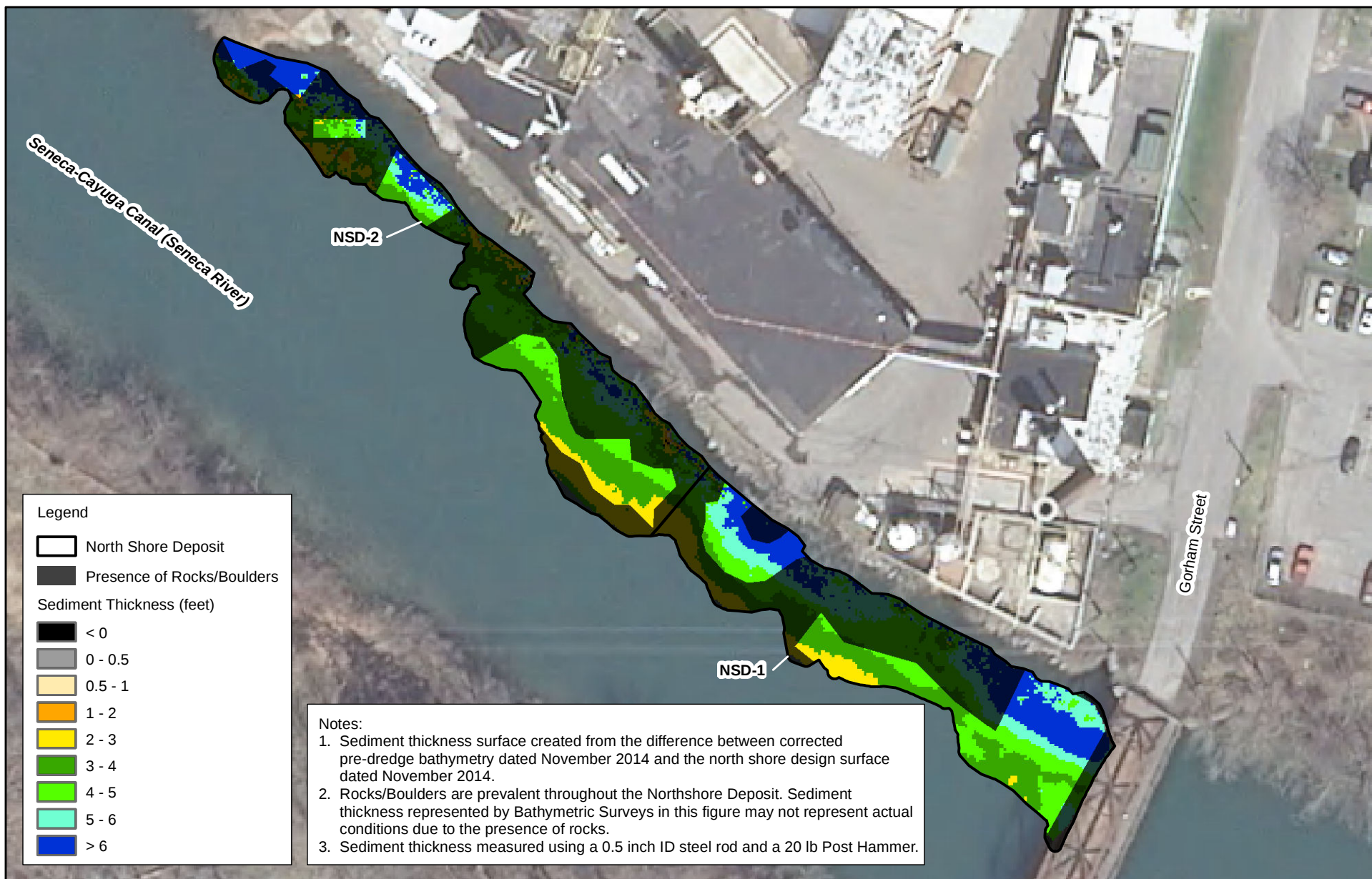
Figure 2 Sediment Thickness Map AOC A Sediment Removal Verification North Shore Deposit Former Hampshire Chemical Corp. Facility Waterloo, New York
