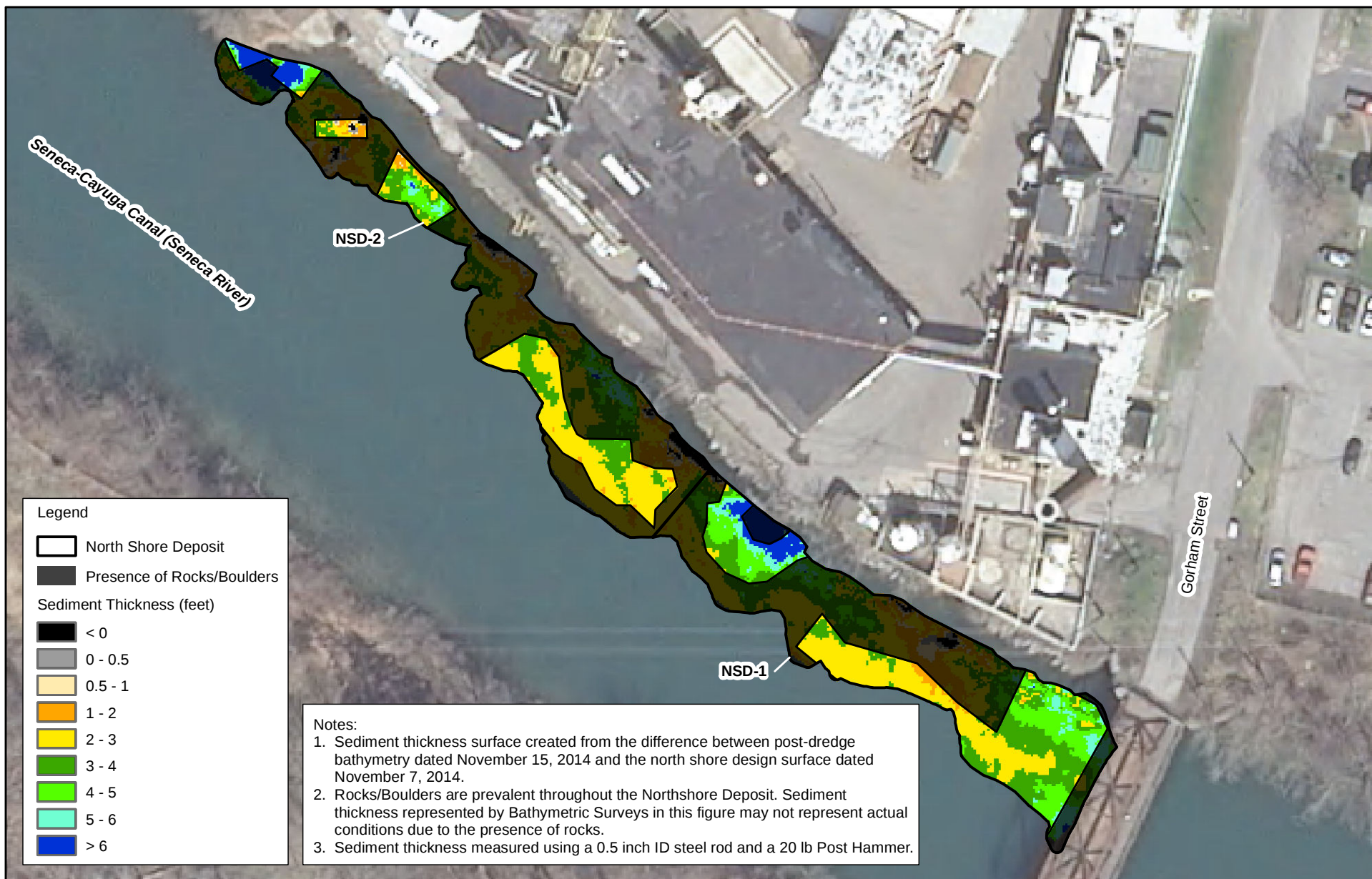
Figure 3 Post-Dredge Sediment Remaining AOC A Sediment Removal Verification North Shore Deposit Former Hampshire Chemical Corp. Facility Waterloo, New York
