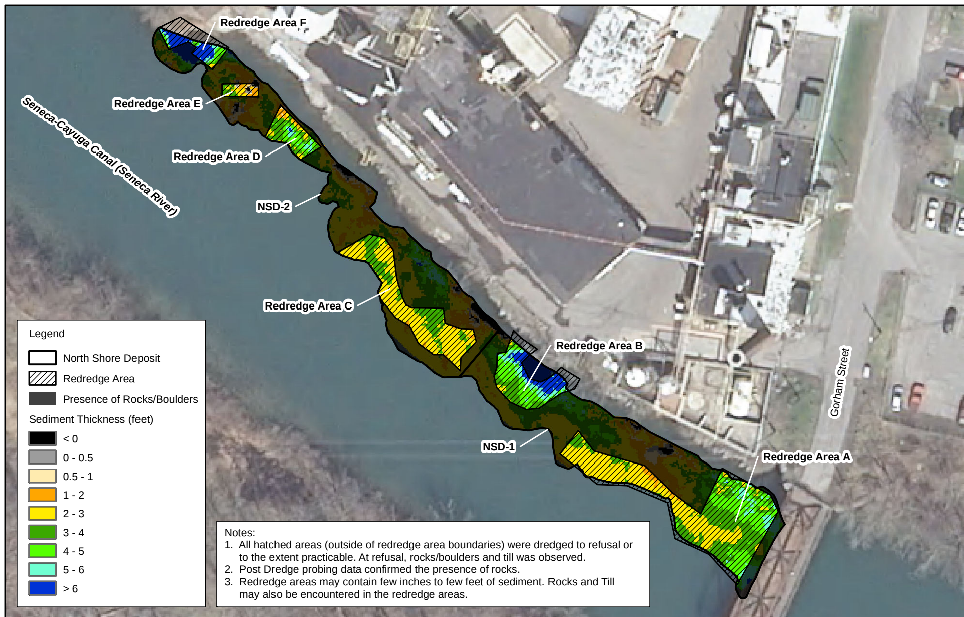
Figure 4 Redredge Area AOC A Sediment Removal Verification North Shore Deposit Former Hampshire Chemical Corp. Facility Waterloo, New York
