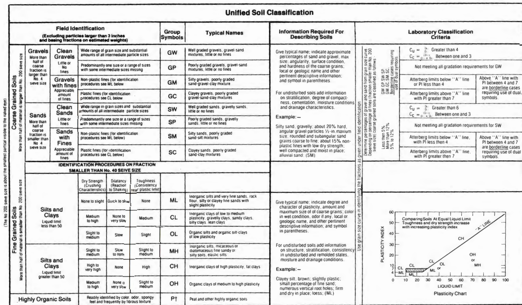
Figure 2-4 Unified Soil Classification System
