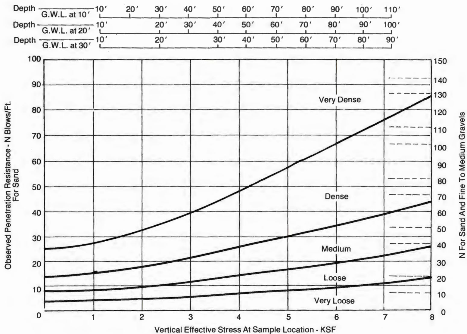
Figure 2-8 - Relative Density Of Sand From Standard Penetration Test
