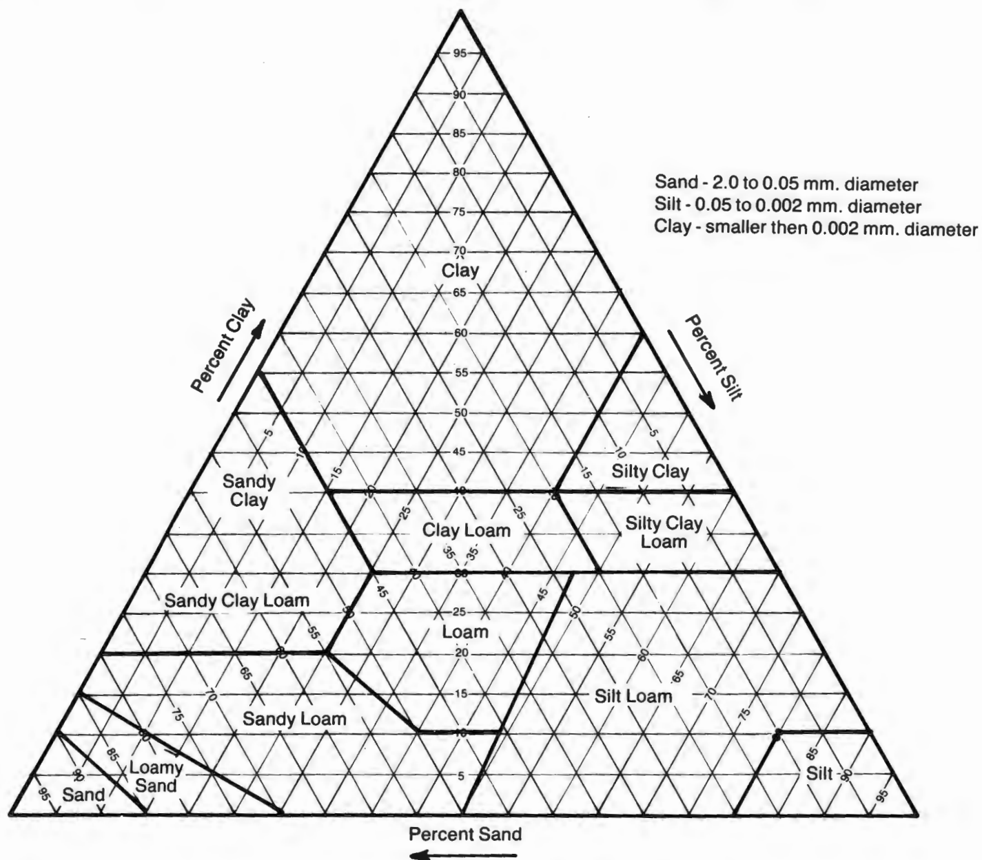
Figure EXP - 4BL5 Textural Soil Classification Chart, U.S. Department of Agriculture
