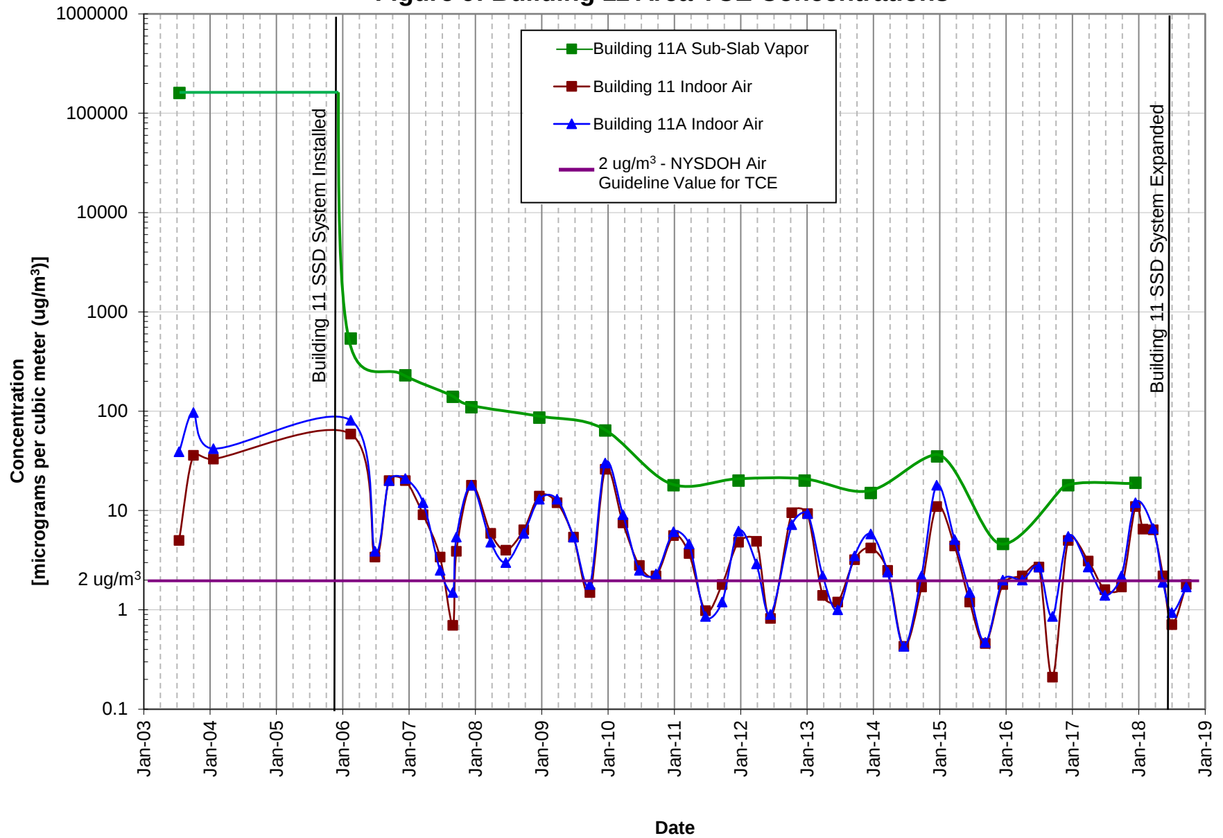
Figure 9: Building 11 Area TCE Concentrations
