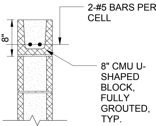
3 MASONRY BOND BEAM TYPICAL SECTION 1" □ 1'-0"
