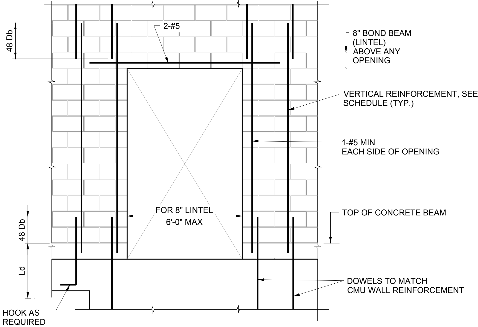
OPENING IN CMU WALL
