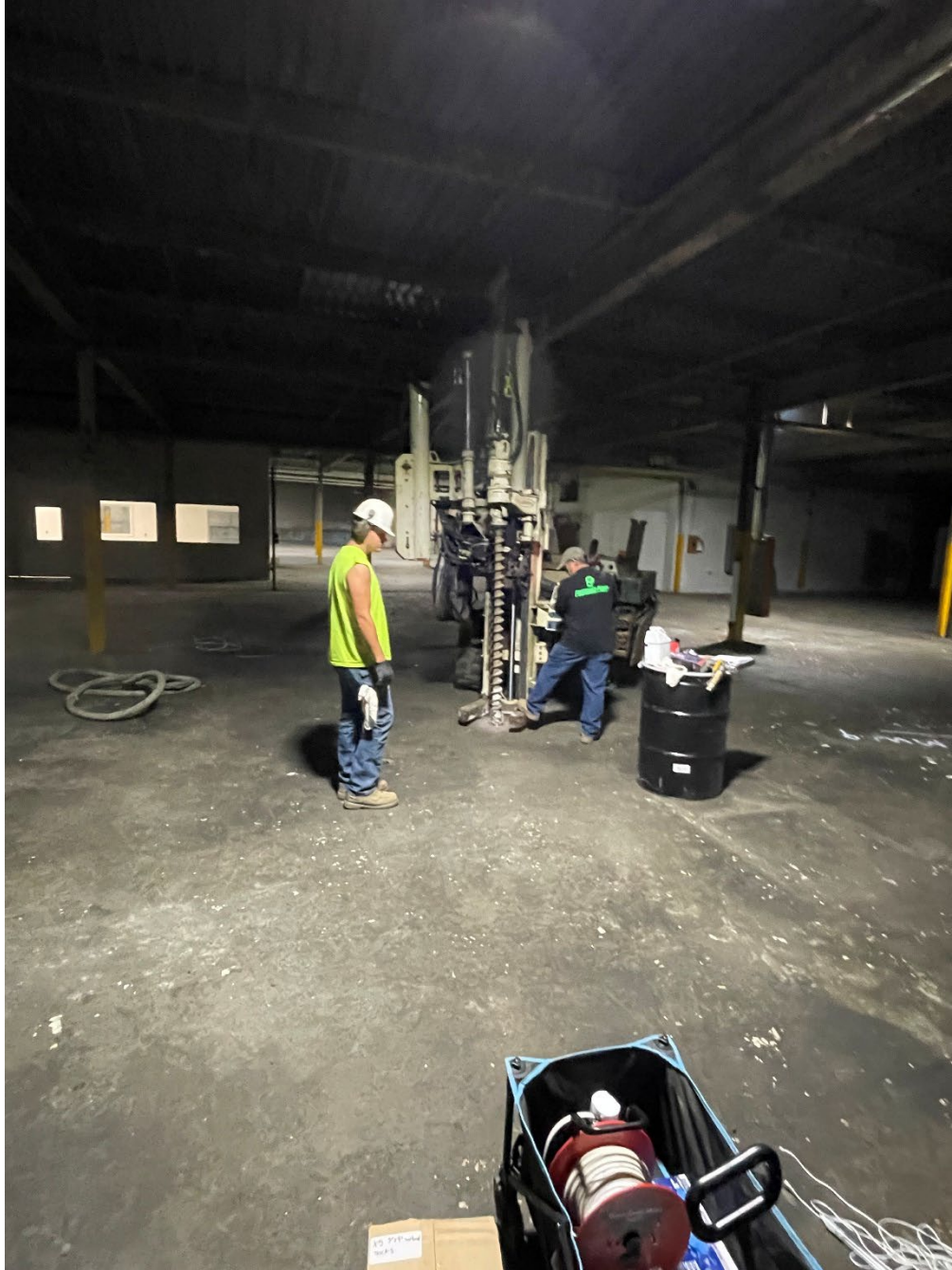
Auguring concrete at MW-9 injection well.
