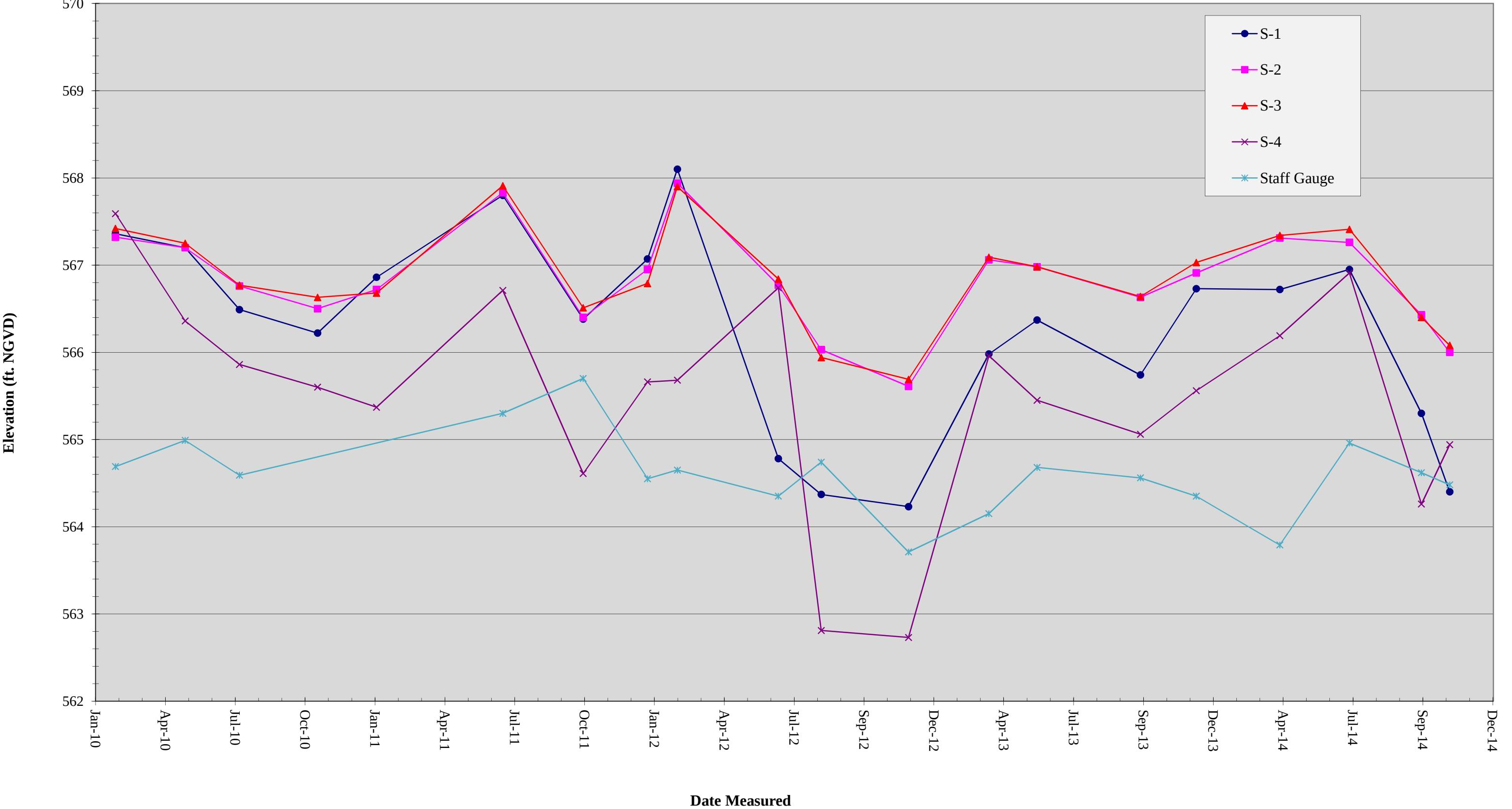
Figure 3.4a - Sump Hydrograph (2010-2014) for S-1, S-2, S-3, S-4, and Staff Gauge CHERRY FARM / RIVER ROAD SITE 4100 RIVER ROAD, TONAWANDA, NEW YORK (NYSDEC SITE NO. 9-15-063/9-15-031)
