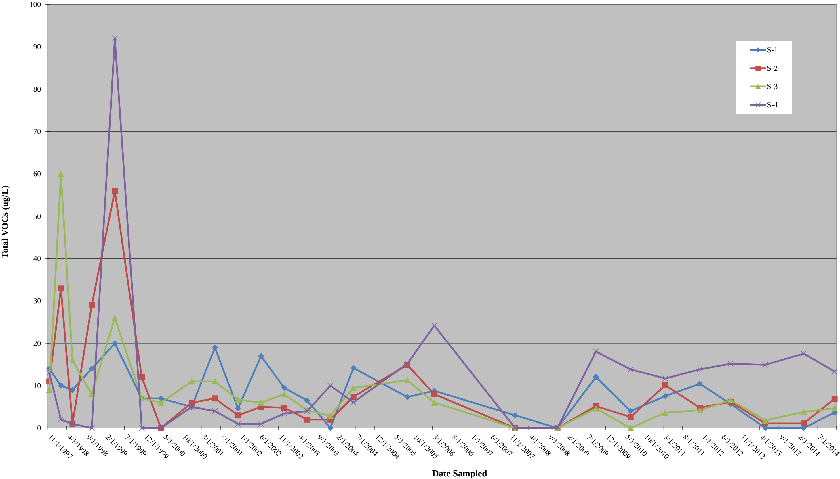
Figure 3.1d - Sump Concentration Trend Total VOCs CHERRY FARM / RIVER ROAD SITE 4100 RIVER ROAD, TONAWANDA, NEW YORK (NYSDEC SITE NO. 9-15-063/9-15-031)
