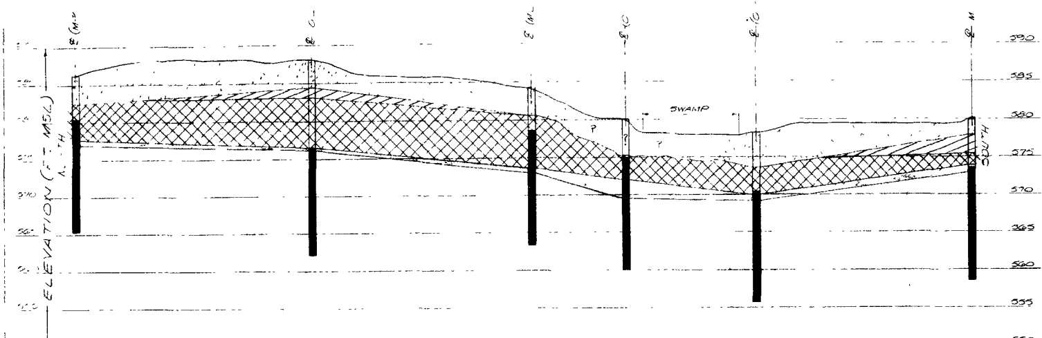
SECTION B-B SCALE: 1" = 50' HORIZ & 1" = 5' VERT
