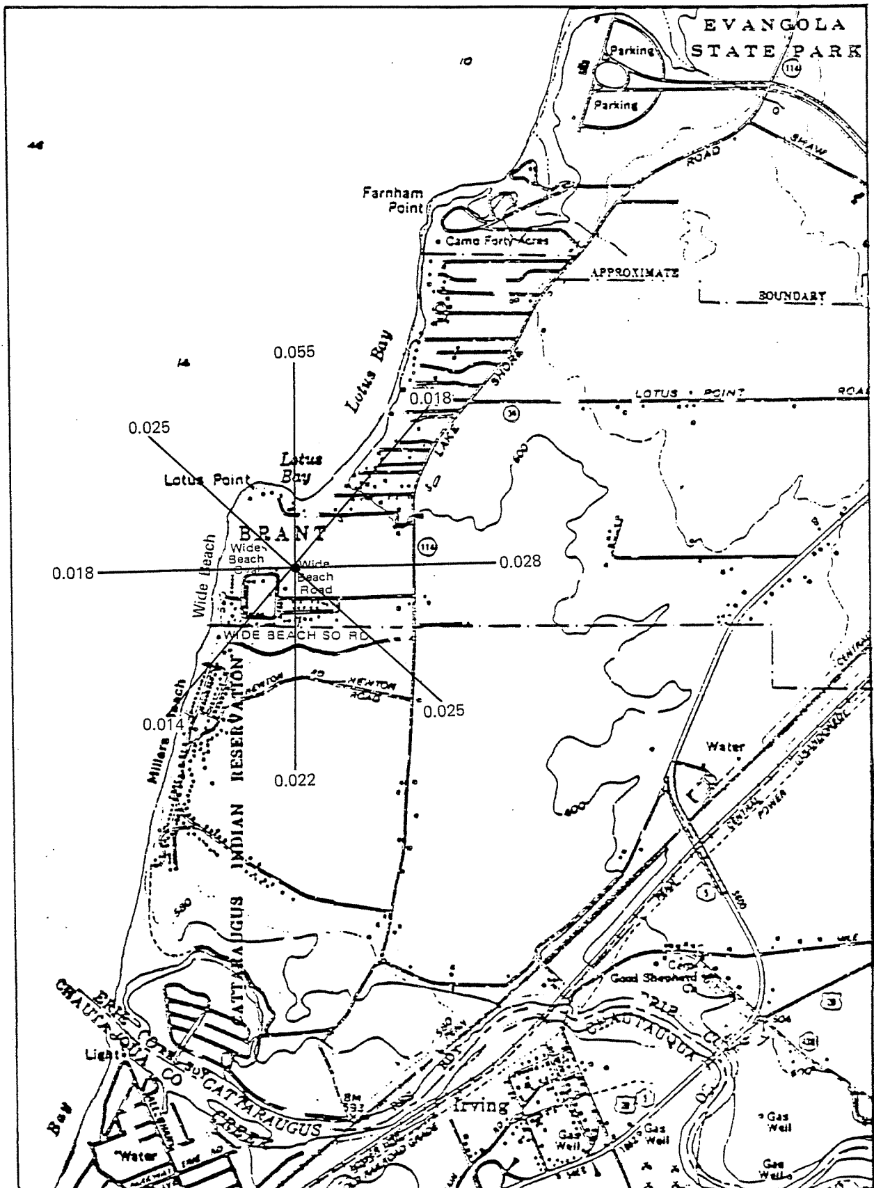
Figure 6-3. Offsite airborne transport of Aroclor 1254 (modeled concentrations in \text{mg}/\text{m}^3 ).
