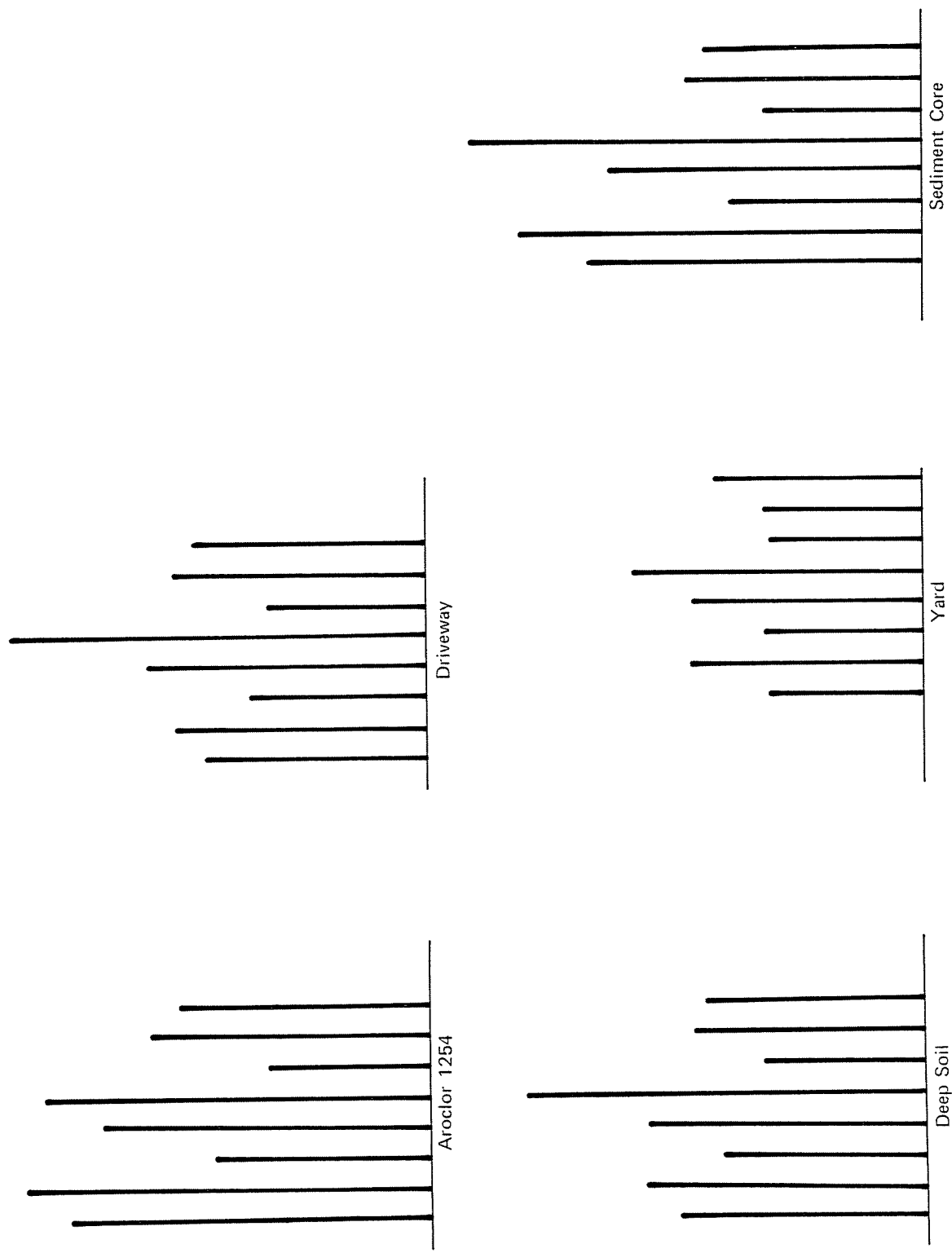
Figure 6-6. PCB profiles for SP-2250 chromatograms.
