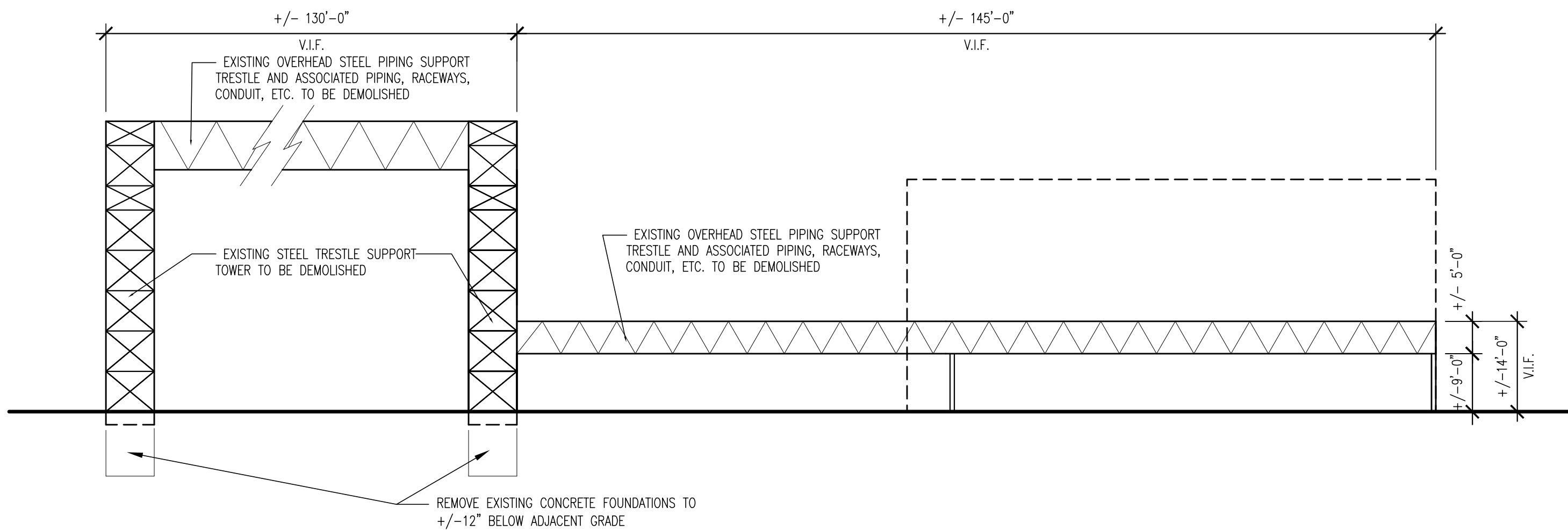
2 SOUTH EXTERIOR ELEVATION - DEMOLITION 1/16"=1'-0"
