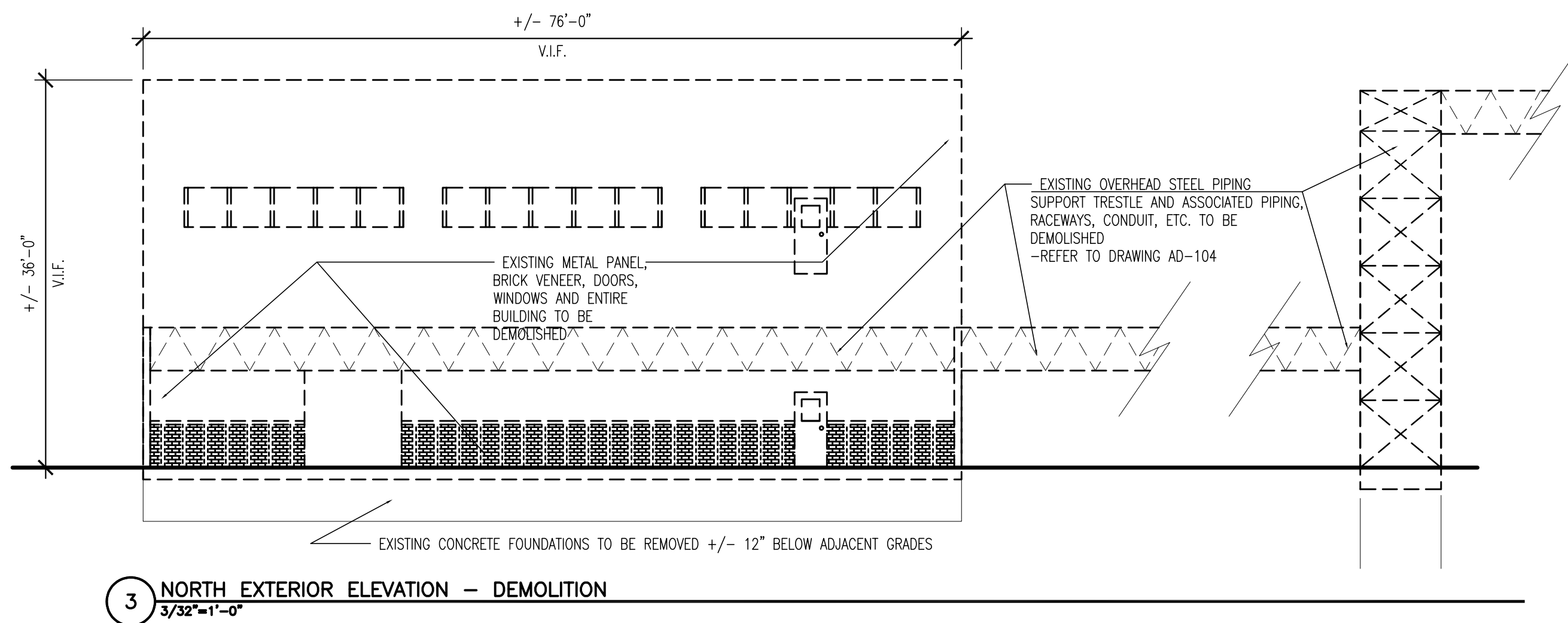
4 EAST EXTERIOR ELEVATION — DEMOLITION 3/32"=1'-0"
