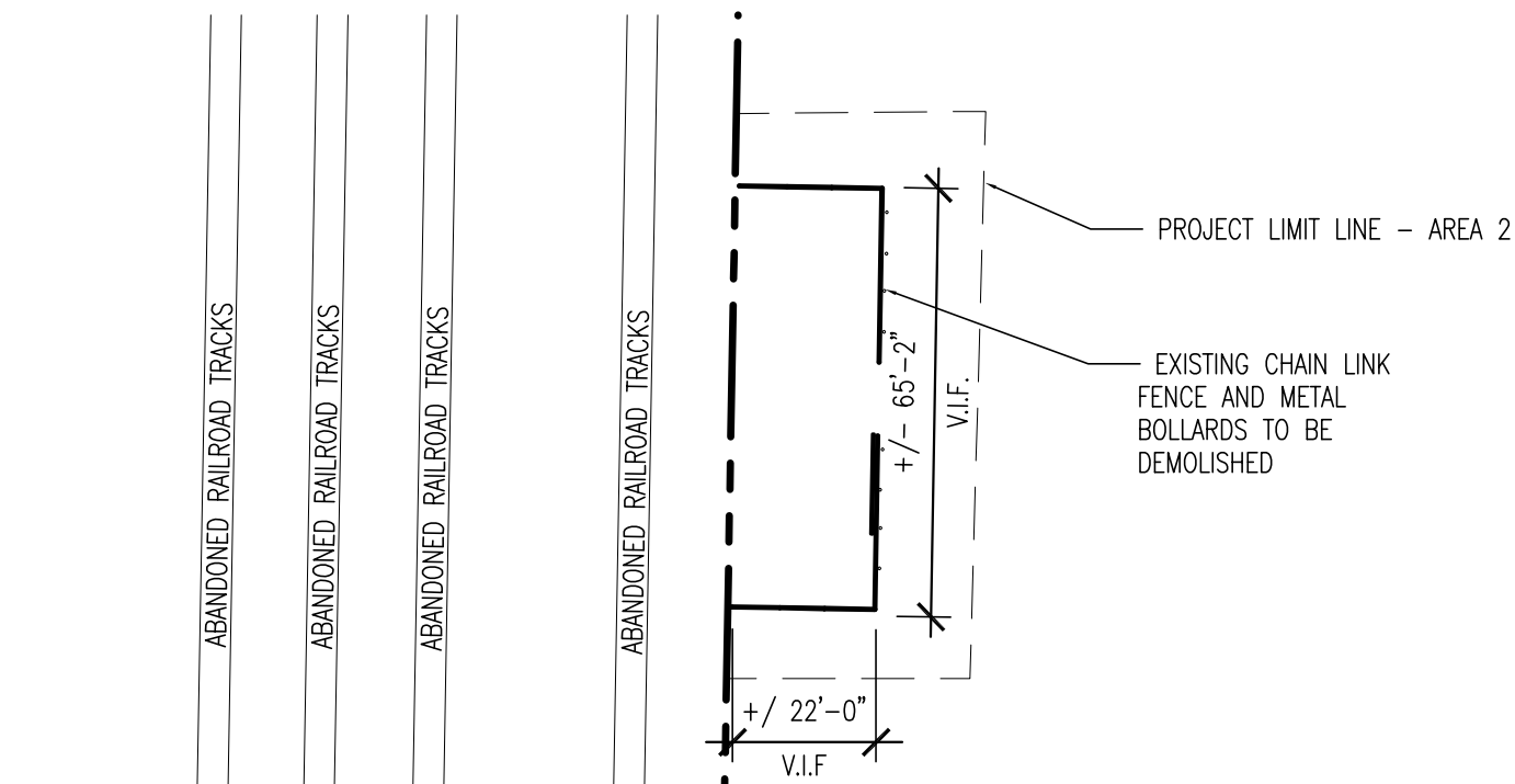
3 OVERALL DEMOLITION PLAN - AREA 2 1"=30'-0"
