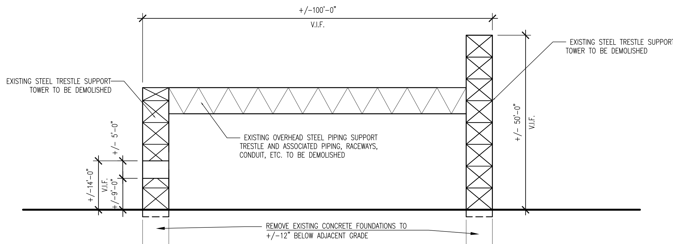
3 EAST EXTERIOR ELEVATION - DEMOLITION 1/16"=1'-0"
