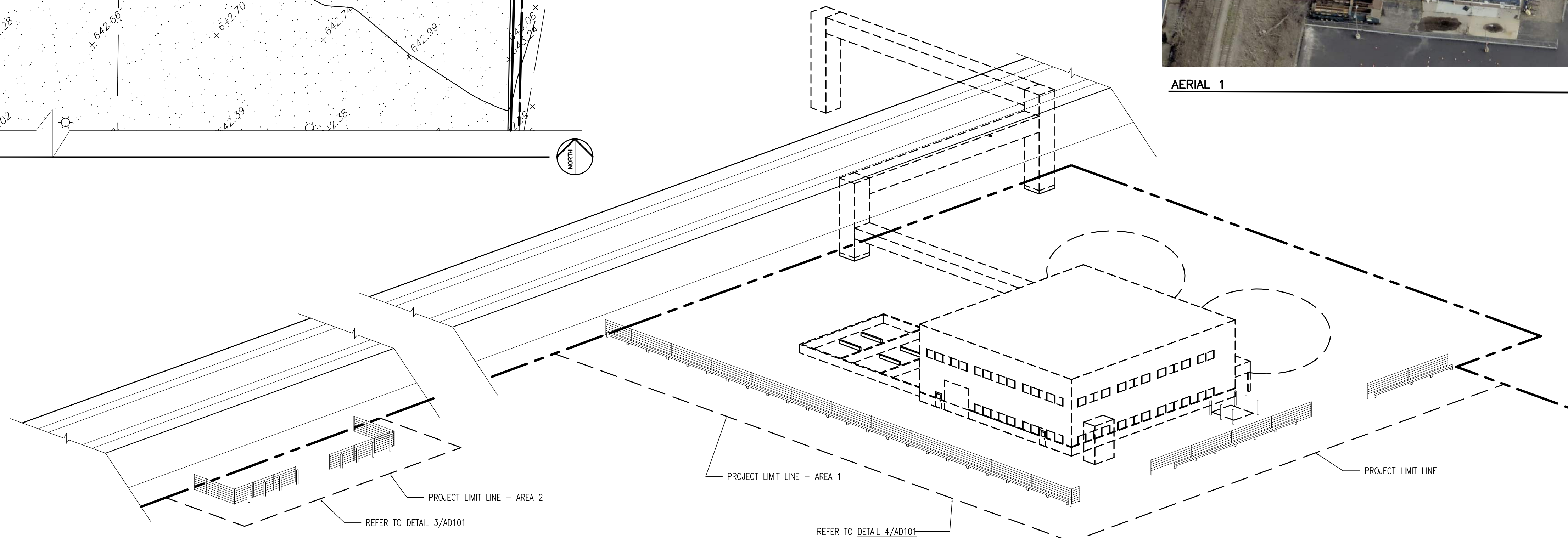
1 OVERALL AXONOMETRIC DEMOLITION PLAN 1"=30'-0"
