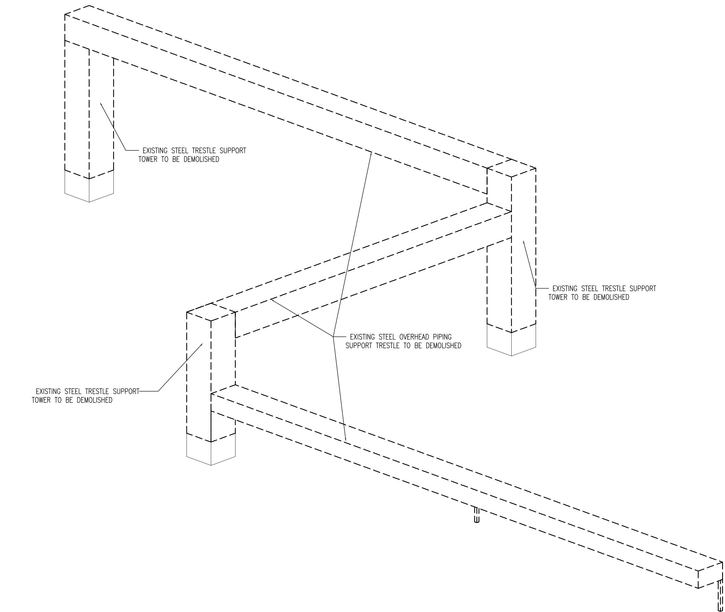
4 OVERALL TRESTLE AXONOMETRIC VIEW 1"=30'-0"
