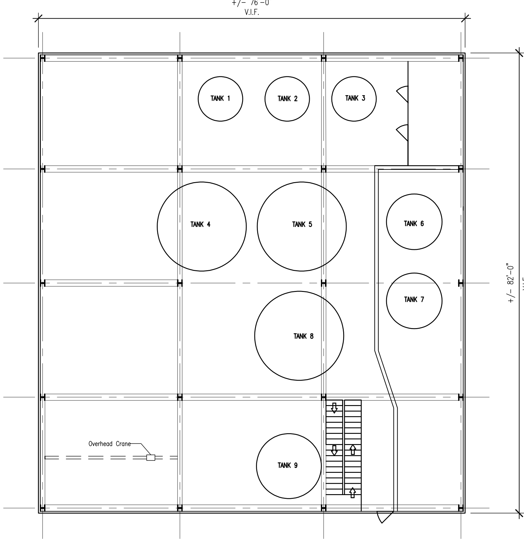
5 FLOOR/TANK PLAN — DEMOLITION 1"=30'-0"
