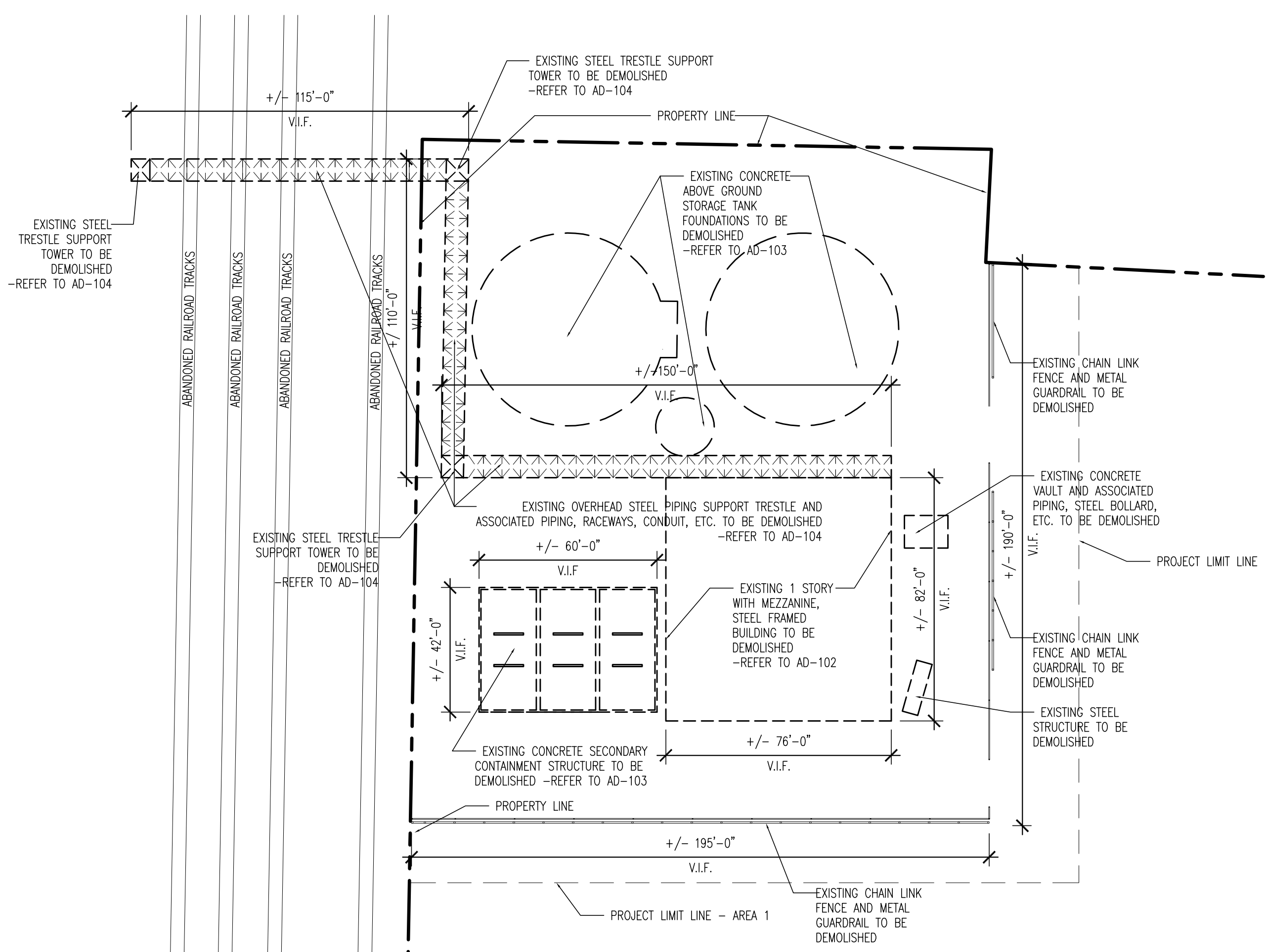
2 OVERALL DEMOLITION PLAN - AREA 1 1"=30'-0"
