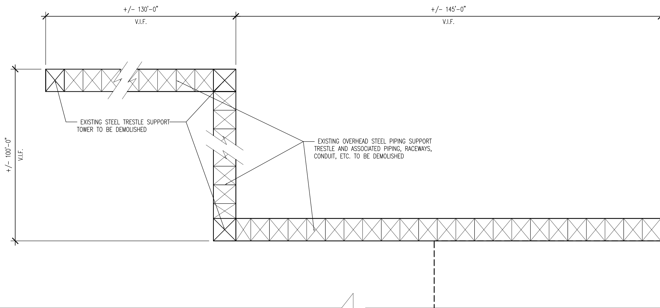
1 OVERALL TRESTLE PLAN 1/16"=1'-0"
