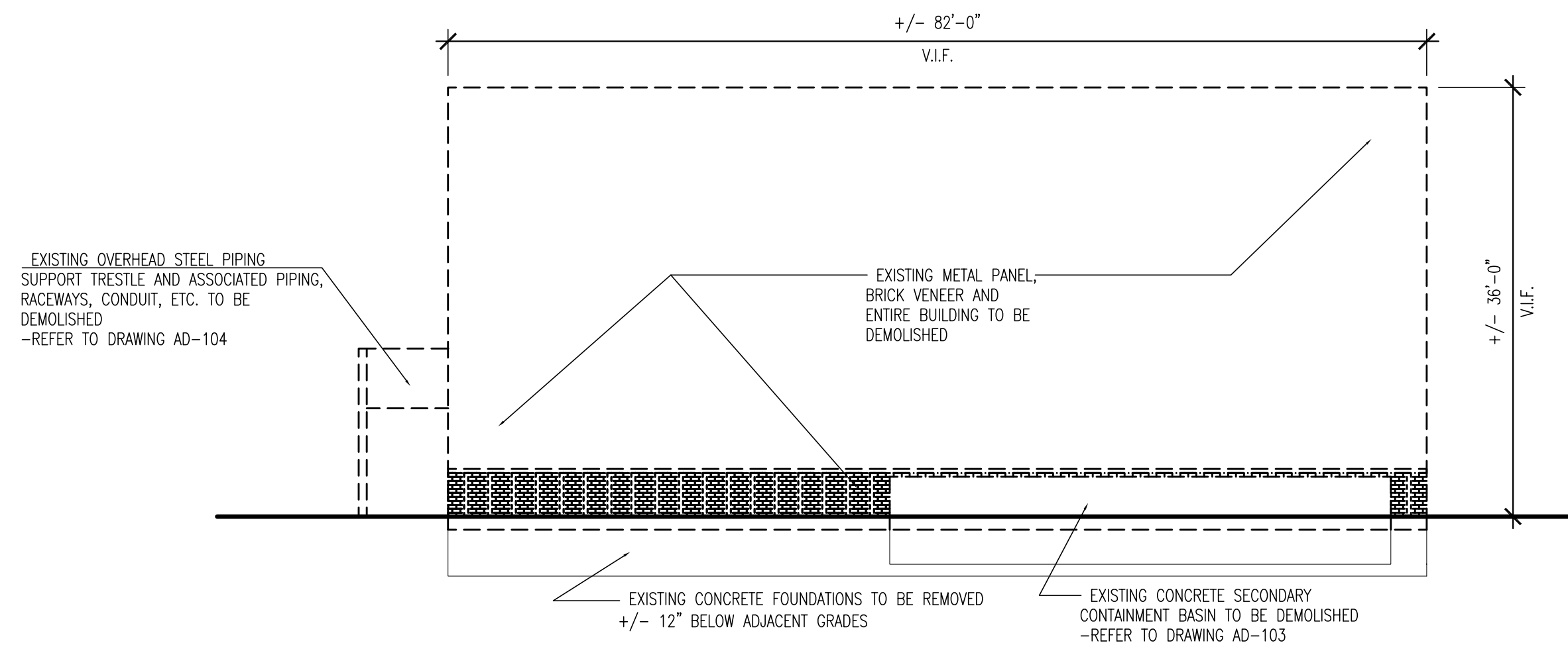
2 WEST EXTERIOR ELEVATION — DEMOLITION 3/32"=1'-0"
