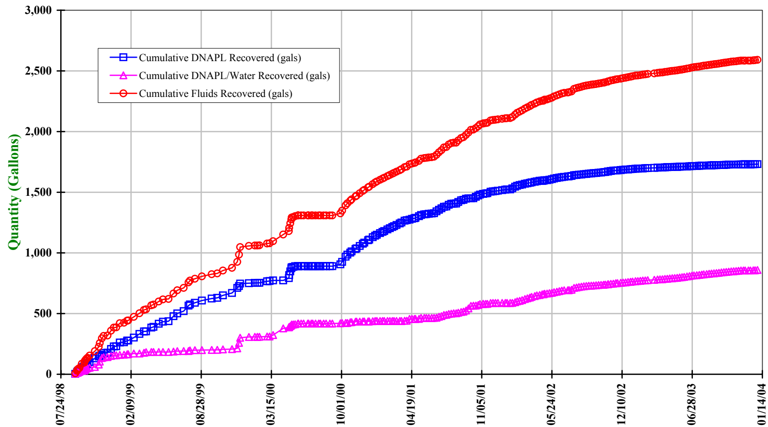
Figure 3-2. DNAPL and DNAPL/Water Recovery - Cumulative Totals Former Gastown Manufactured Gas Plant Site
