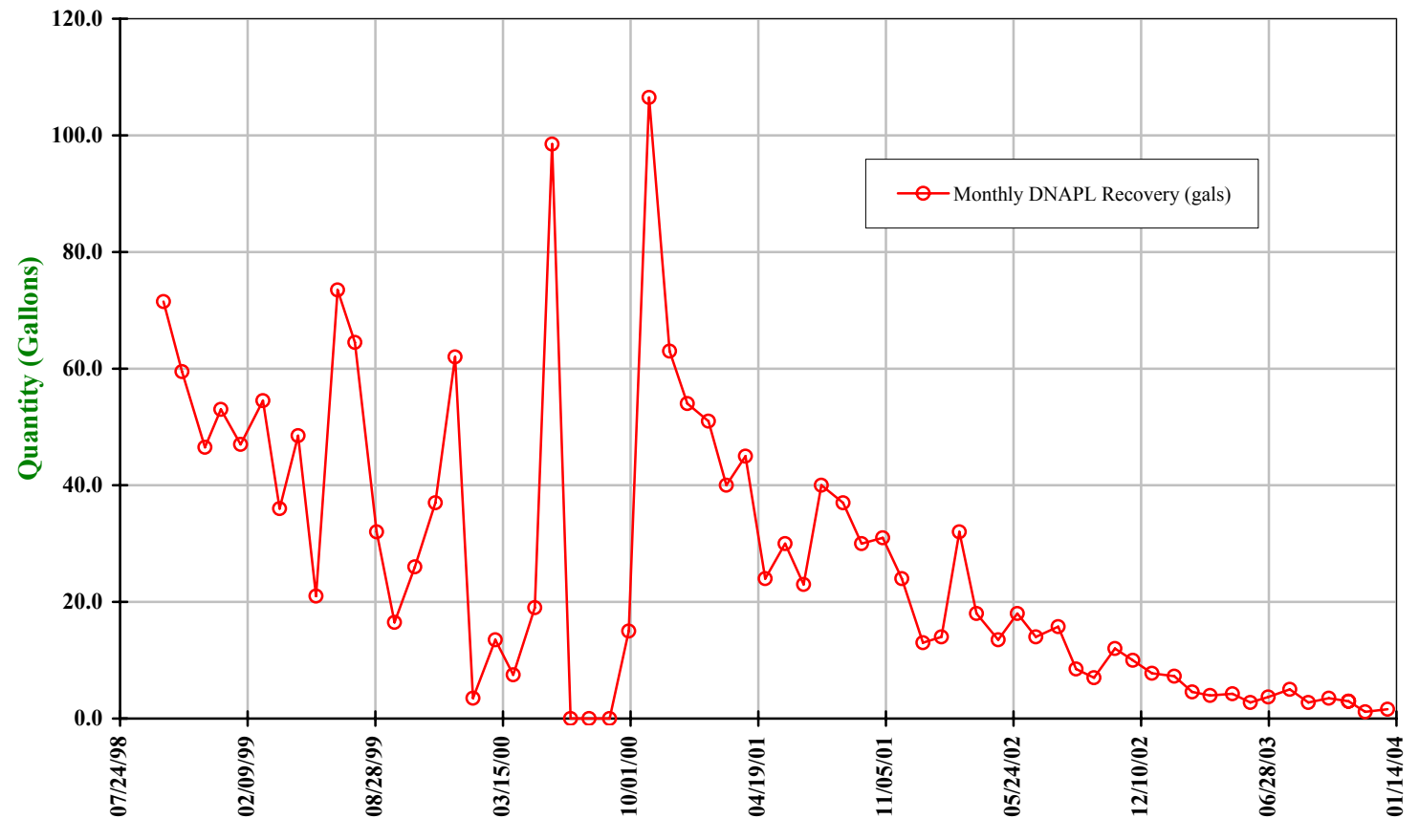
Figure 4-2. Monthly DNAPL Recovery Former Gastown Manufactured Gas Plant Site
