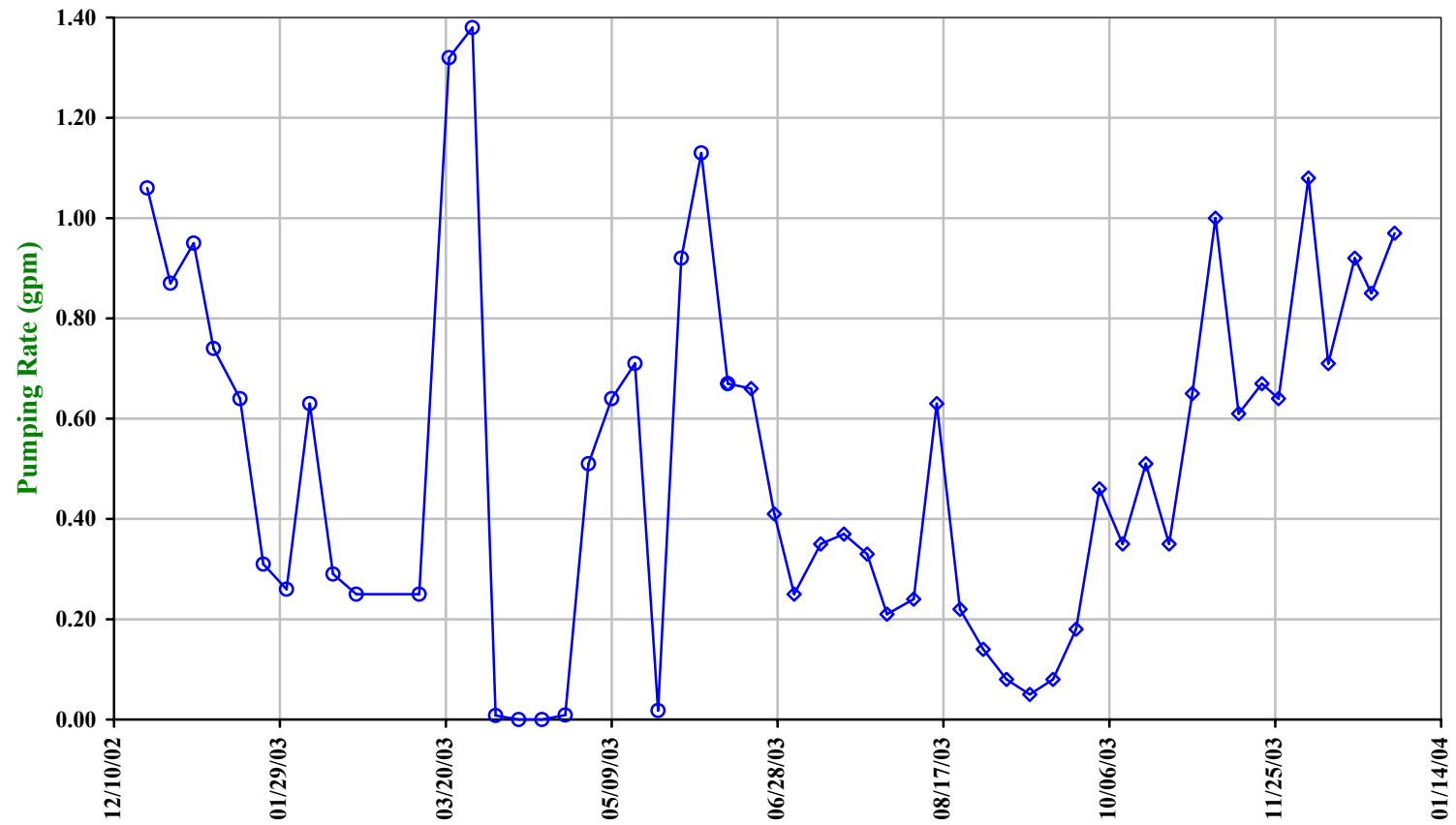
Figure 3-1. Groundwater Pumping Rates for 2003 Former Gastown Manufactured Gas Plant Site
