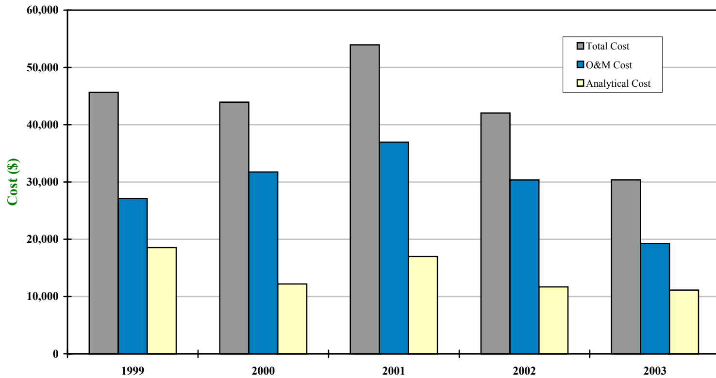
Figure 4-6. Annual O&M Costs for the Groundwater/NAPL Extraction and Treatment System Former Gastown Manufactured Gas Plant Site
