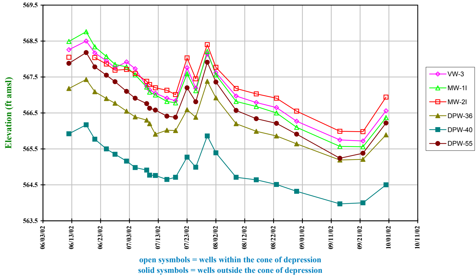
Figure 4-4. Hydrographs from Selected Wells Former Gastown Manufactured Gas Plant Site
