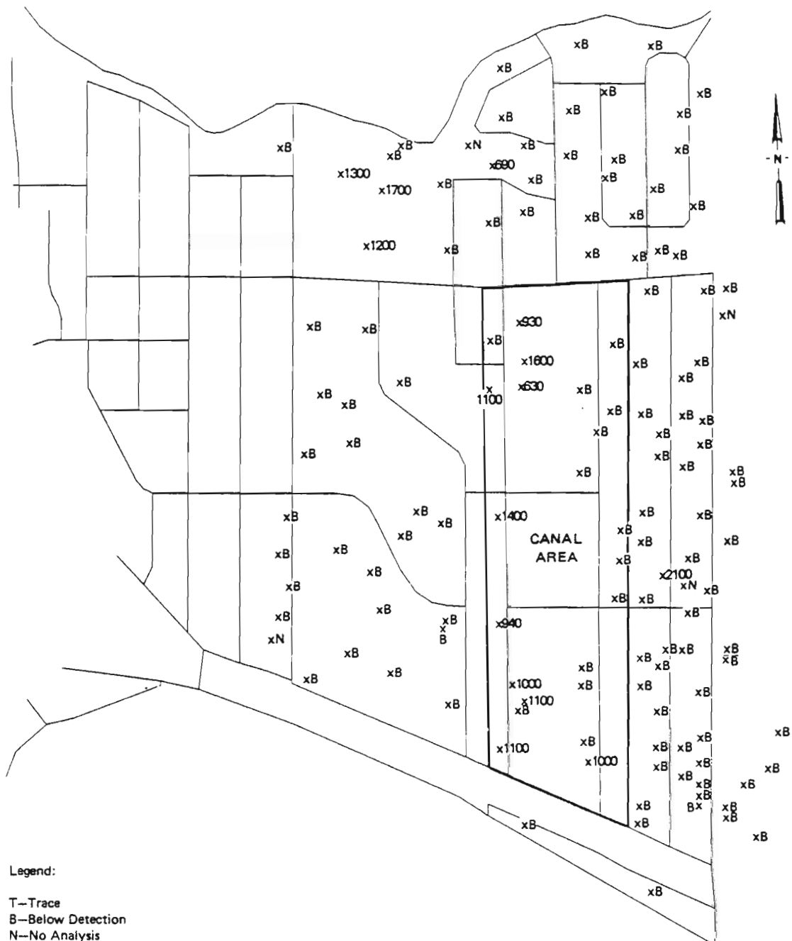
Figure 31. Soil Sampling Sites, Cadmium, Maximum Concentrations (micrograms per kilogram ppb).
