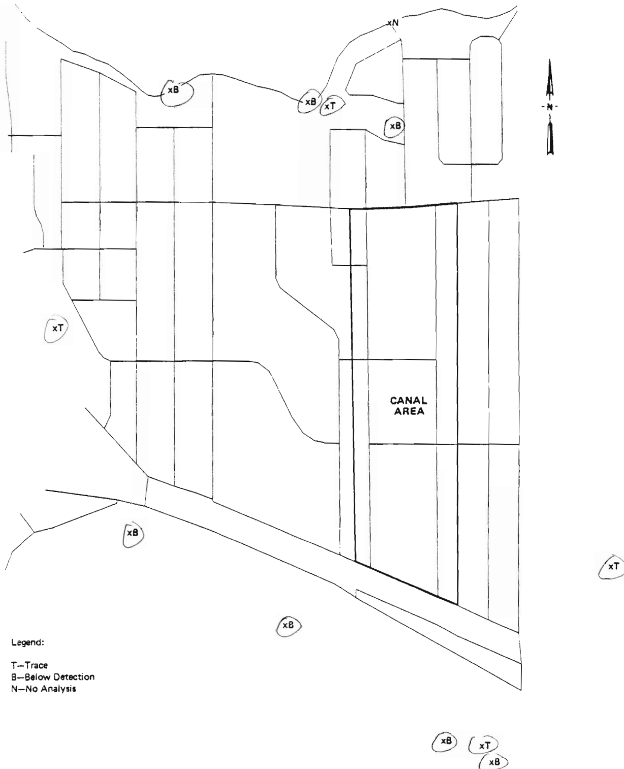
Figure 46. Surface Water Sampling Sites, γ-BHC, Maximum Concentrations (micrograms per liter, ppb).
