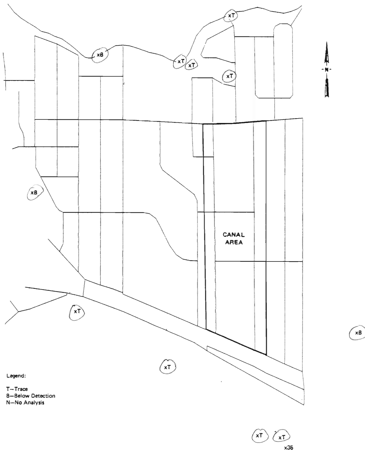
Figure 44. Surface Water Sampling Sites, Toluene, Maximum Concentrations (micrograms per liter, ppb).
