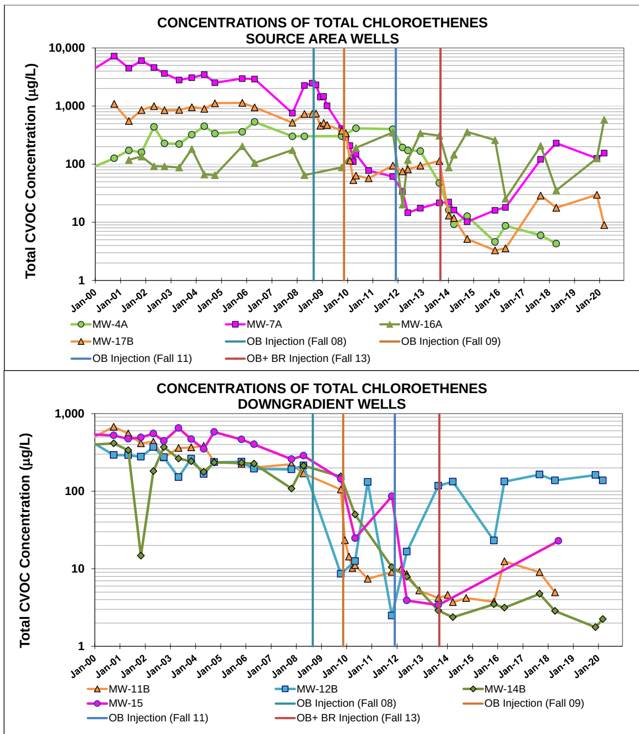
FIGURE 15 FORMER CARBORUNDUM COMPANY LONG TERM TRENDS OF TOTAL CHLORINATED ETHENES IN SOURCE AREA AND DOWNGRADIANT WELLS AECOM 257 West Genesee Street, Buffalo, NY 14202
