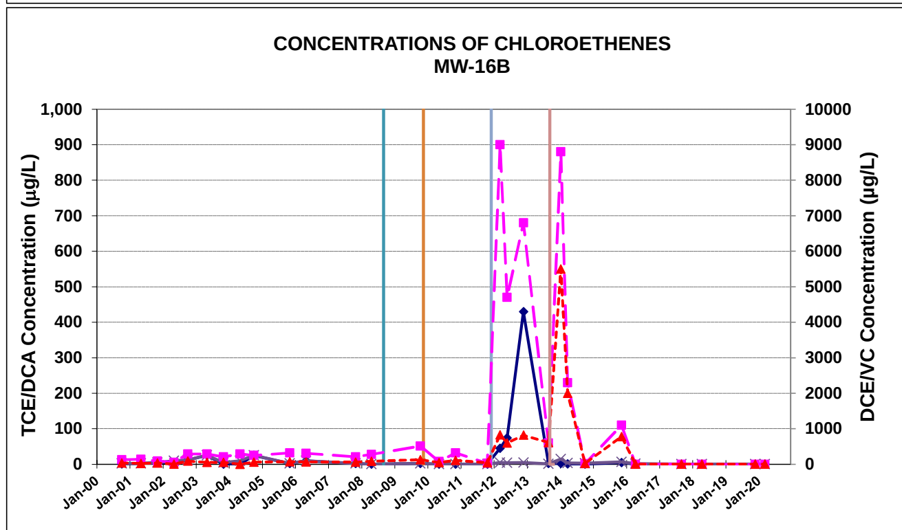
FIGURE 22 FORMER CARBORUNDUM COMPANY LONG TERM TRENDS OF CHLORINATED ETHENES IN WELLS MW-16A AND MW-16B AECOM 257 West Genesee Street, Buffalo, NY 14202
