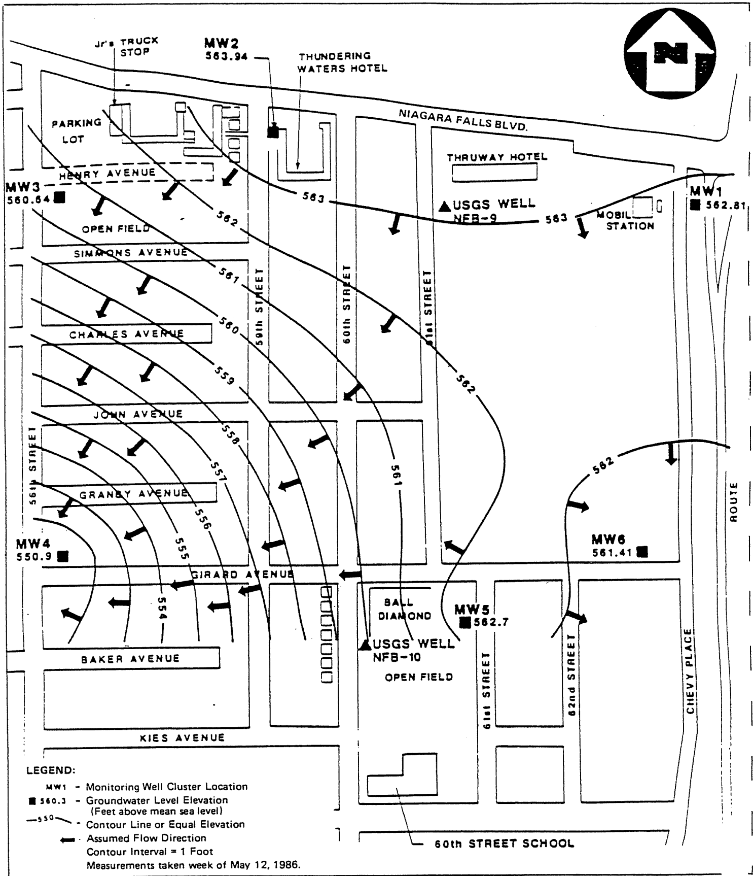
Figure 4-5 POTENTIOMETRIC SURFACE CONTOUR MAP FOR UPPER FRACTURE ZONE WELLS
