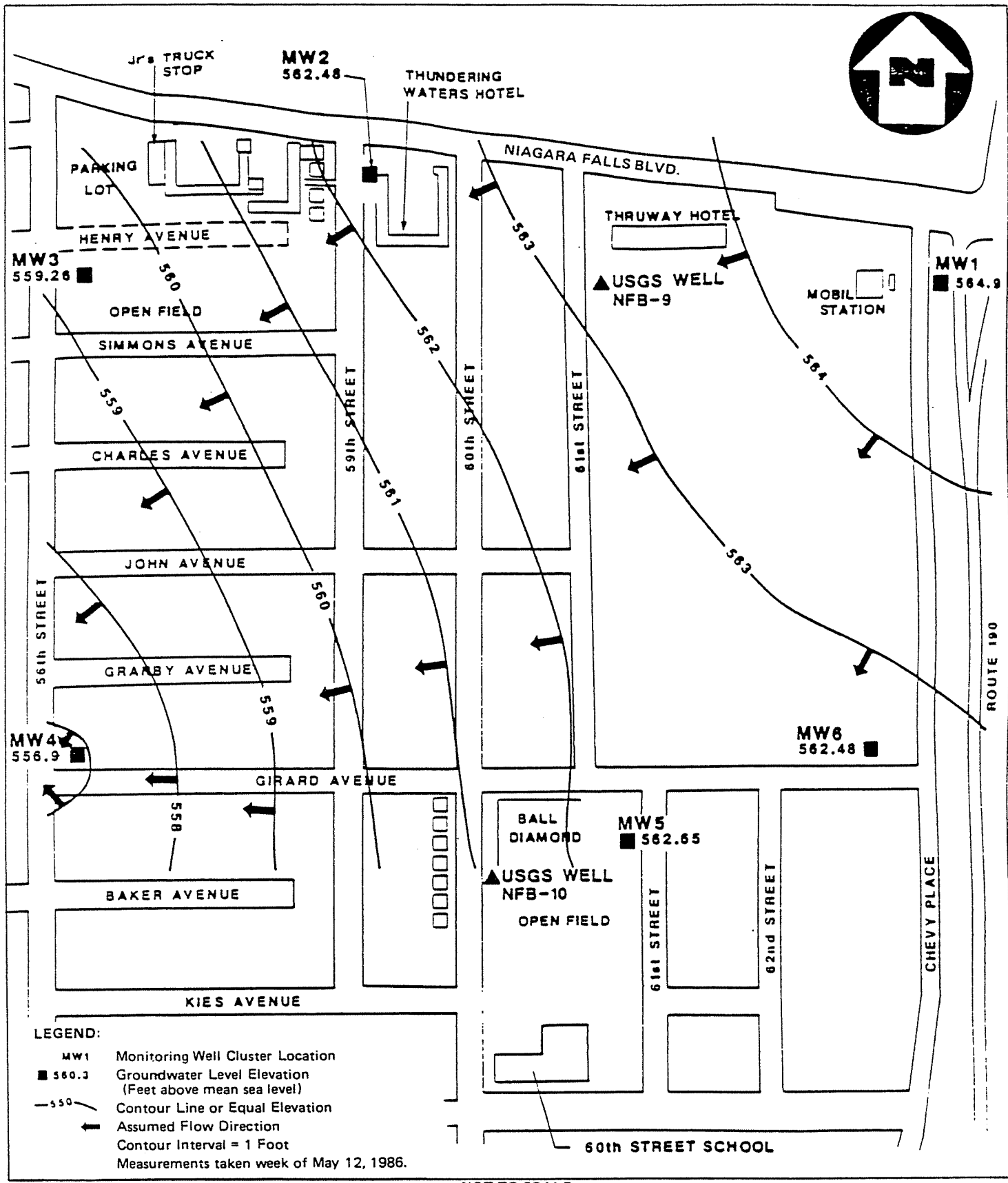
Figure 4-6 POTENTIOMETRIC SURFACE CONTOUR MAP FOR LOWER FRACTURE ZONE WELLS
