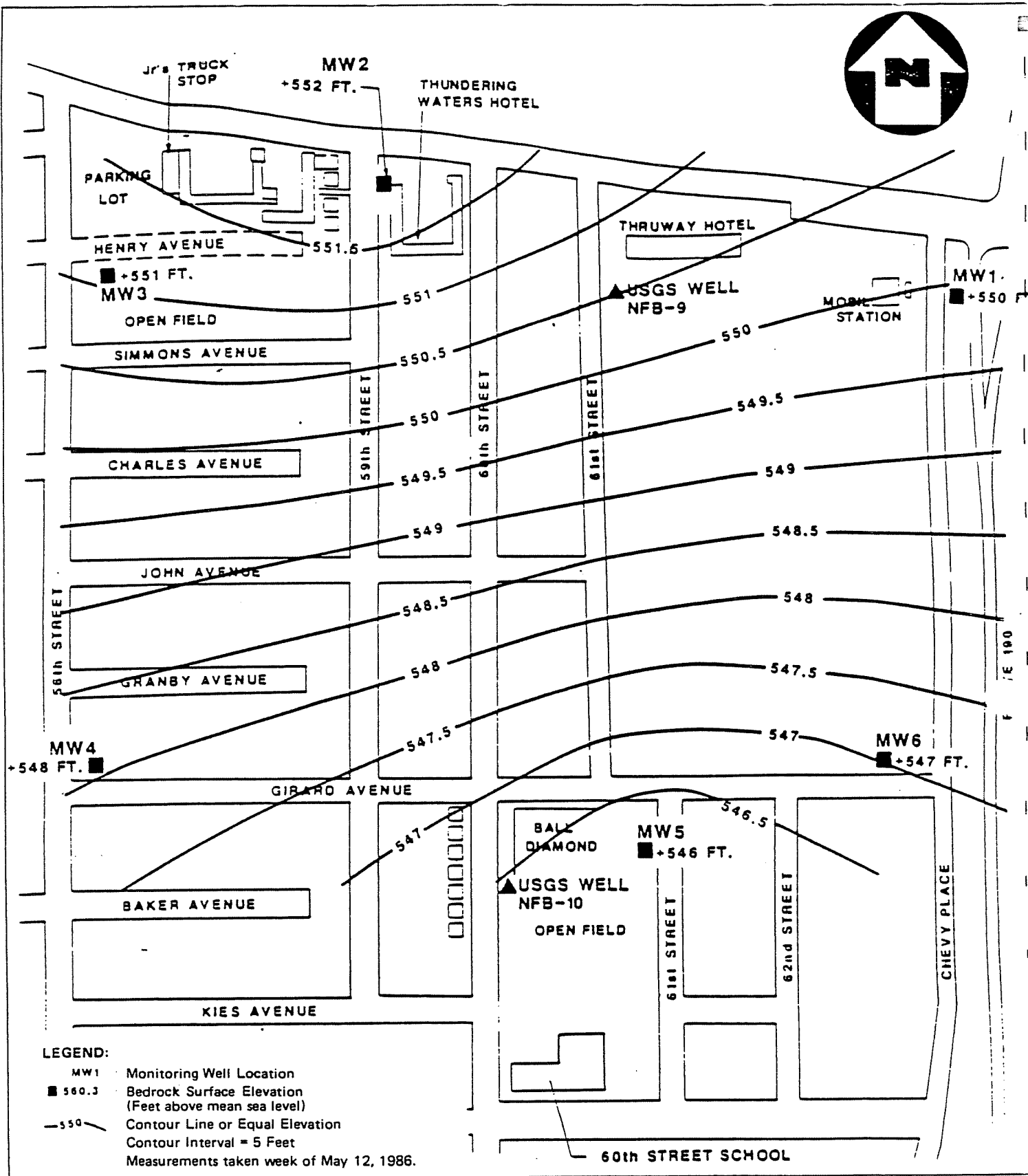
Figure 4-1 TOP OF BEDROCK CONTOUR MAP
