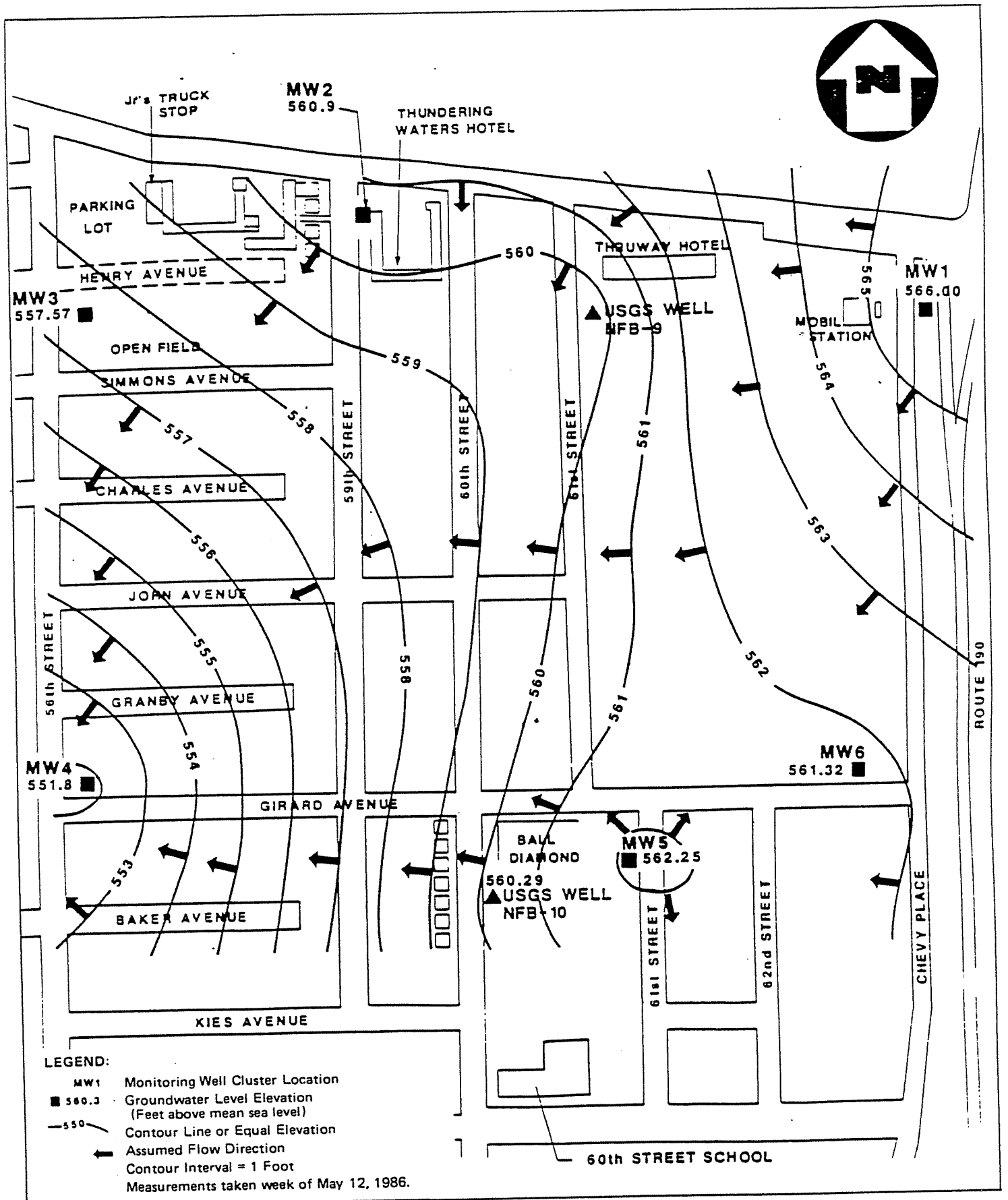
Figure 4-4 POTENTIOMETRIC SURFACE CONTOUR MAP FOR REGOLITH WELLS
