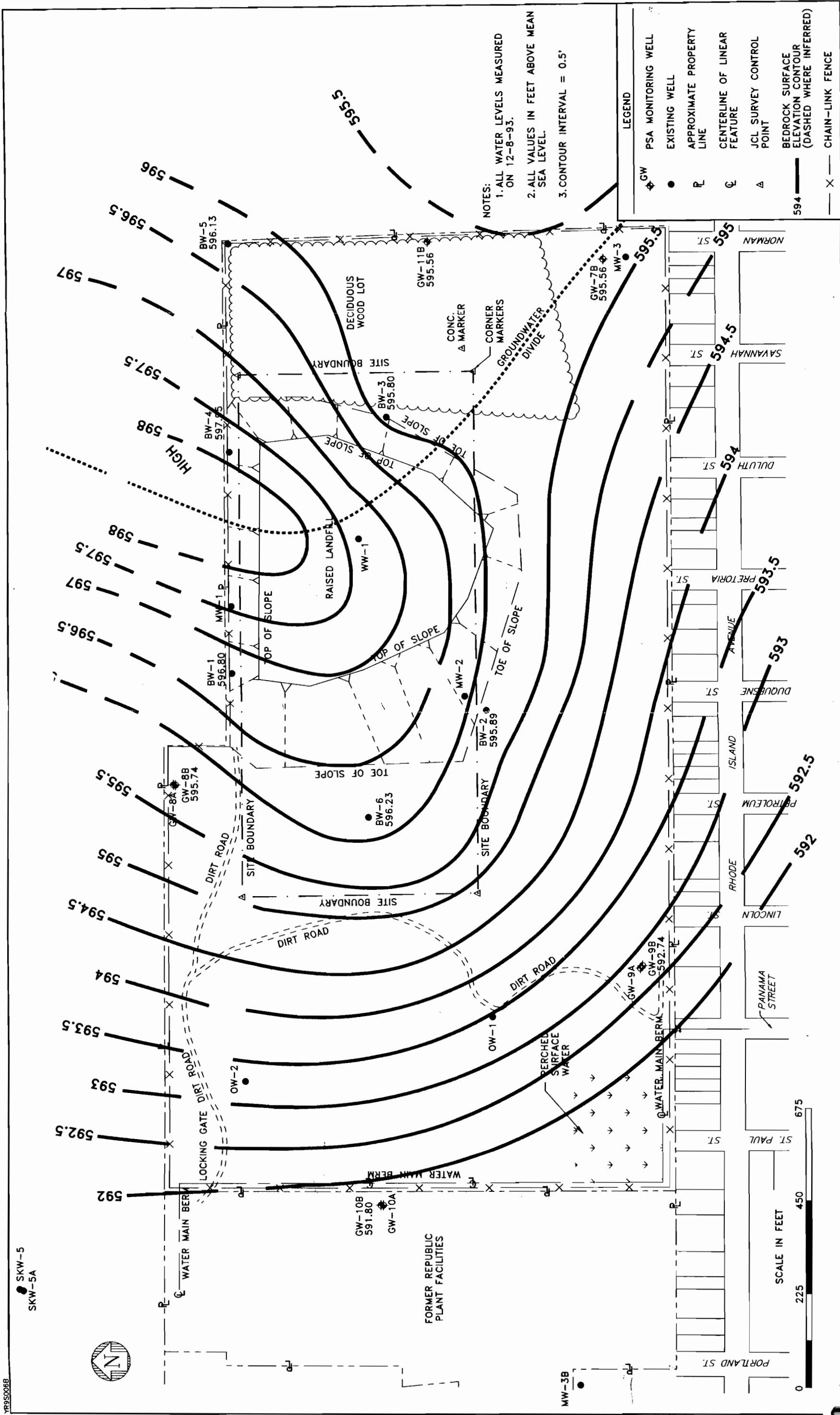
Figure 3-10 BEDROCK AQUIFER POTENTIOMETRIC SURFACE MAP UNION CARBIDE SITE
