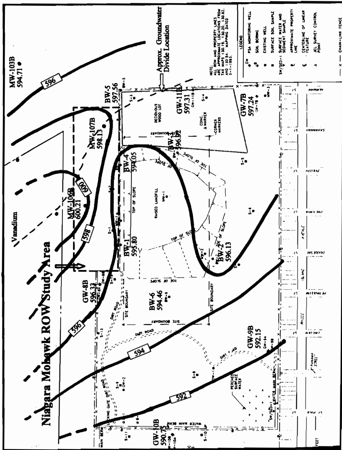
Figure 8 - Bedrock Groundwater Contours
