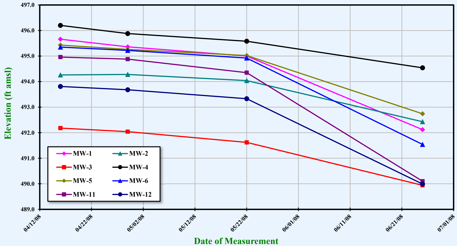
Figure 2-10. 2008 Overburden micro-well hydrographs for the Former Barker Chemical Site. Well locations are shown on Figure 2-8.
