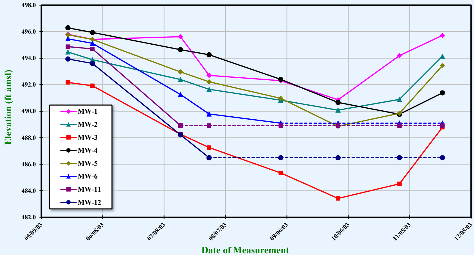
Figure 2-9. 2003 Overburden micro-well hydrographs for the Former Barker Chemical Site. Lines are dashed where the wells are dry. Well locations are shown on Figure 2-8.
