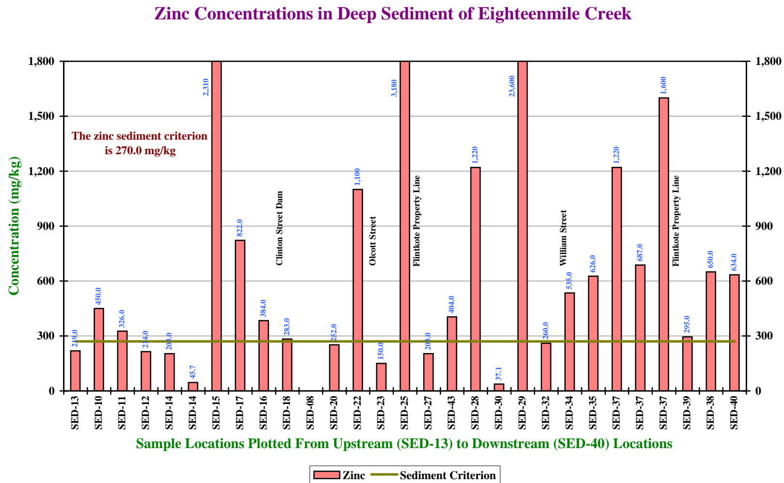
Figure 6-12. Zinc concentrations in deep sediment of Eighteenmile Creek from the New York State Barge Canal (SED-13) to Harwood Street (SED-40). A scale was selected that best presents the data at lower concentrations. The blanks indicate that the sample was not analyzed for zinc.
