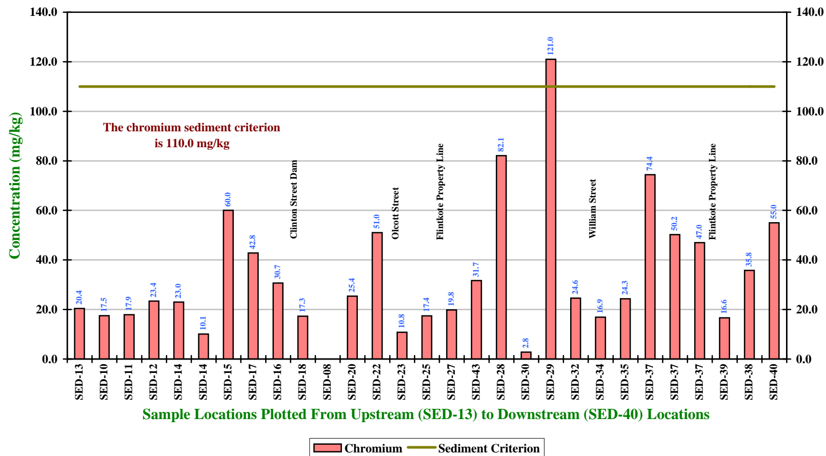
Figure 6-6. Chromium concentrations in deep sediment of Eighteenmile Creek from the New York State Barge Canal (SED-13) to Harwood Street (SED-40). The blanks indicate that the sample was not analyzed for chromium.
