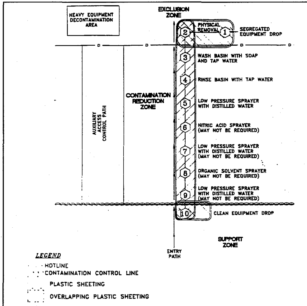
Figure 2. Decontamination Layout
