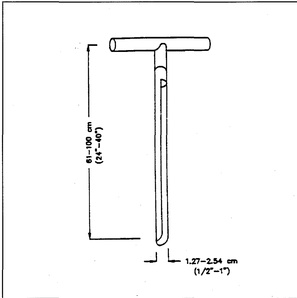
FIGURE 2. Sampling Trier
