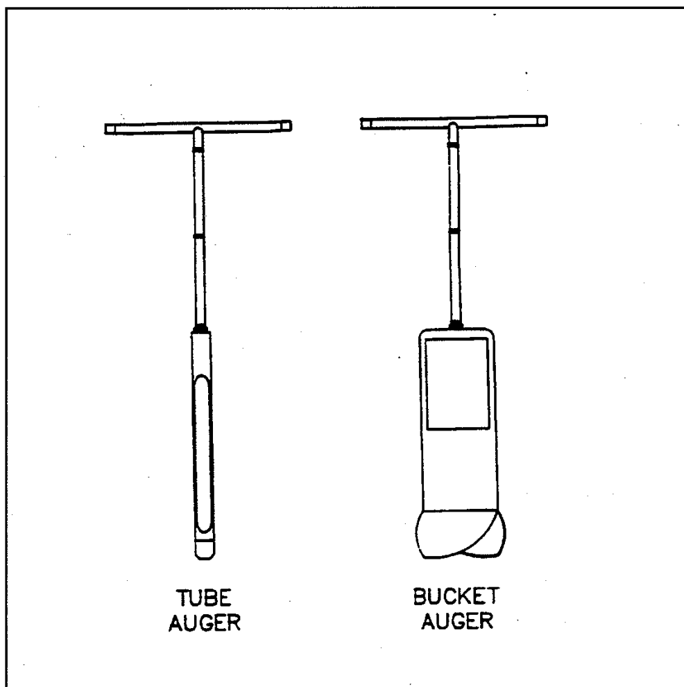
FIGURE 1. Sampling Augers
