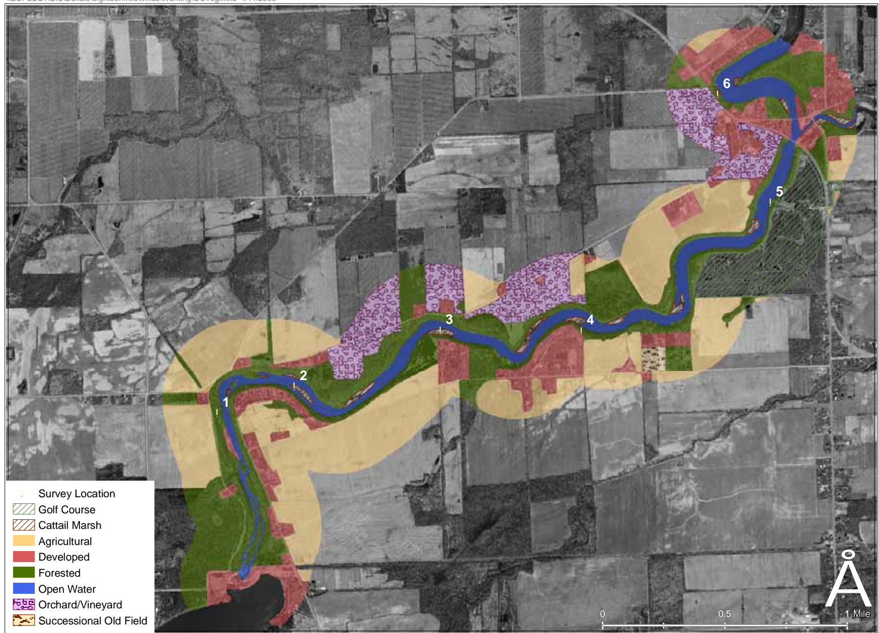
Figure 2-4 Wildlife Survey Locations and Surrounding CoverTypes - Oak Orchard Creek
