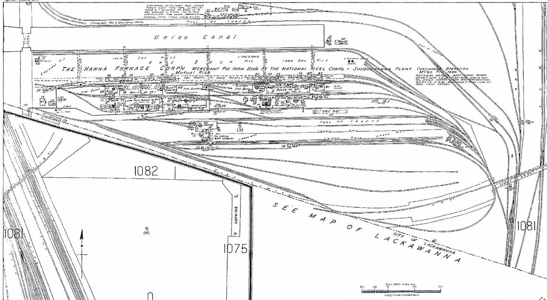
Figure 2 HANNA FURNACE CORPORATION PLANT, BUFFALO, NEW YORK, CIRCA 1940
