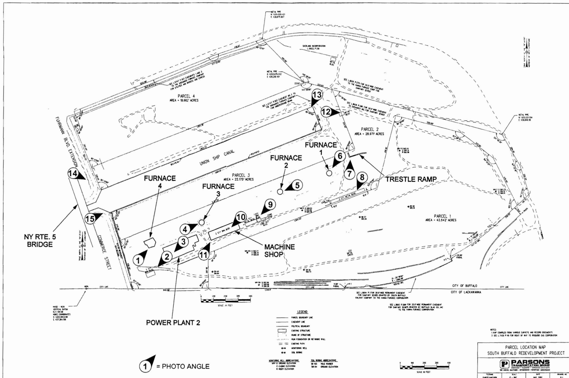
Site plan with photo angles. Hanna Furnace Redevelopment Project, Buffalo, Erie County, New York.
