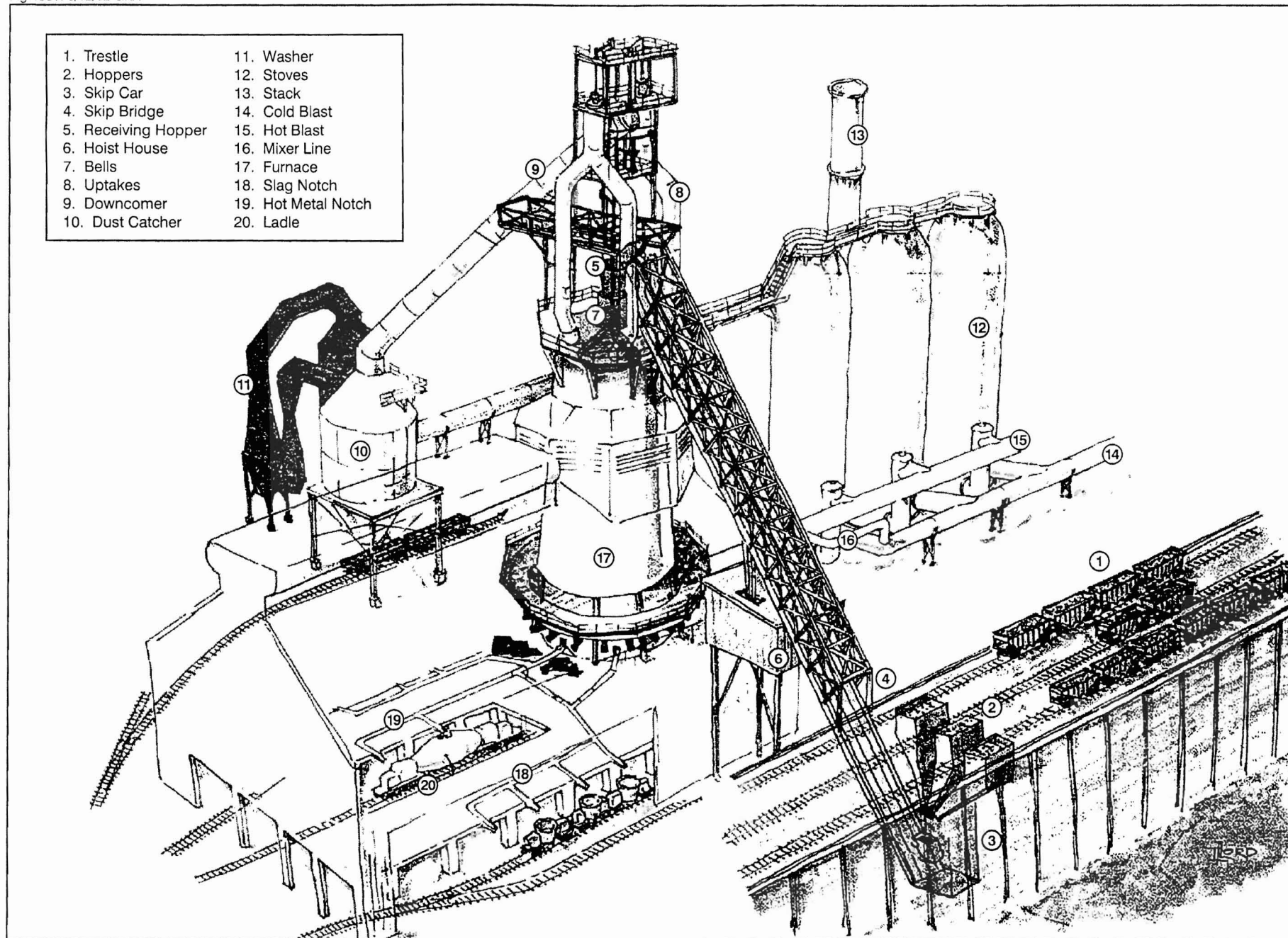
Figure 5 SCHEMATIC REPRESENTATION OF A BLAST FURNACE PLANT
