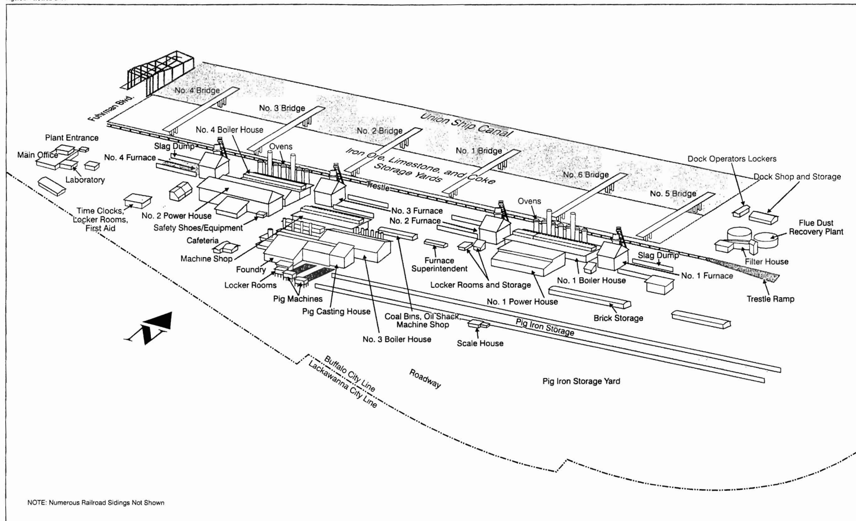
Figure 3 SCHEMATIC REPRESENTATION OF THE HANNA FURNACE CORPORATION PLANT, BUFFALO, NEW YORK, CIRCA 1941-1960
