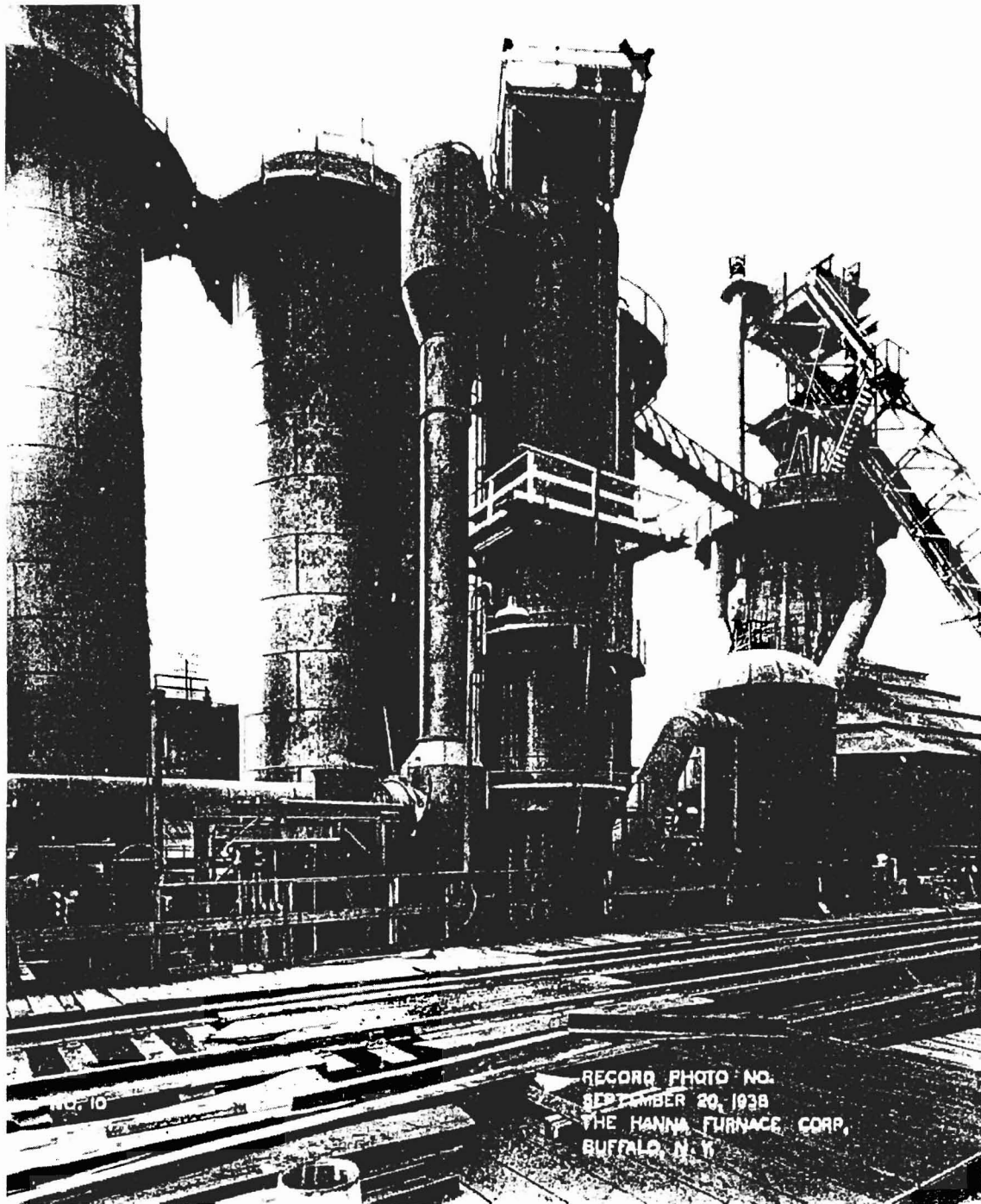
No. 1 Furnace with skip bridge, downcomer, dust catcher, washer and three stoves. Elevated trestle with a rail line in the foreground.
