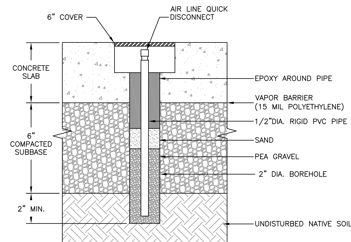
2 SOIL VAPOR MONITORING POINT DETAIL
