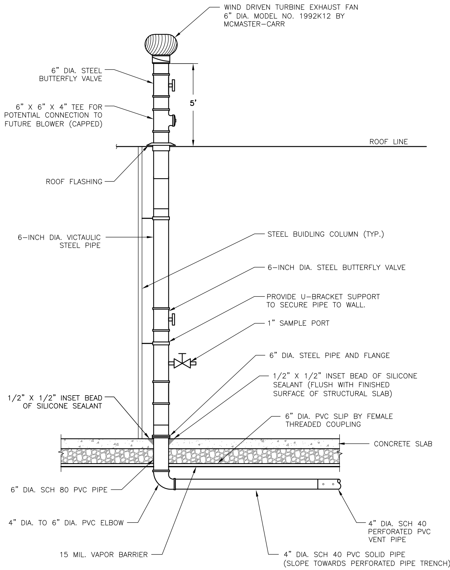
2 VERTICAL RISER DETAIL
