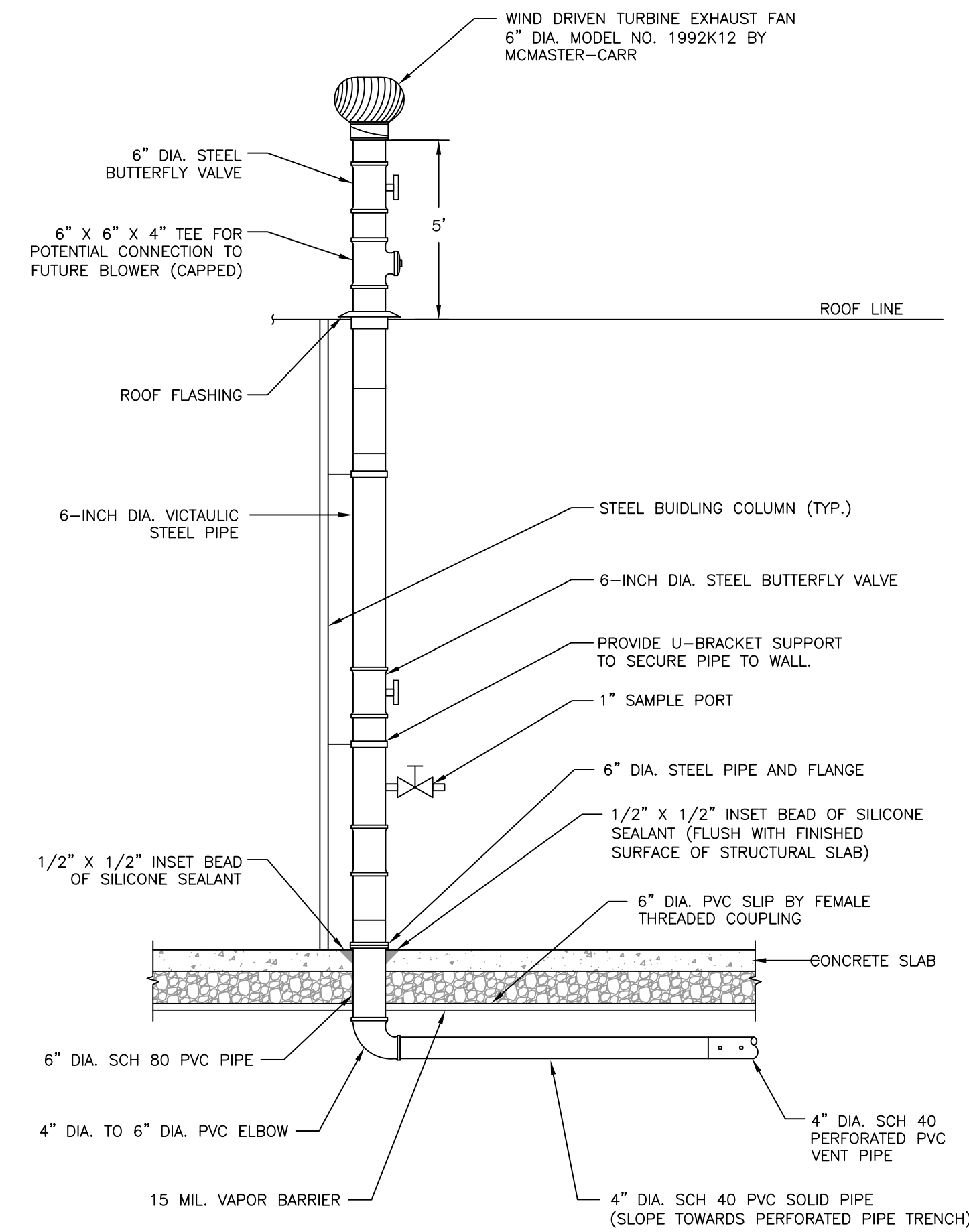
1 RISER DETAIL
