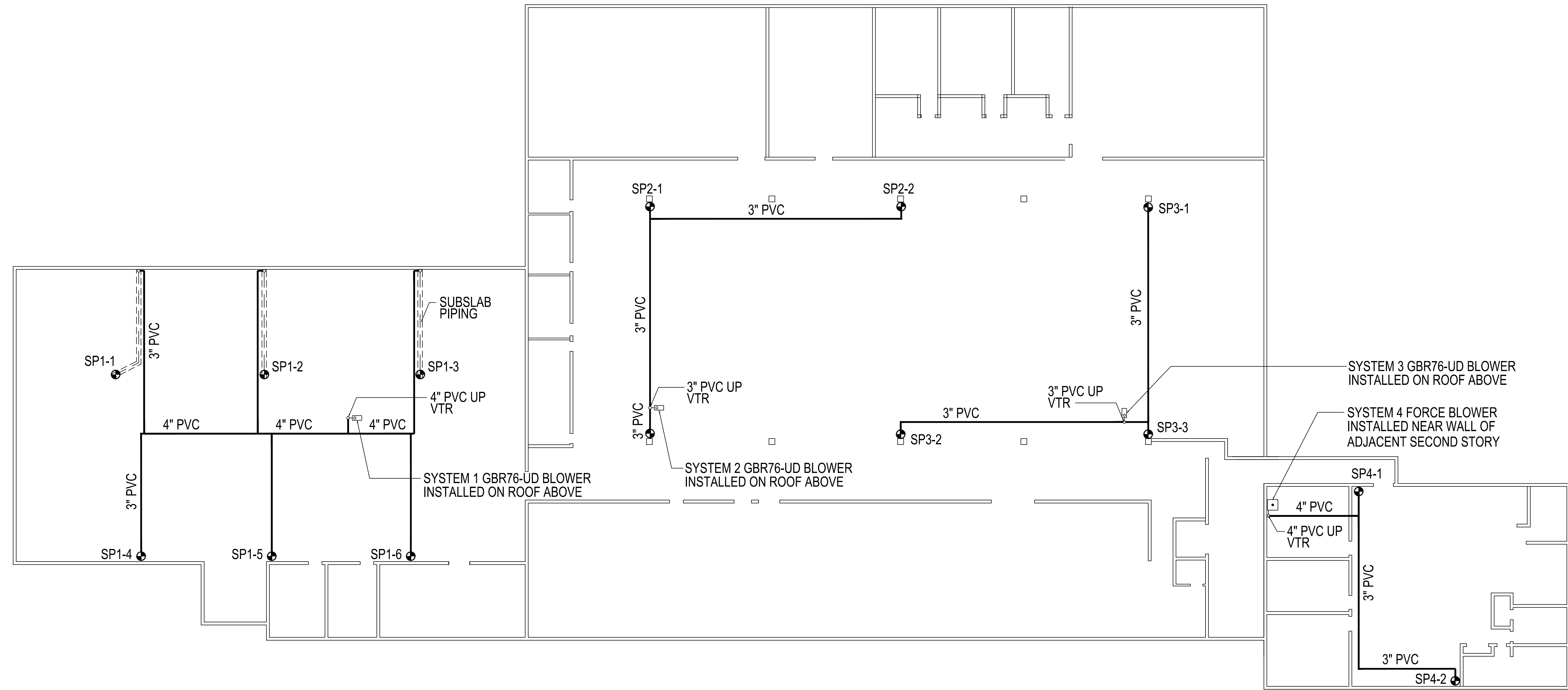
FLOOR PLAN
