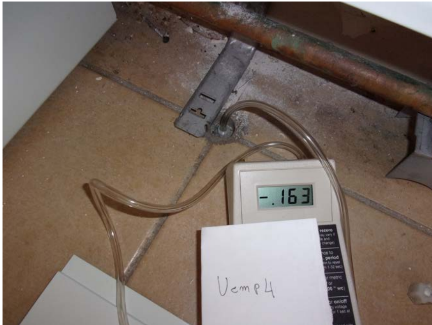
3. View of VEMP-4 in June 2016.
