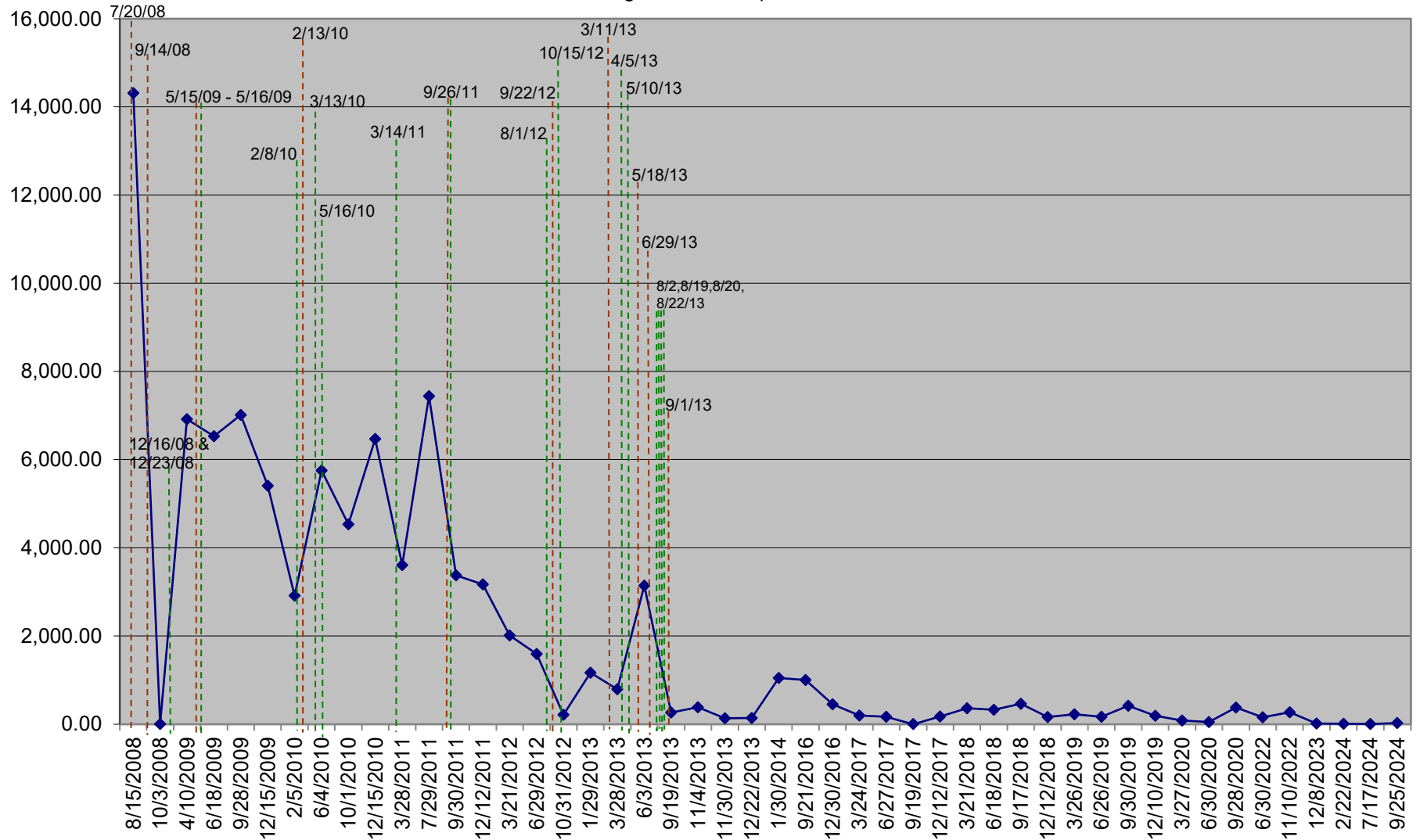
Graph 1 IRMW-7 Total Petroleum VOCs 3035 White Plains Road, Bronx, NY August 2008 - September 2024
