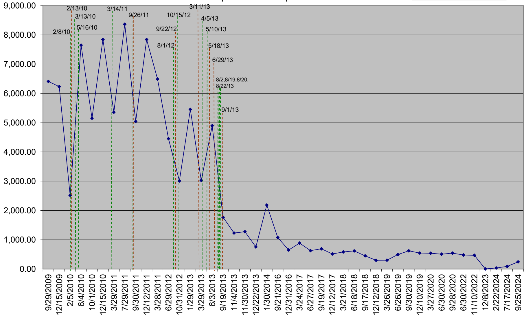
Graph 2 IRMW-10 Total Petroleum VOCs 3035 White Plains Road, Bronx, NY September 2009 - September 2024
