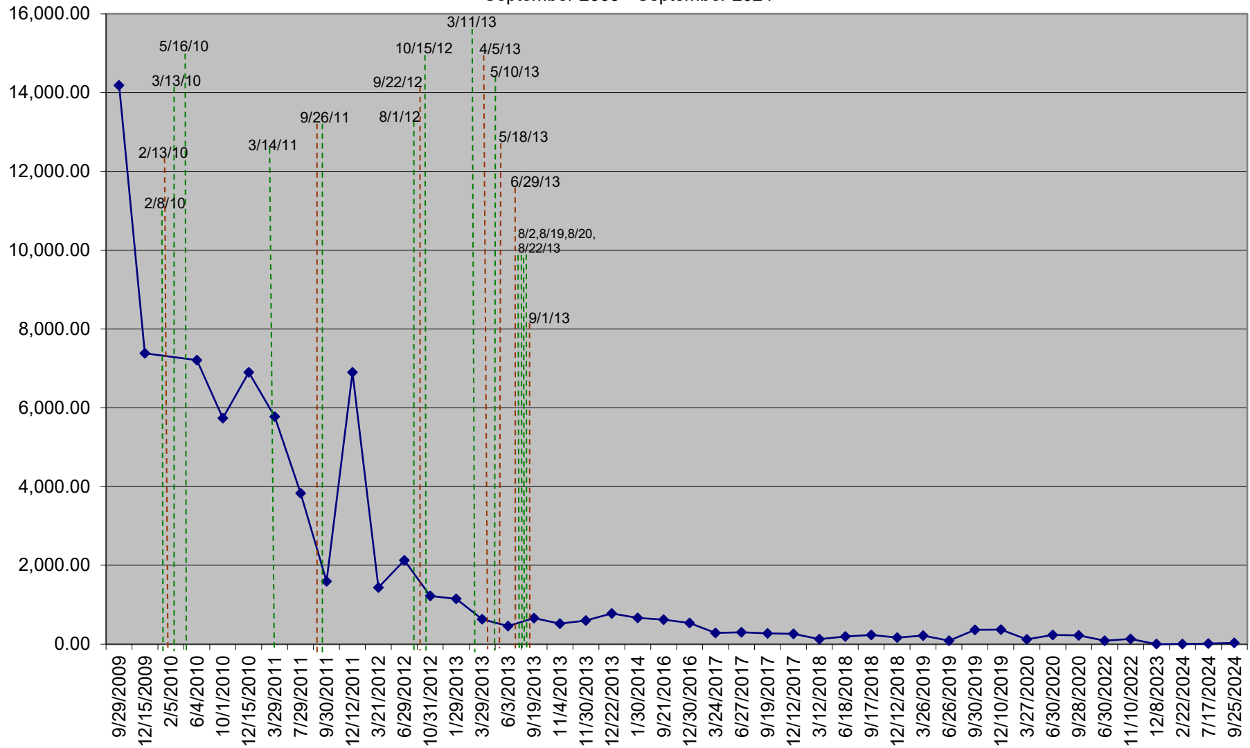
Graph 3 IRMW-11 Total Petroleum VOCs 3035 White Plains Road, Bronx, NY September 2009 - September 2024
