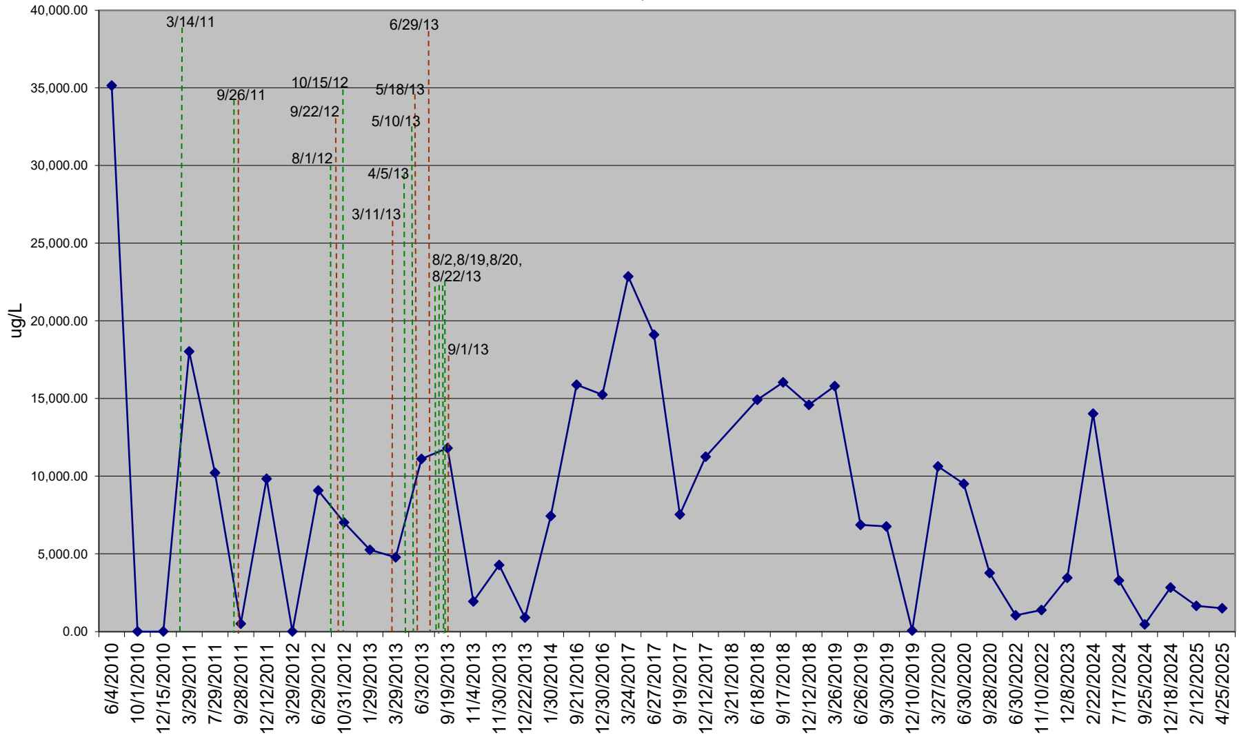
Graph 4 IRMW-14 Total Petroleum VOCs 3035 White Plains Road, Bronx, NY June 2010 - April 2025
