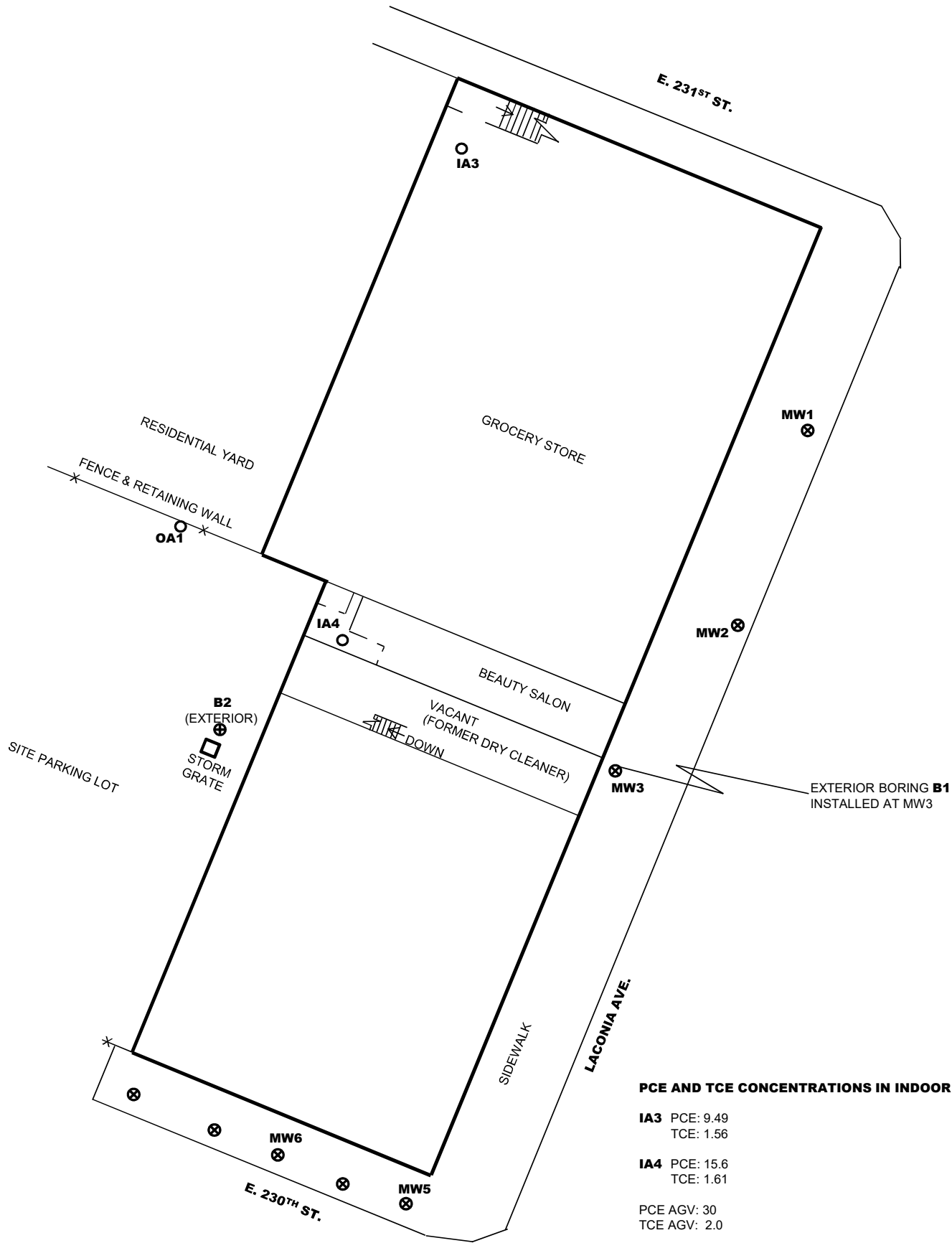
FIGURE 4, AIR SAMPLE LOCATIONS (INTERIOR DETAILS SHOW 1 ST FLR. ONLY) 4125 TO 4149 LACONIA AVE. BRONX, NY
