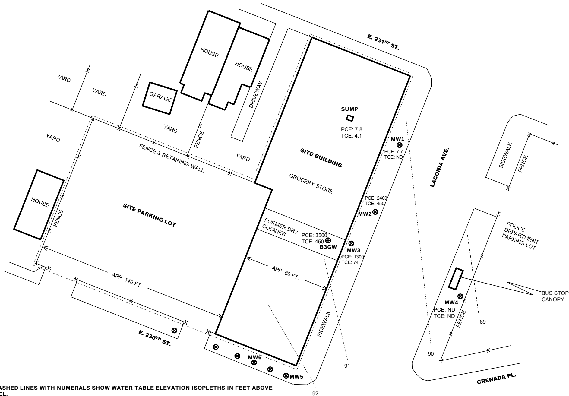
FIGURE 2, WELL LOCATION PLAN: 4125 TO 4149 LACONIA AVE.
