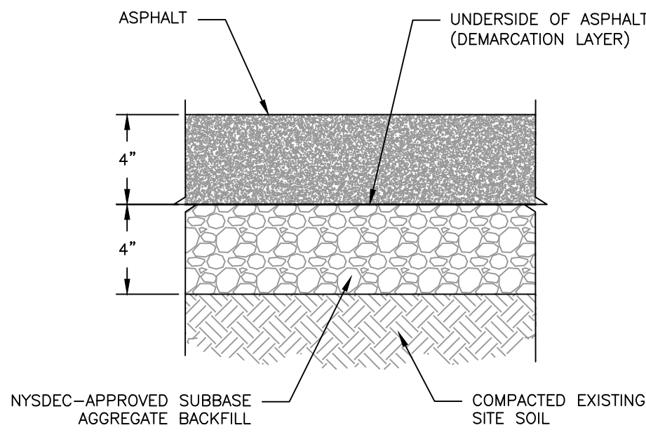
SITE COVER SYSTEM: PAVED AREA-PARKING LOT SCALE: NOT TO SCALE
