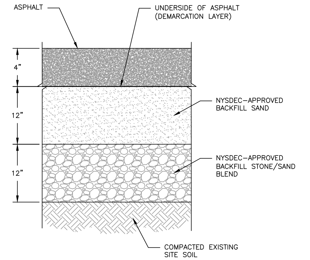
SITE COVER SYSTEM: PAVED AREA-PARKING LOT SCALE: NOT TO SCALE
