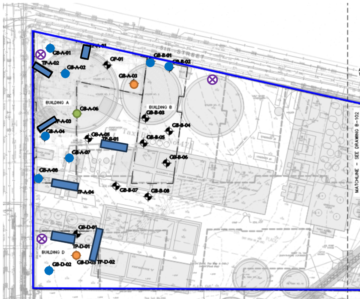
Figure 1: Site Plan – West
