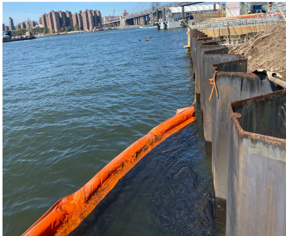
Photo 4: View of turbidity curtain maintenance and repair.
