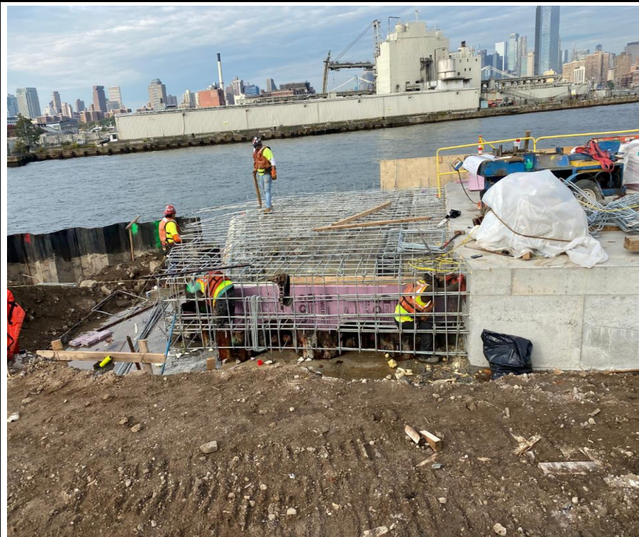
Photo 4: View of the rebar installation along the waterfront facing north.
