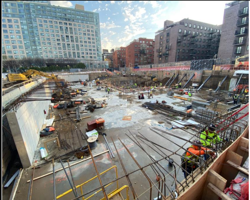
Photo 1: View of Site conditions and activities facing northeast.
