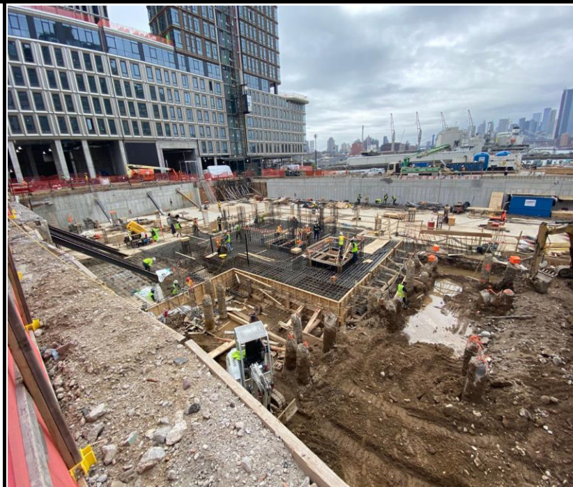
Photo 4: View of Site conditions facing southwest.
