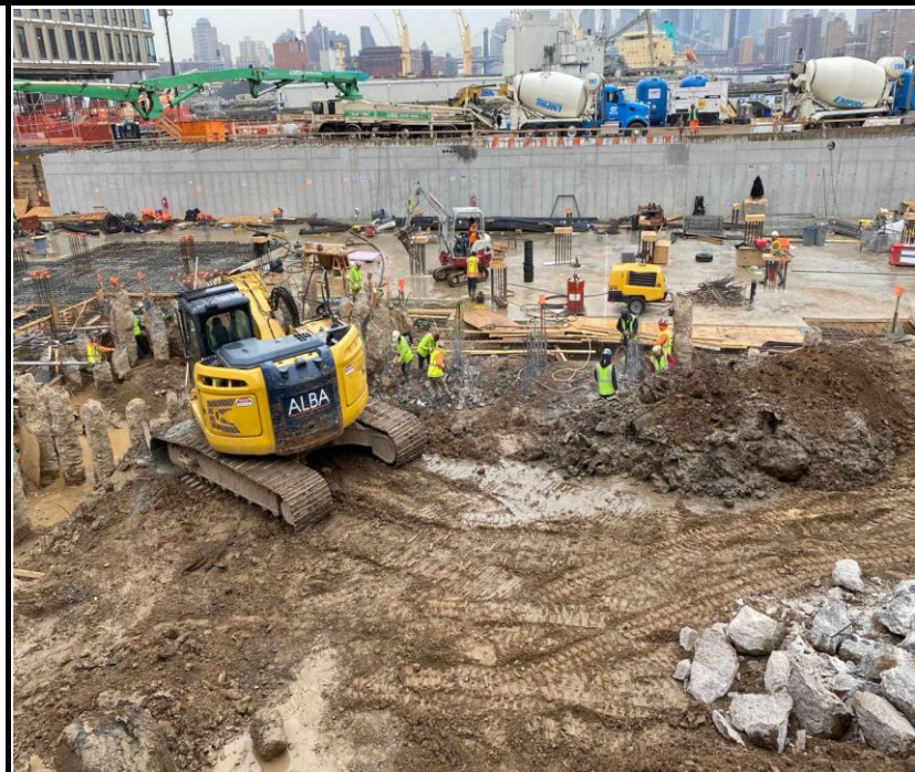
Photo 2: View of Site conditions and soil excavation facing west.
