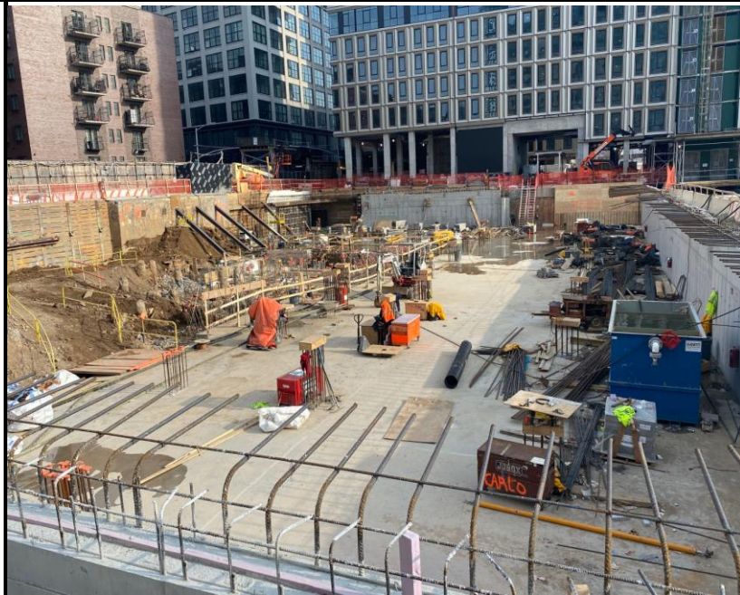
Photo 3: View of site conditions and activities facing south.
