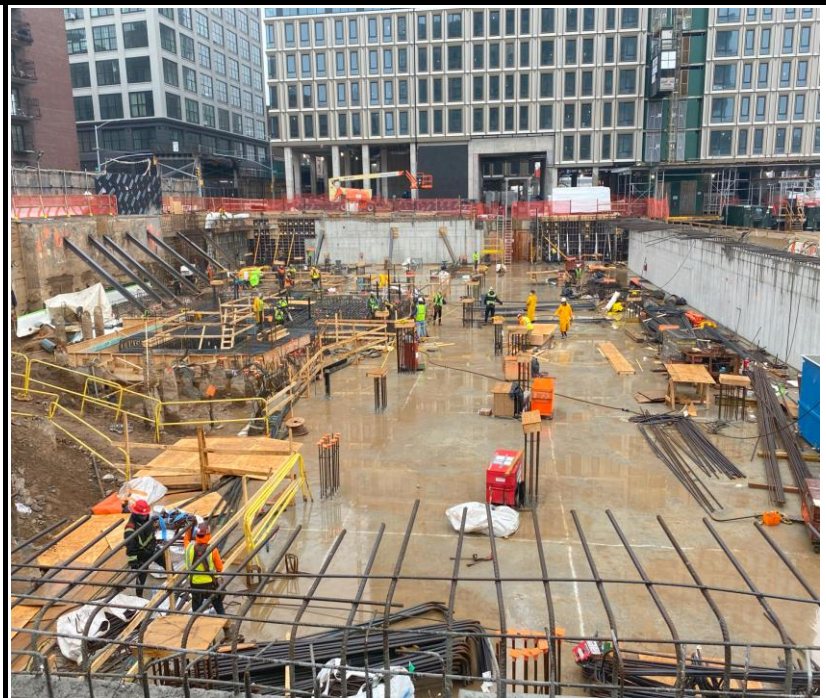
Photo 2: View of Site conditions and foundation development facing south.
