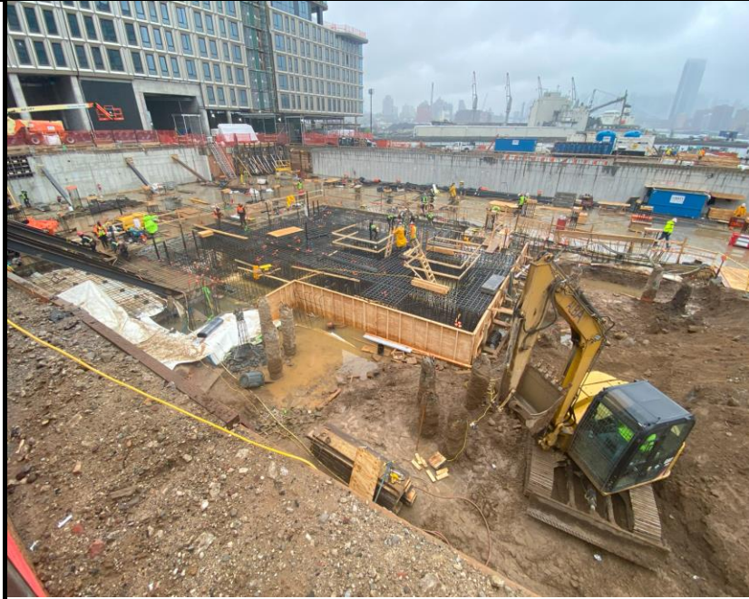
Photo 1: View of Site conditions and activities facing west.
