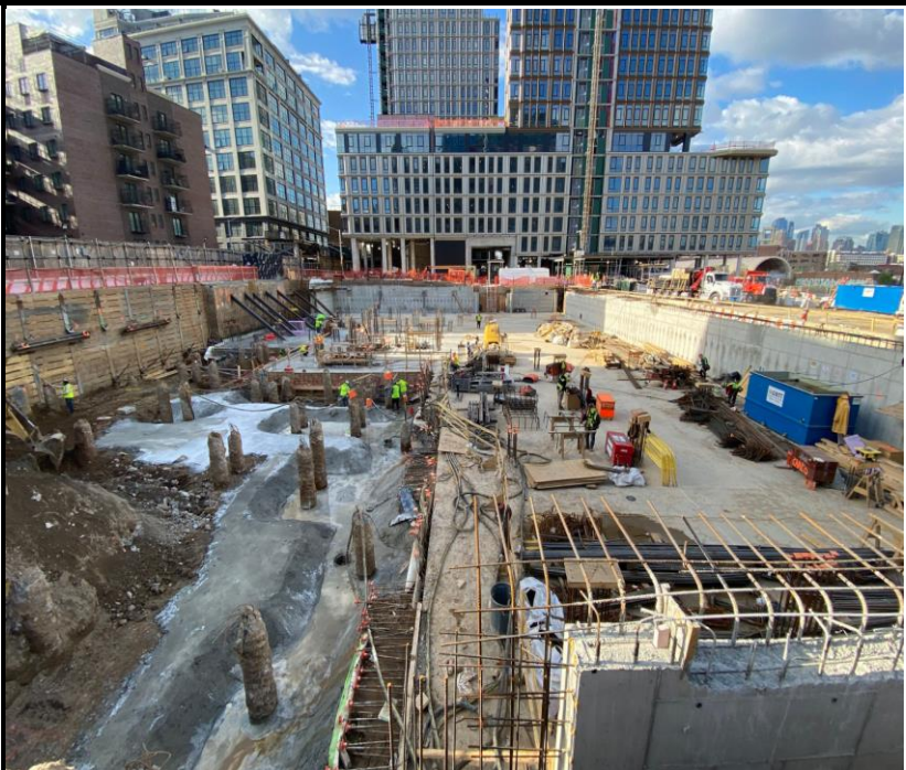
Photo 4: View of Site conditions facing south.
