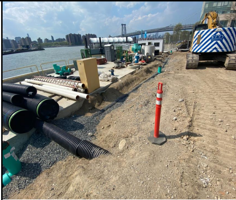
Photo 4: View of continued work on stormwater piping, facing northwest.
