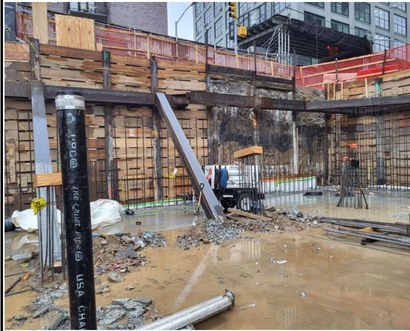
Photo 3: View of rebar installation facing east.
