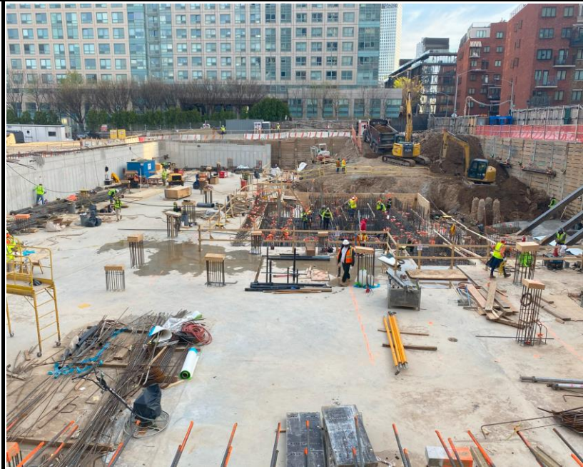
Photo 1: View of Site conditions and activities facing north.
