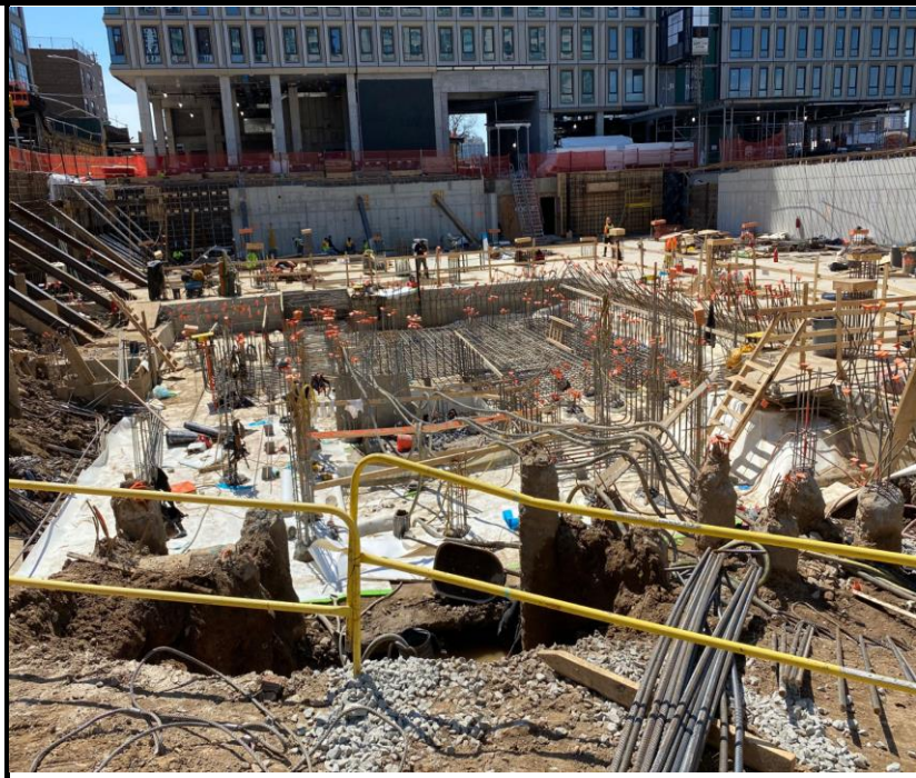
Photo 4: View of waterproofing and rebar installation.
