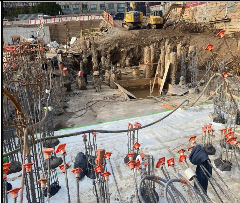
Photo 4: View of Site conditions and soil excavation facing north.
