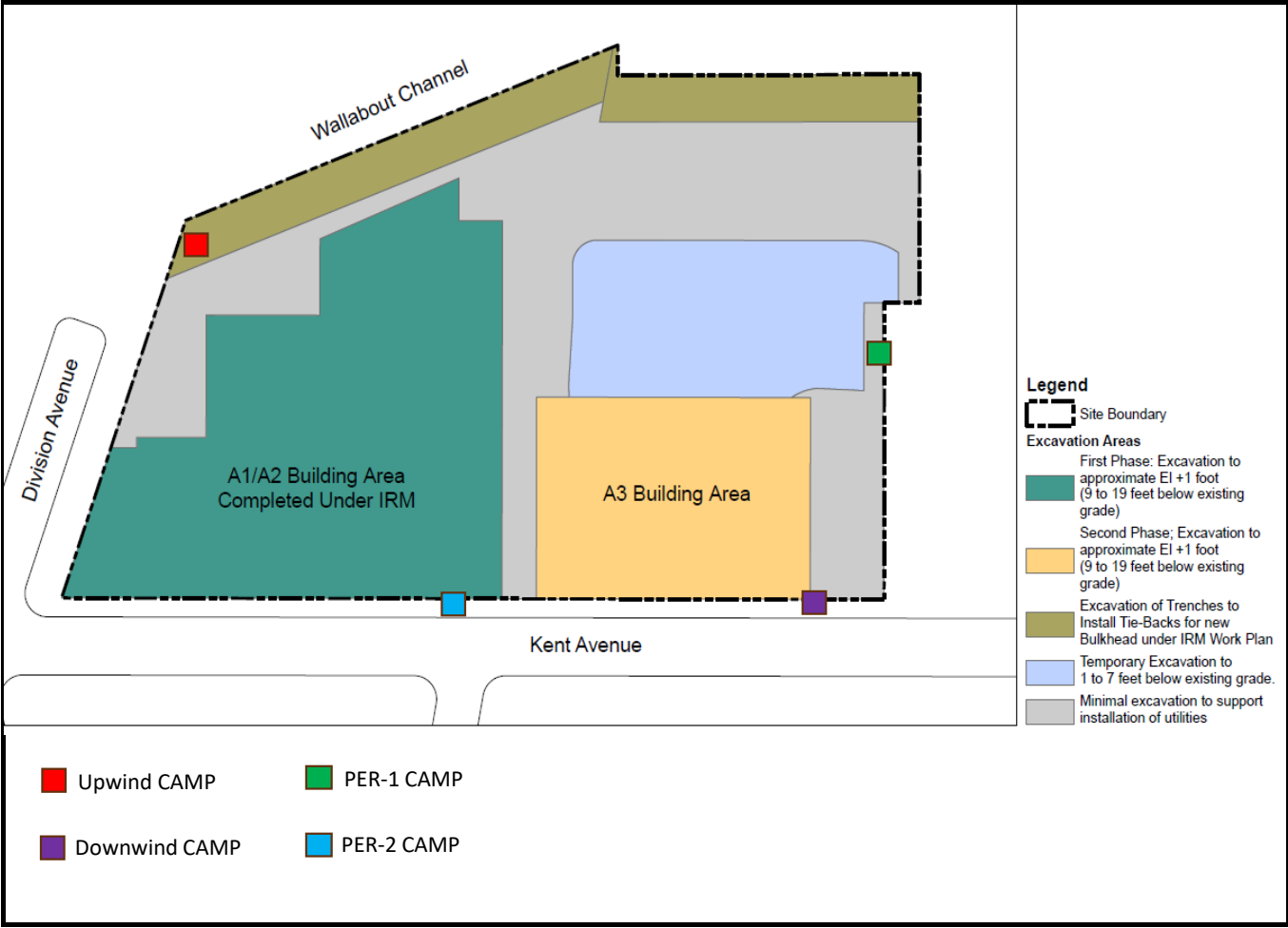
Site Layout Map and Excavation Figures
