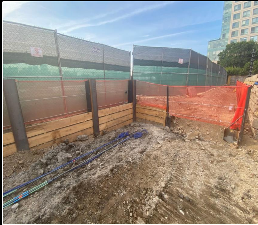
Photo 4: View of lagging installation.
