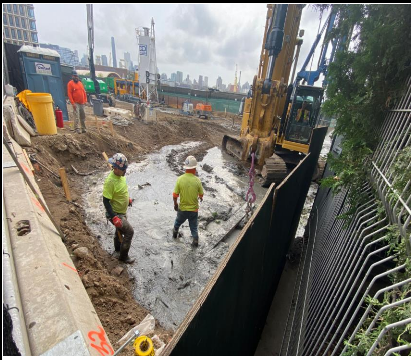
Photo 4: View of Site conditions during pile installation and grouting facing southwest.
