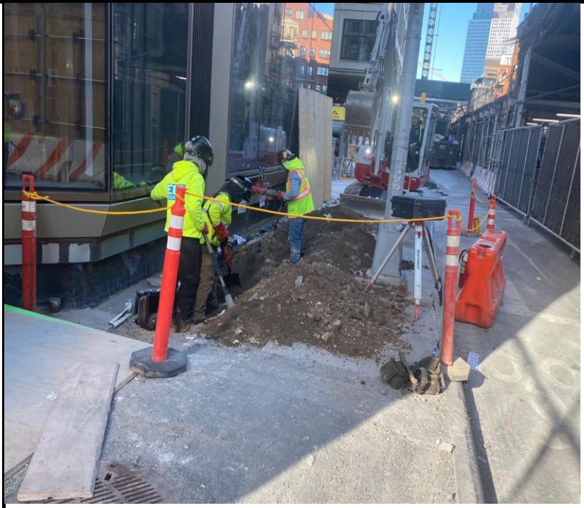
Photo 2: View of ECD completing utility trenching.
