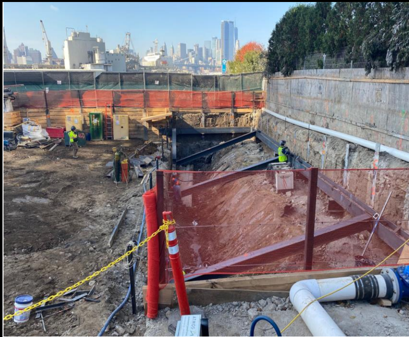
Photo 1: View of continued SOE installation for the northern remedial excavation.
